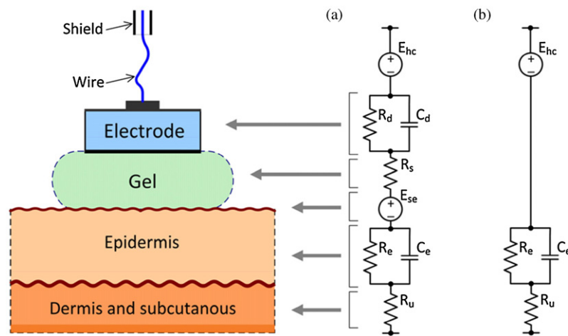
Figure 1. Electrical model for electrode-to-skin interface: (a) gel electrode and (b) dry electrode.
