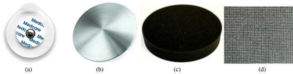
Figure 2. Electrode categories: (a) conventional Ag/AgCl, (b) stainless-steel disc, (c) conductive foam and (d) conductive fabric.
