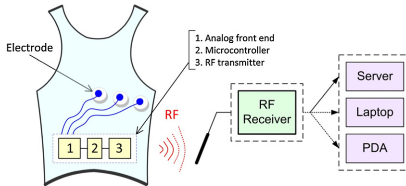
Figure 3. Practical design of a dry-electrode system.
