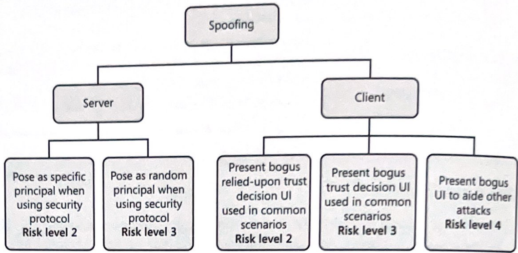
Figure 9-6 Spoofing threats risk ranking.
