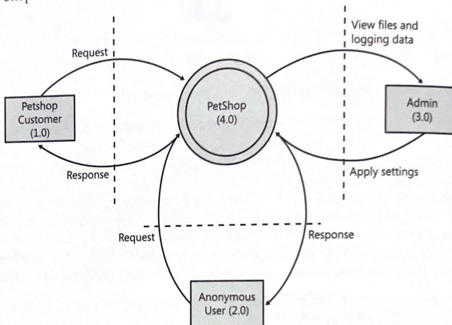
Figure 9-3 Context diagram for Pet Shop 4.0.
