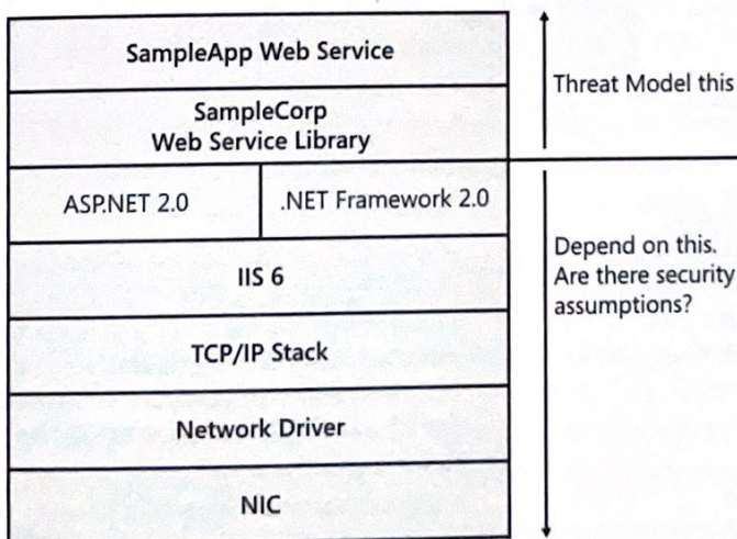
Figure 9-2 Drawing the line between what you threat-model and what you depend on.
