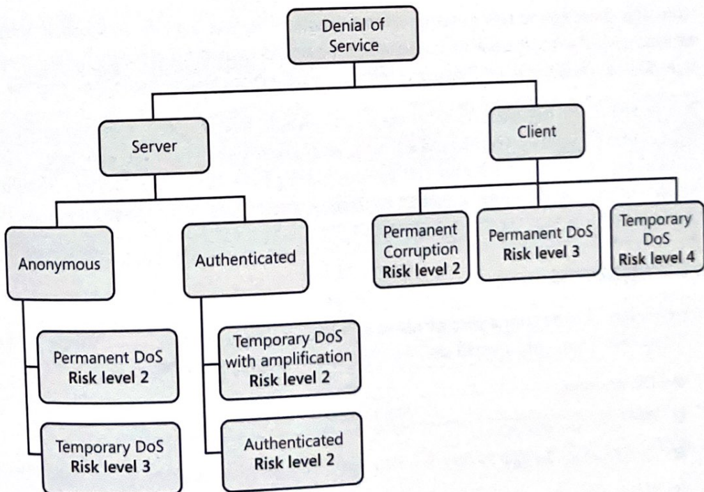
Figure 9-9 DoS threats risk ranking.
