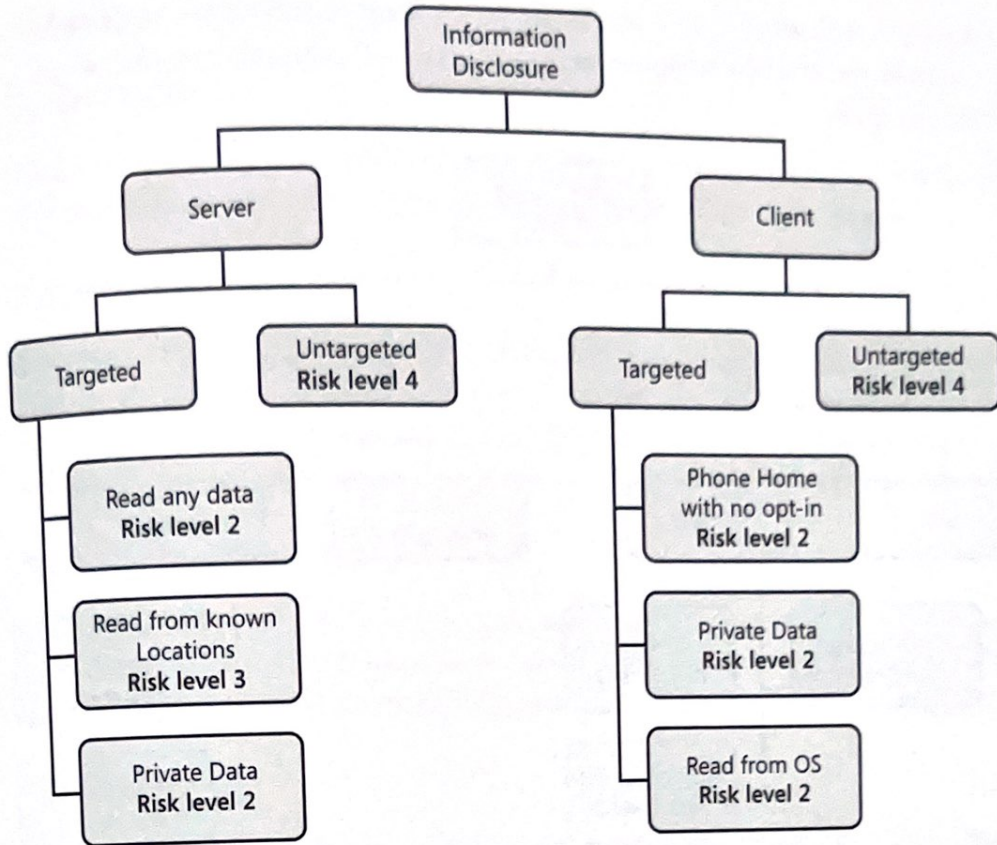
Figure 9-8 Information disclosure threats risk ranking.
