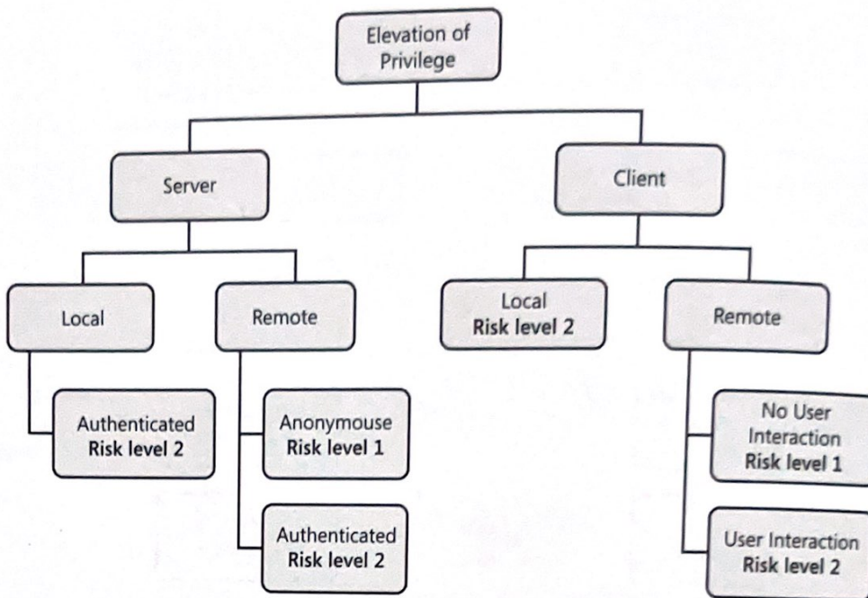
Figure 9-10 EoP threats risk ranking.
