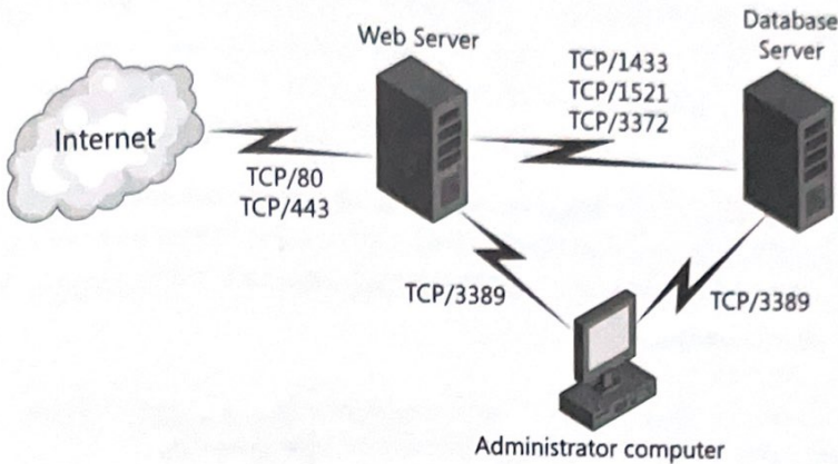
Figure 9-1 Port usage in the Pet Shop 4.0 application.
