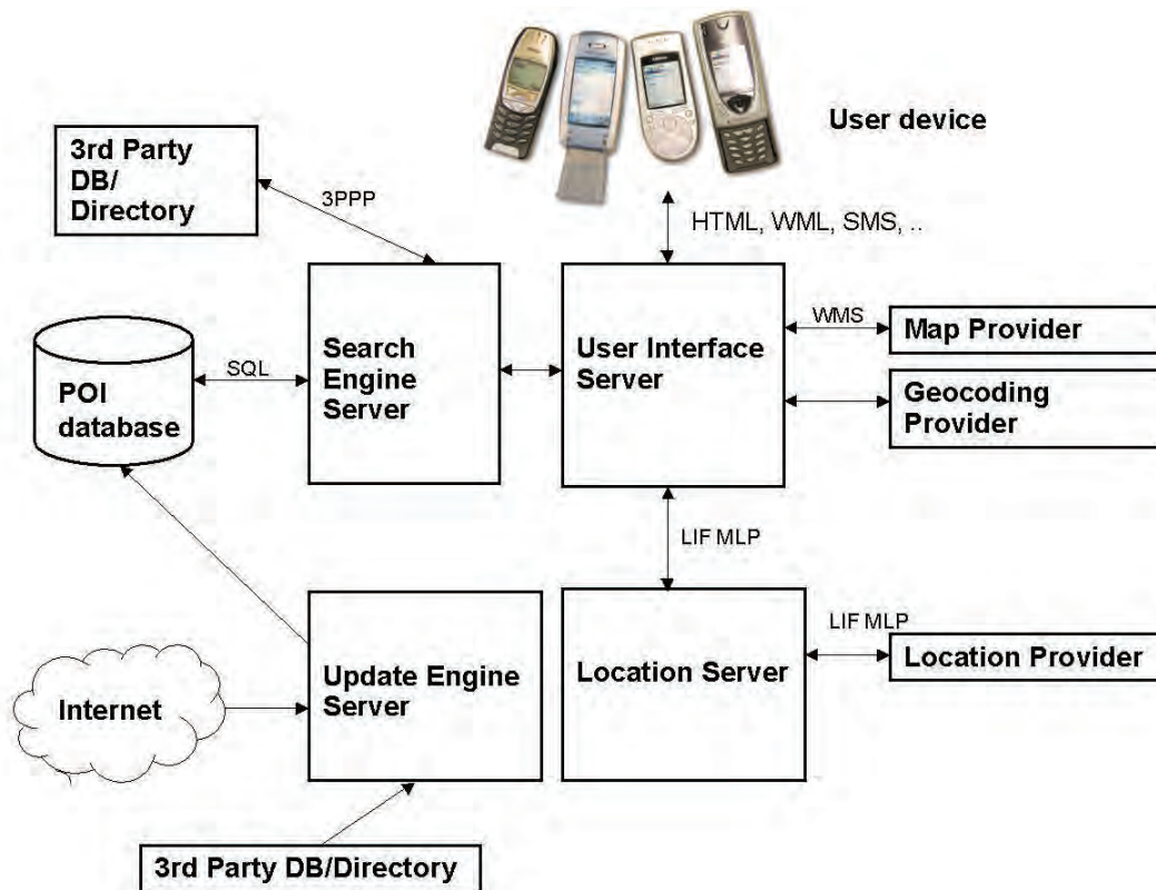
Figure 26. Architecture of NAVISearch location-aware integrated directory service.
