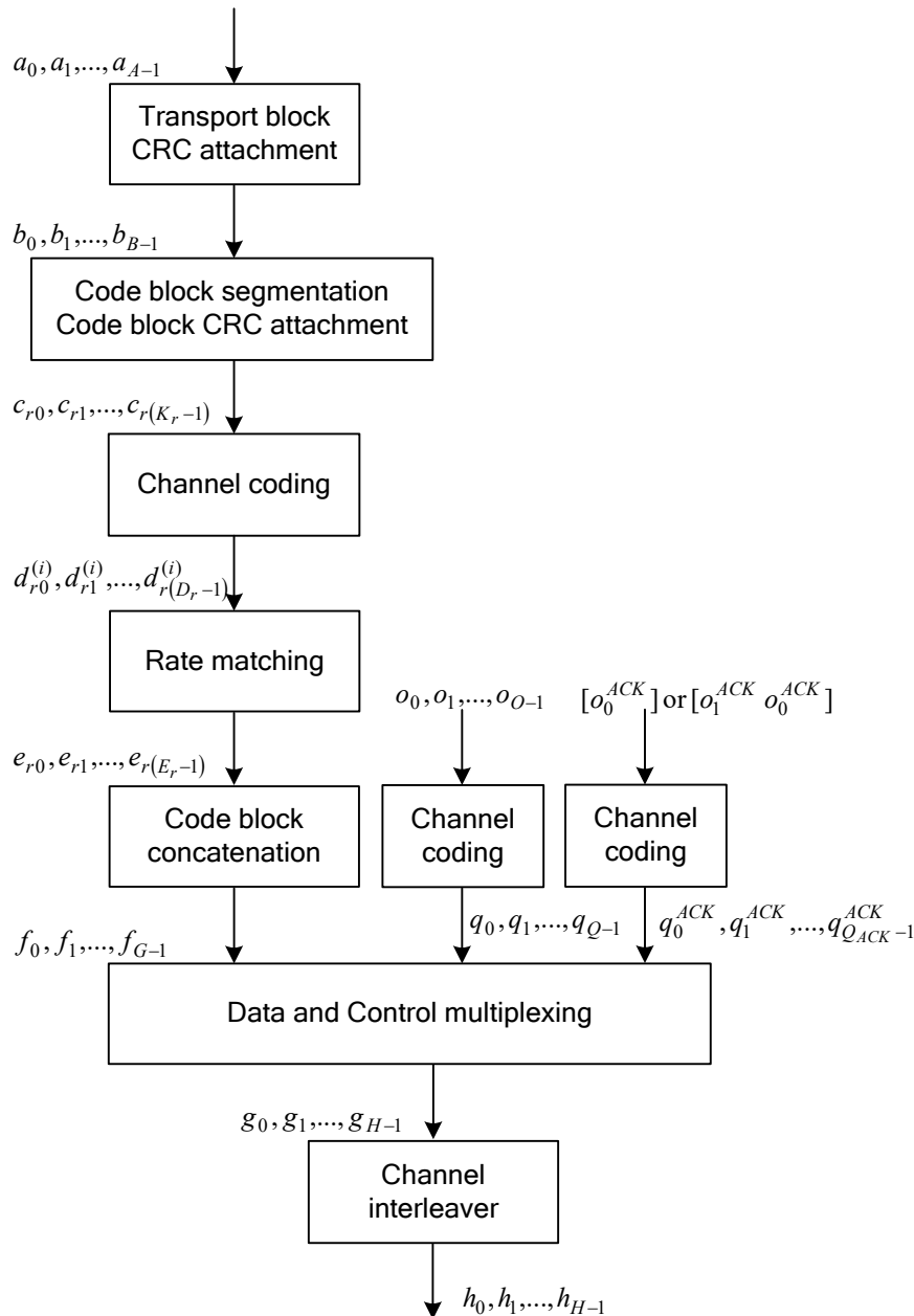
Figure 5.2.2-1: Transport channel processing for UL-SCH
