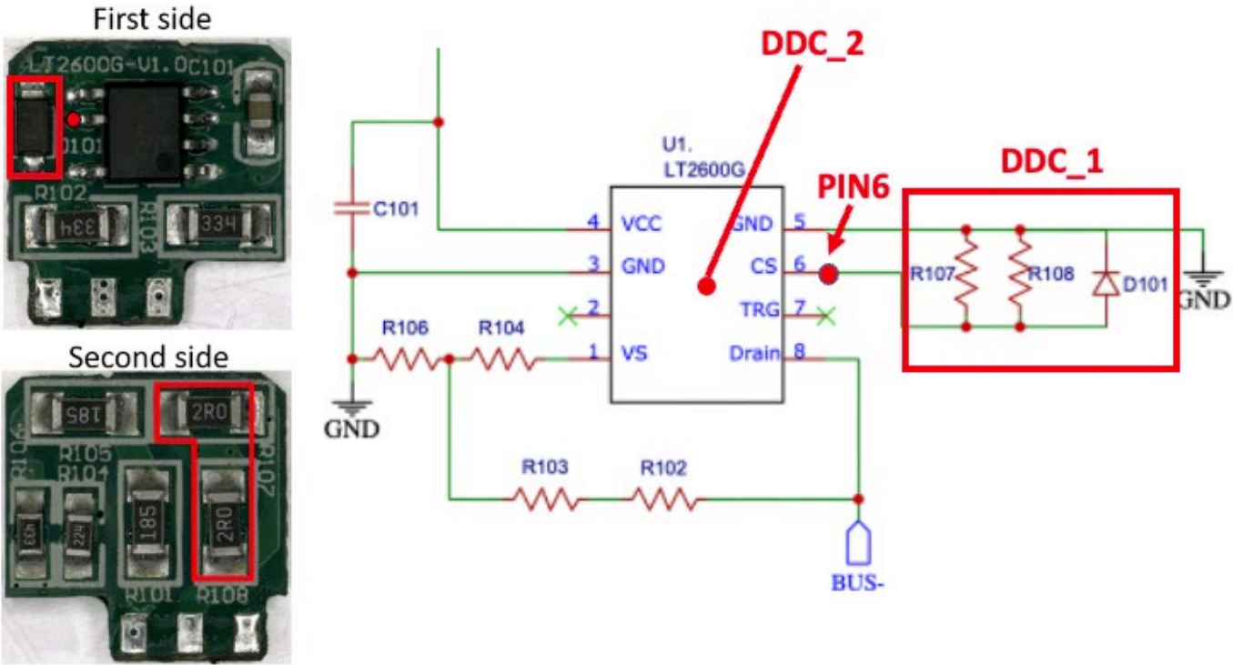
Figure 26. The detection determining circuit is comprised of DDC_1 on the GE daughter board, outlined in red on the PCB (bottom left) and on the equivalent circuit schematic (right), and DDC_2 comprised of circuitry within the LT2600G package, labeled on the schematic as U1_.
