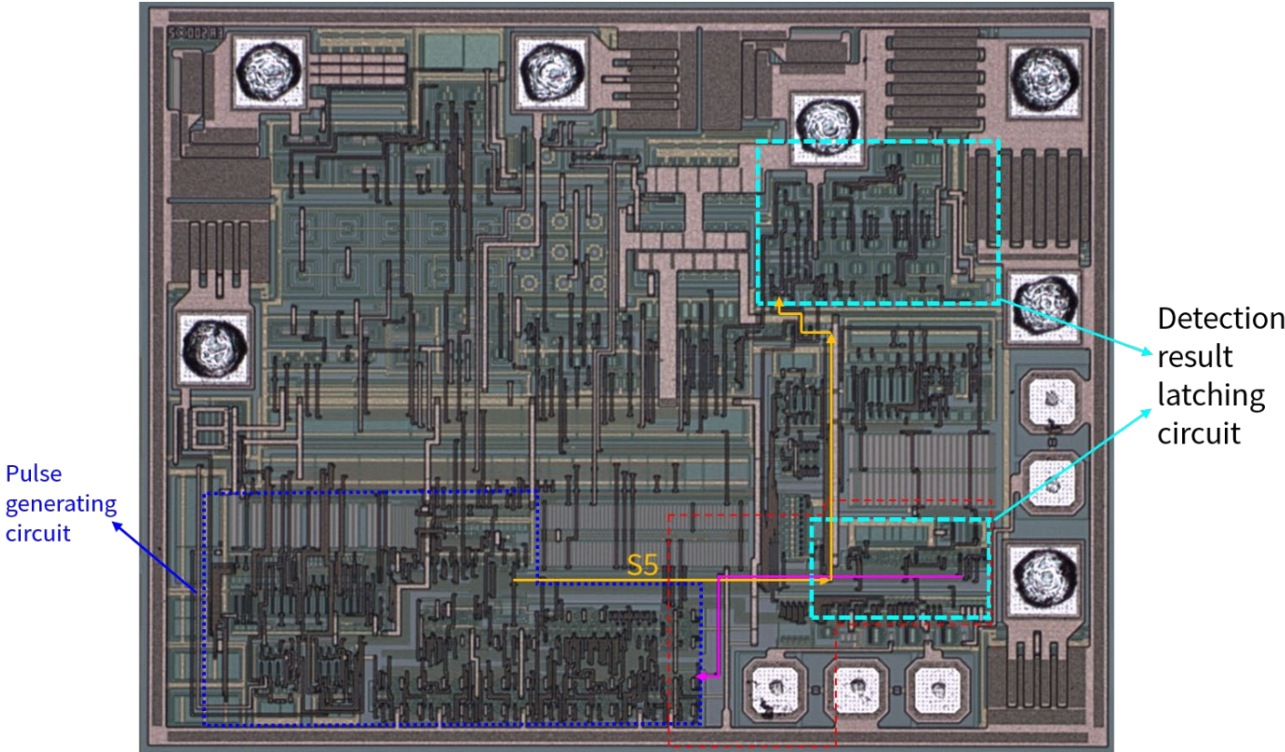
Figure 33. The signal OVP_DEL_EN is generated within the detection result latching circuit and is coupled between the pulse generating circuit and an output of the detection result latching circuit. The trace this signal follows is highlighted by the magenta arrow. The region outlined by the dashed red line is shown in greater detail in Figure 34.
