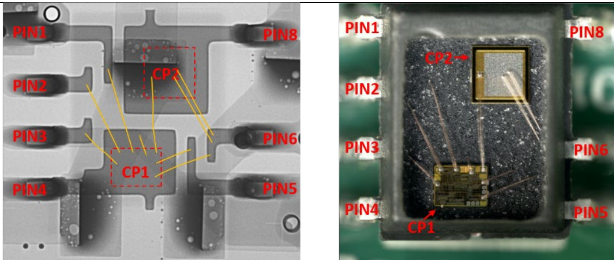
Figure 6. (Left) X-ray image of the LT2600G IC on the LT2600G-V1.0 daughter board showing two chips, labeled as CP1 and CP2. Wire bonds between chips and the package pin outs are highlighted in yellow for visibility. (Right) Optical micrograph of decapped LT2600G on the daughter board.
