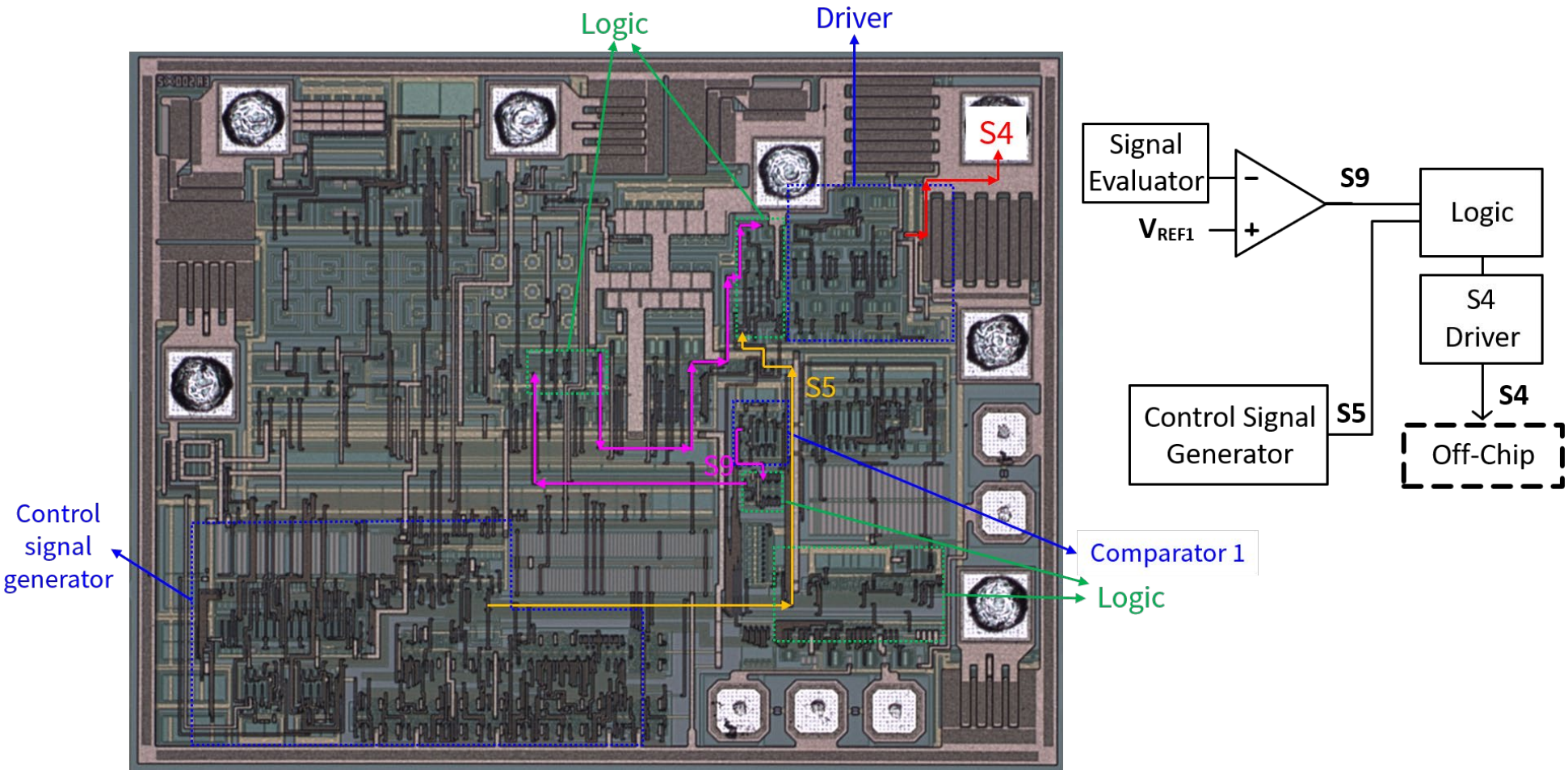
Figure 11. Signal traces from comparator 1 and the pulse generator provide S9 and S5, respectively, as input signals for the digital logic circuitry, which outputs a signal to the S4 driver.
