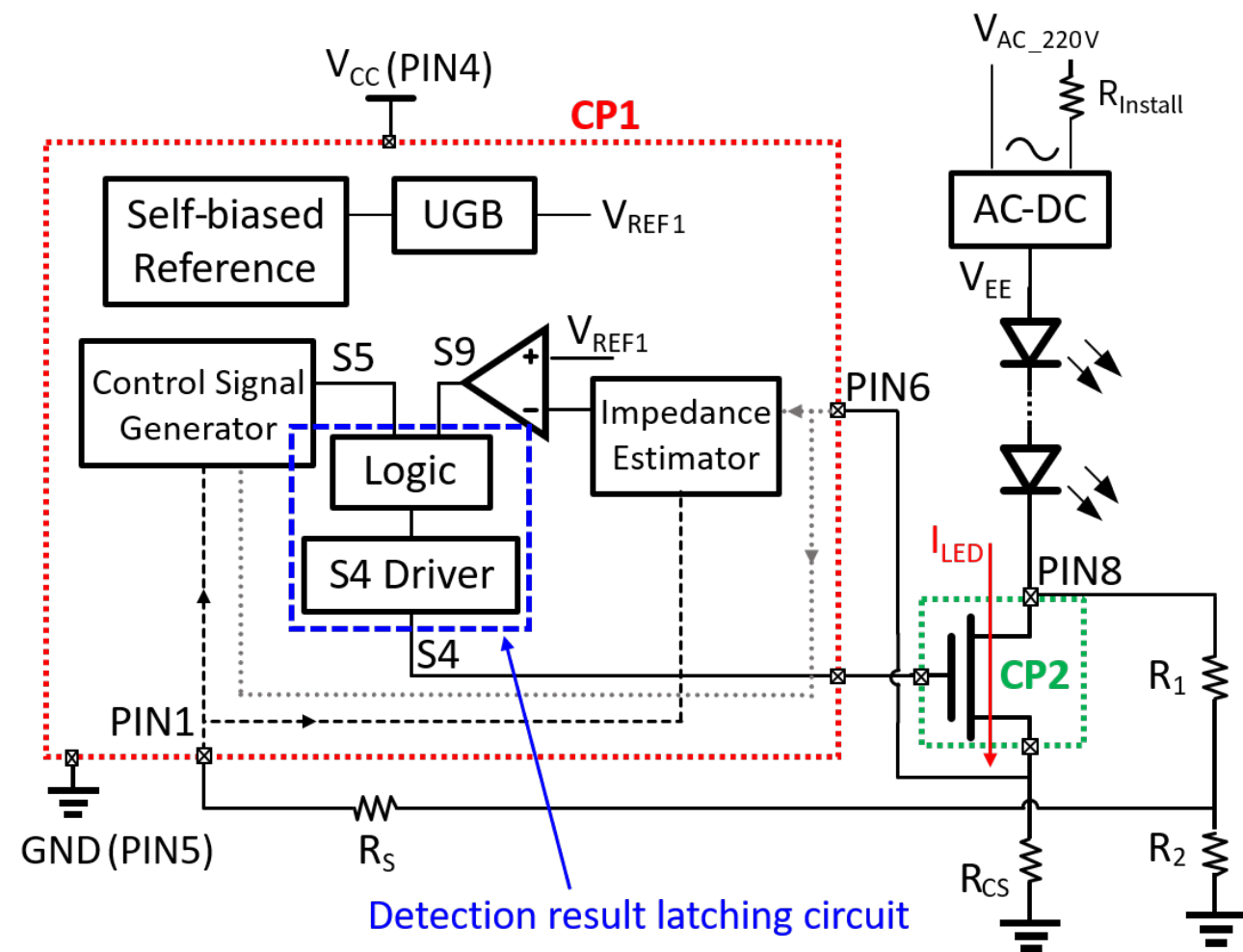
Figure 31. The digital logic and S4 driver, both outlined in dashed blue, together form the detection result latching circuit.
