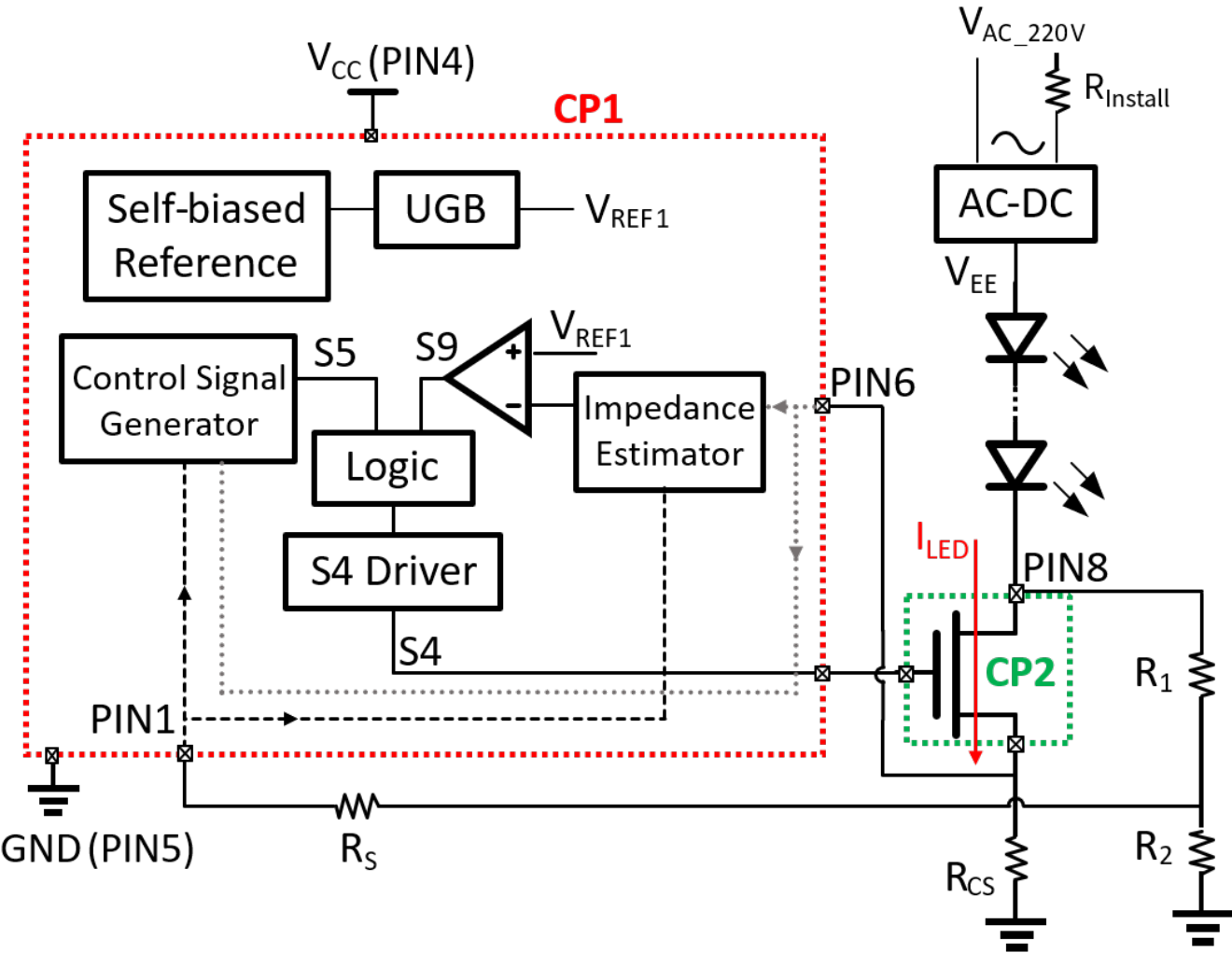
Figure 13. Simplified schematic showing system overview of the installation detection circuit. Comparator 1 follows the impedance estimator, which includes the signal evaluator shown in Figure 10. The output of comparator 1 and the output of the control signal generator are both used as inputs for the subsequent logic circuitry.
