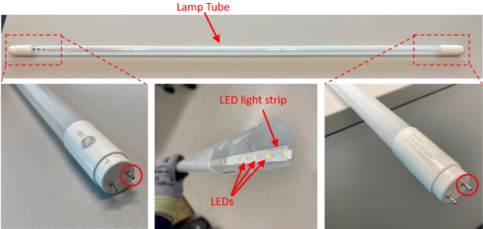
Figure 2. Photos of the GE LED tube lamp showing central portion comprised of lamp tube (top), two end caps with electrical contacts for receiving an external driving signal (bottom right and bottom left), and central portion of the lamp wherein the tube has been broken to expose the LEDs disposed on a strip contained within the tube.
