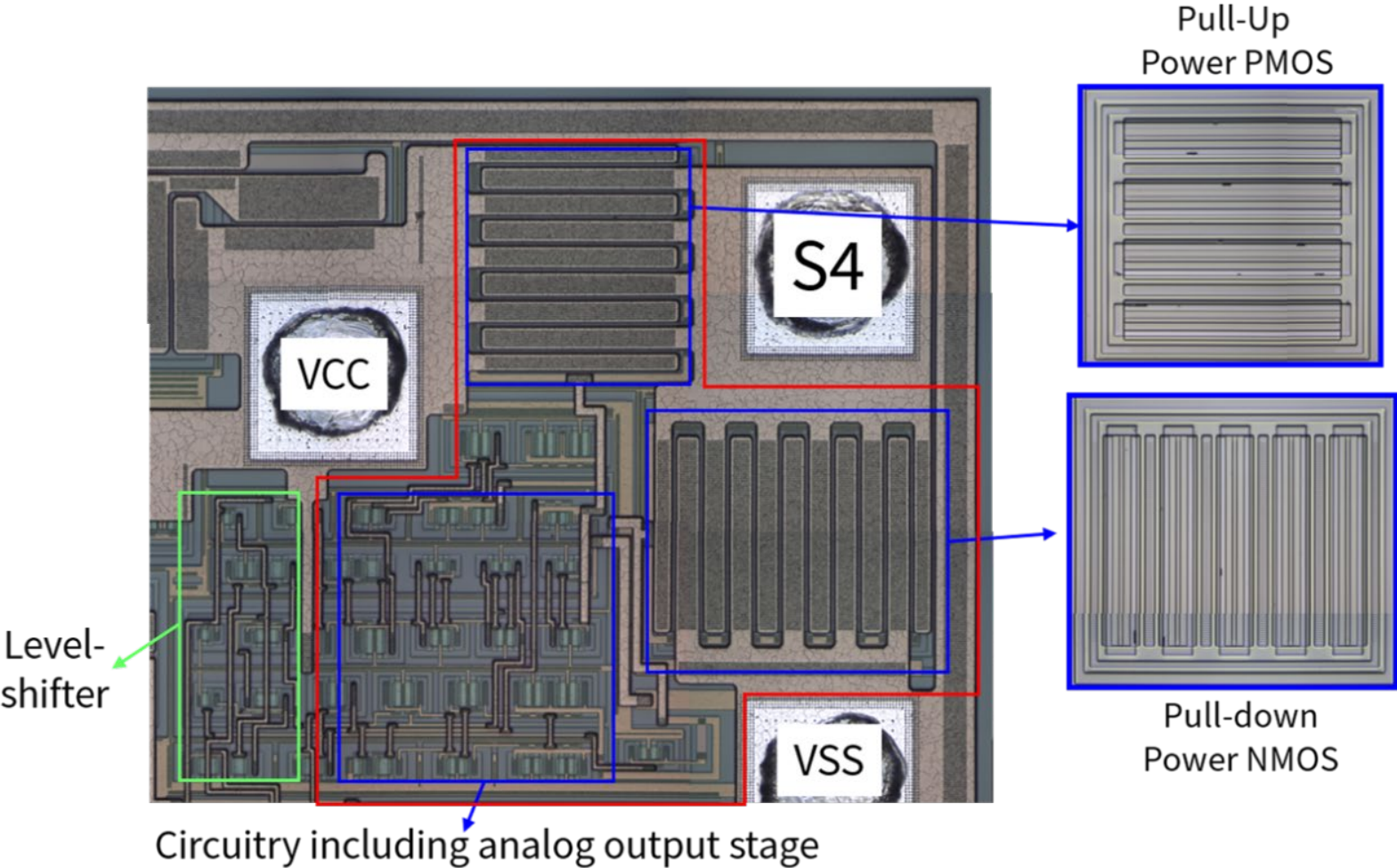
Figure 12. The S4 driver consists of sub-component including a digital input stage, deadtime generator, analog output stage, and large pull-up and pull-down transistors near the S4 pad.
