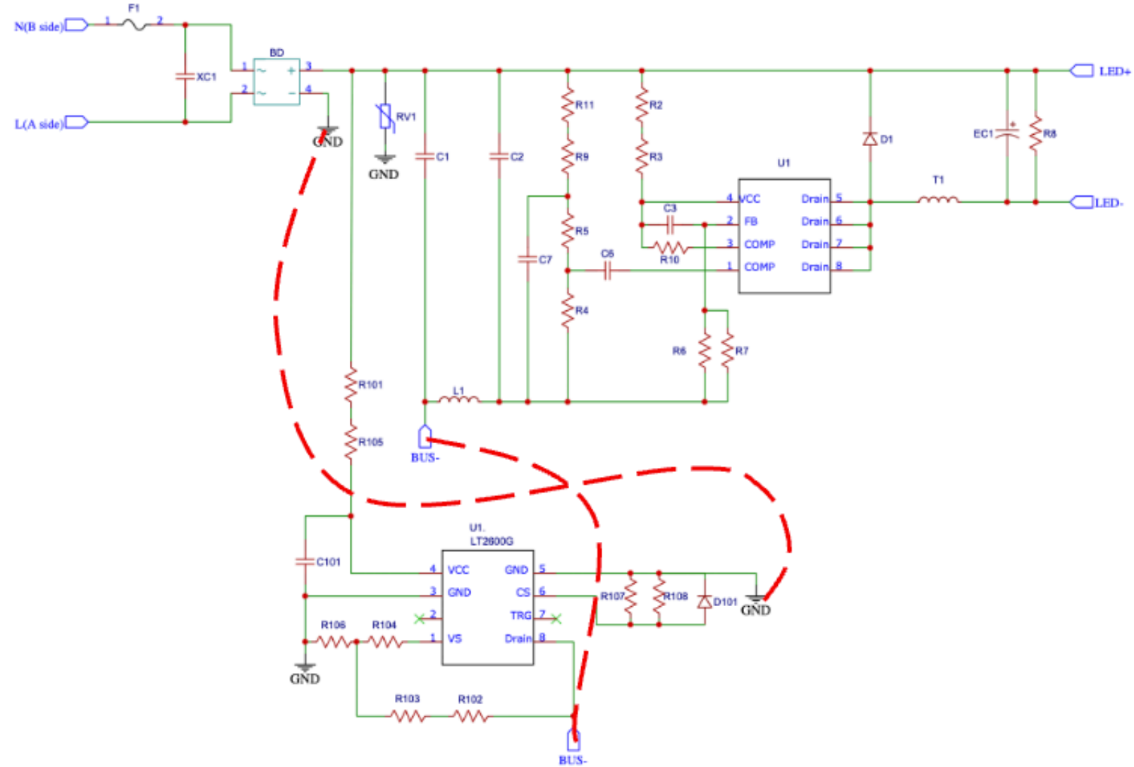
Figure 36. The connection correlation of LT2600G shows it is coupled between the rectifying circuit and the filtering circuit through GND terminal (PIN5) and BUS- terminal (PIN8).
