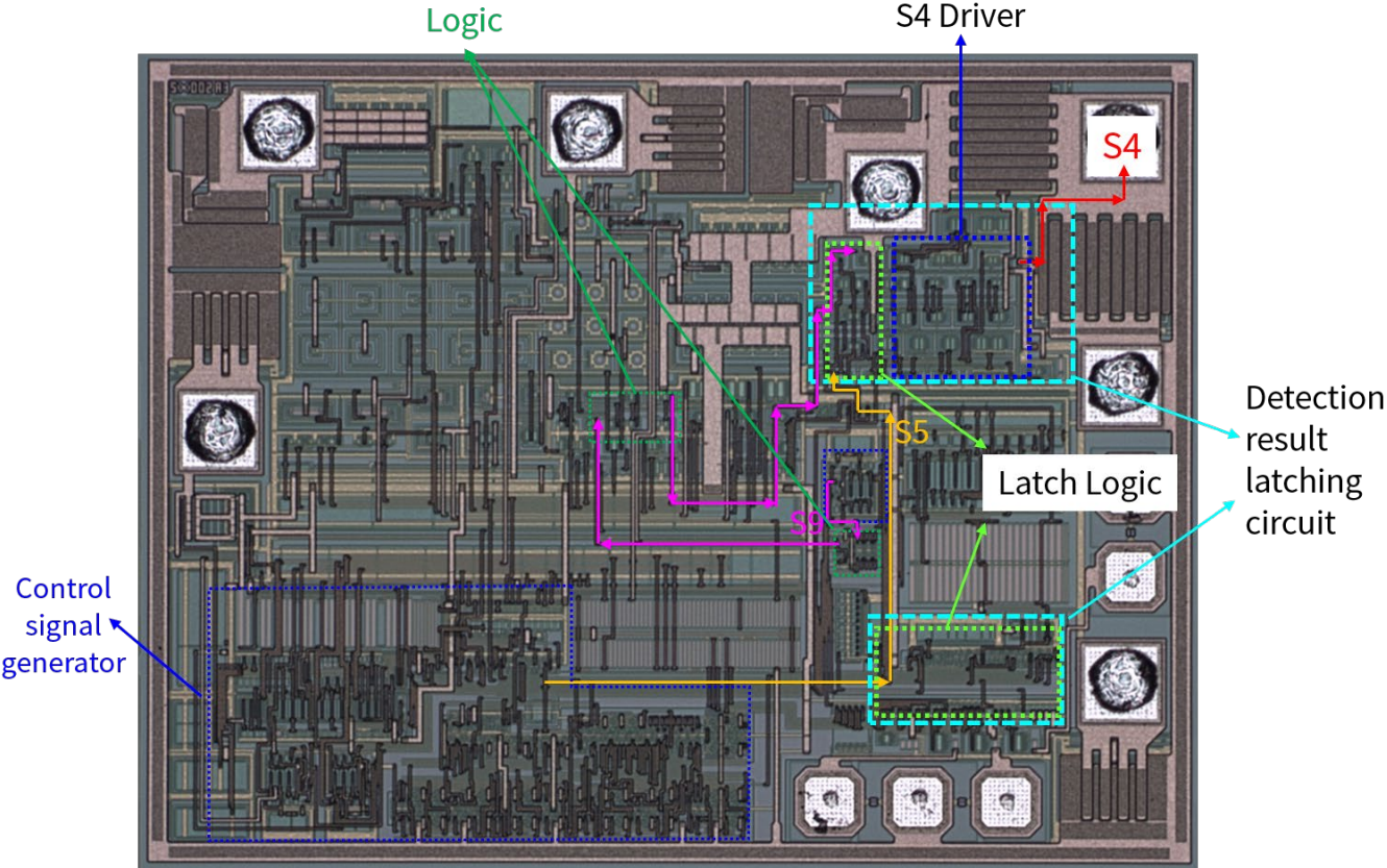
Figure 30. Logic blocks (e.g., digital logic) and the S4 driver together form the detection result latching circuit, outlined by the upper and lower dashed cyan boxes.
