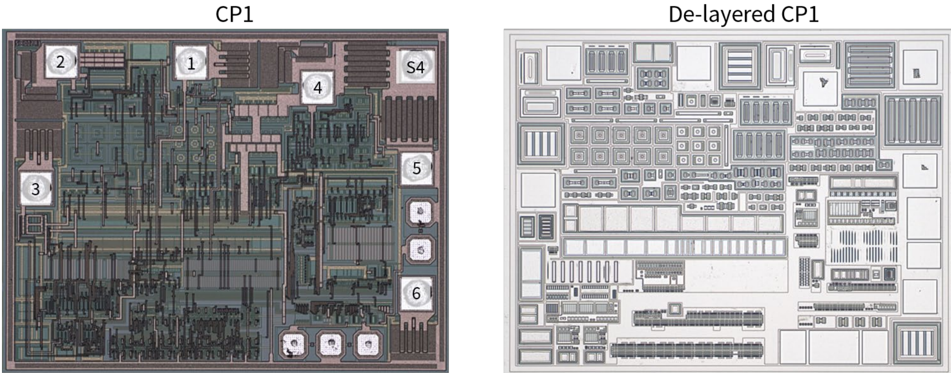
Figure 7. (Left) Optical micrograph of CP1 with wire bonds removed. (Right) Optical micrograph of CP1 after de-layering process to remove metallic traces and insulating layers.
