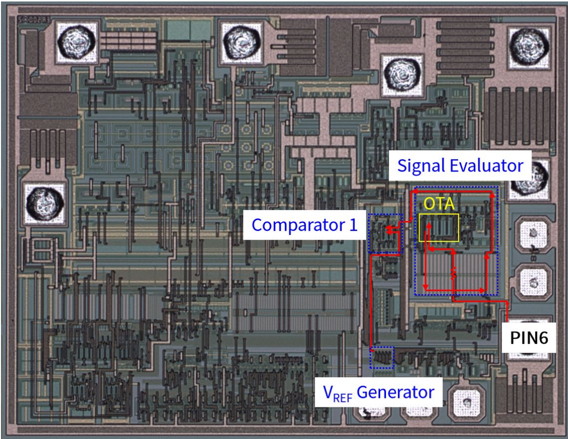
Figure 10. Signal traces from the output of the signal evaluator circuit and a voltage reference, V_{REF1} , provide a pair of input signals to comparator 1, which outputs signal S9.
