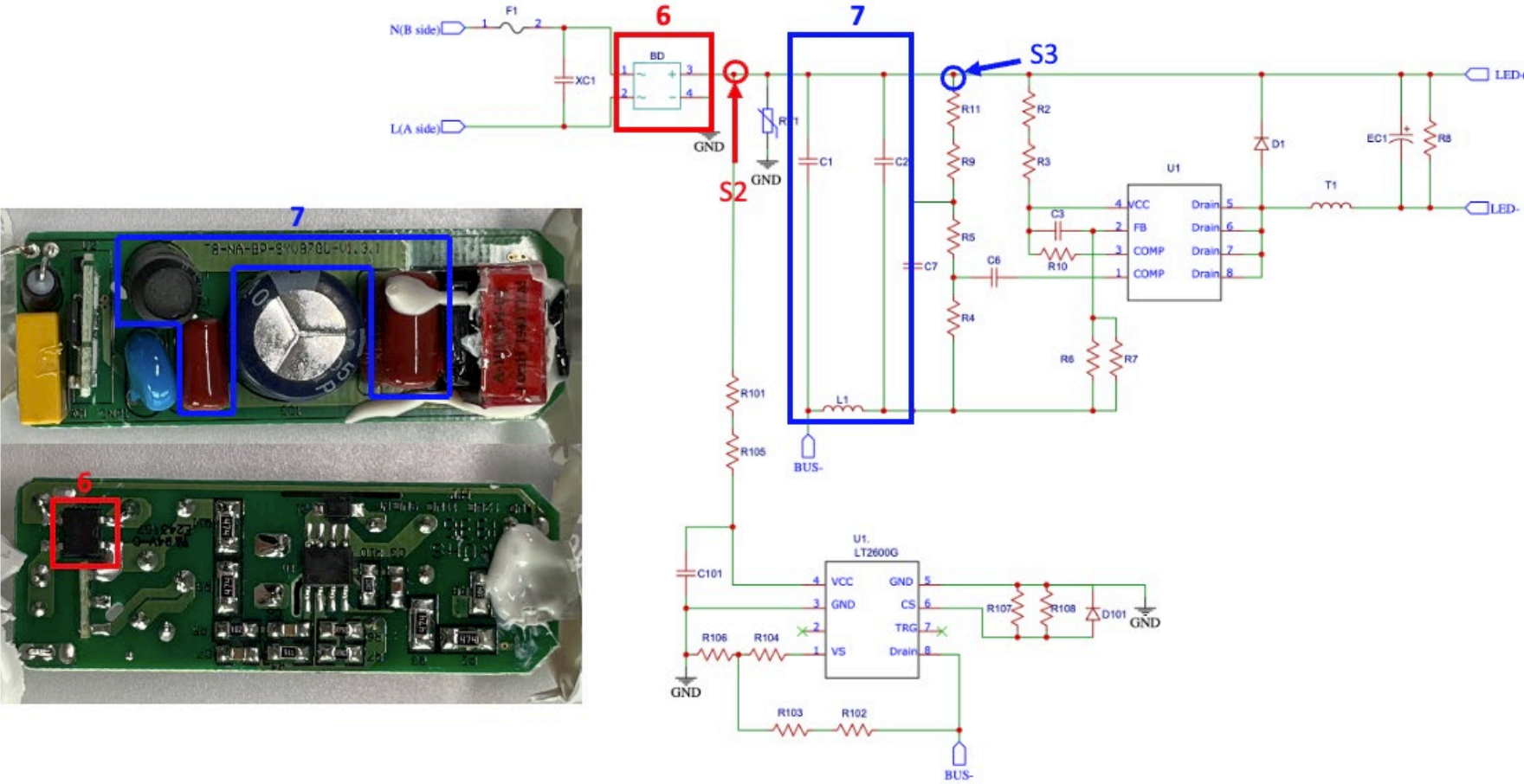
Figure 35. The GE tube lamp comprises a rectifying circuit, outlined in red, and a filtering circuit, outlined in blue on the PCB (left) and on the equivalent circuit diagram (right)
