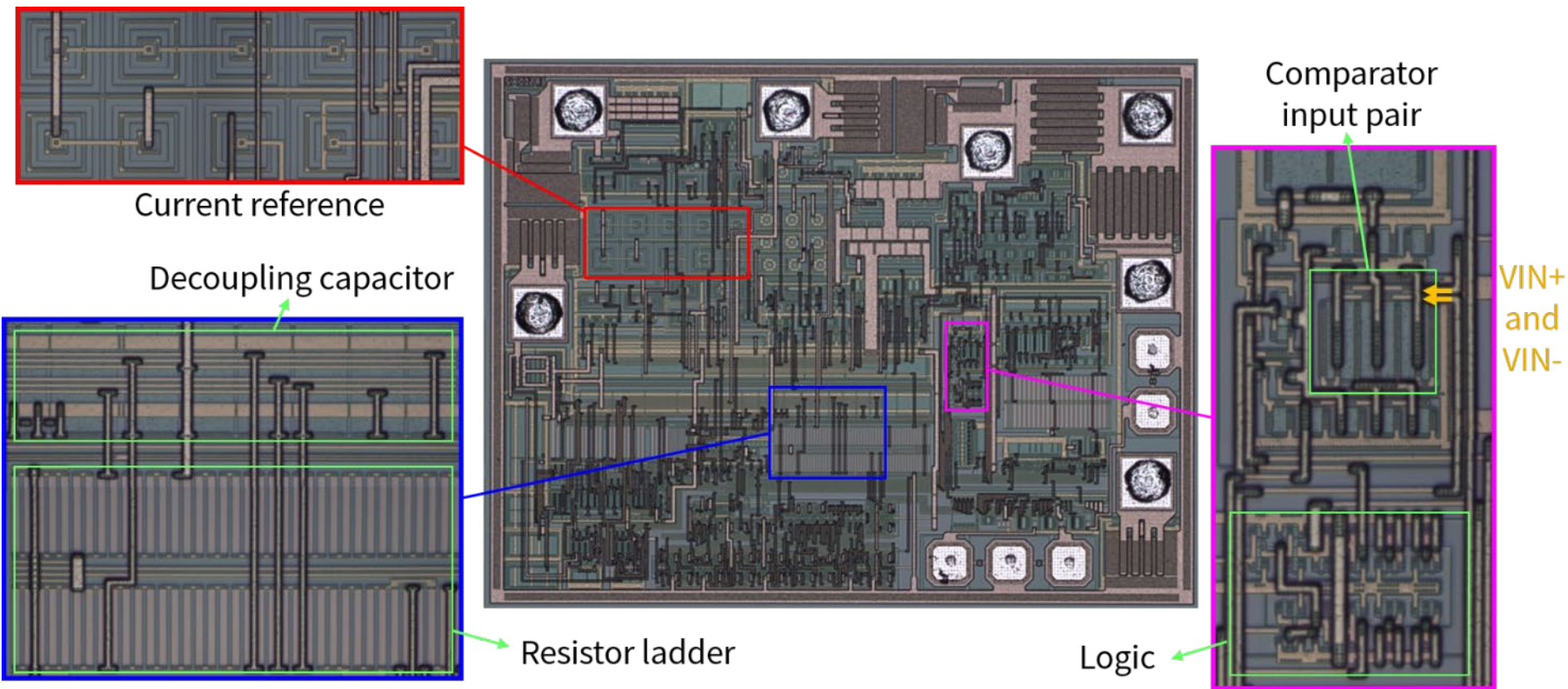
Figure 8. Integrated circuit components are identified on the CP1 die.
