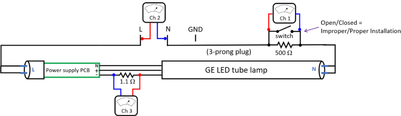
Figure 24. Schematic of measurement setup. Channel 3 measures voltage across a 1.1 Ω shunt resistor, which is proportional to loop current. Thus, loop current can be measured when the lamp is not properly installed (i.e., when the mechanical switch is open and the current must flow through the 500 Ω resistor), and when the lamp is properly installed (i.e., when the mechanical switch is closed and the current may flow through the short circuit around the 500 Ω resistor).
