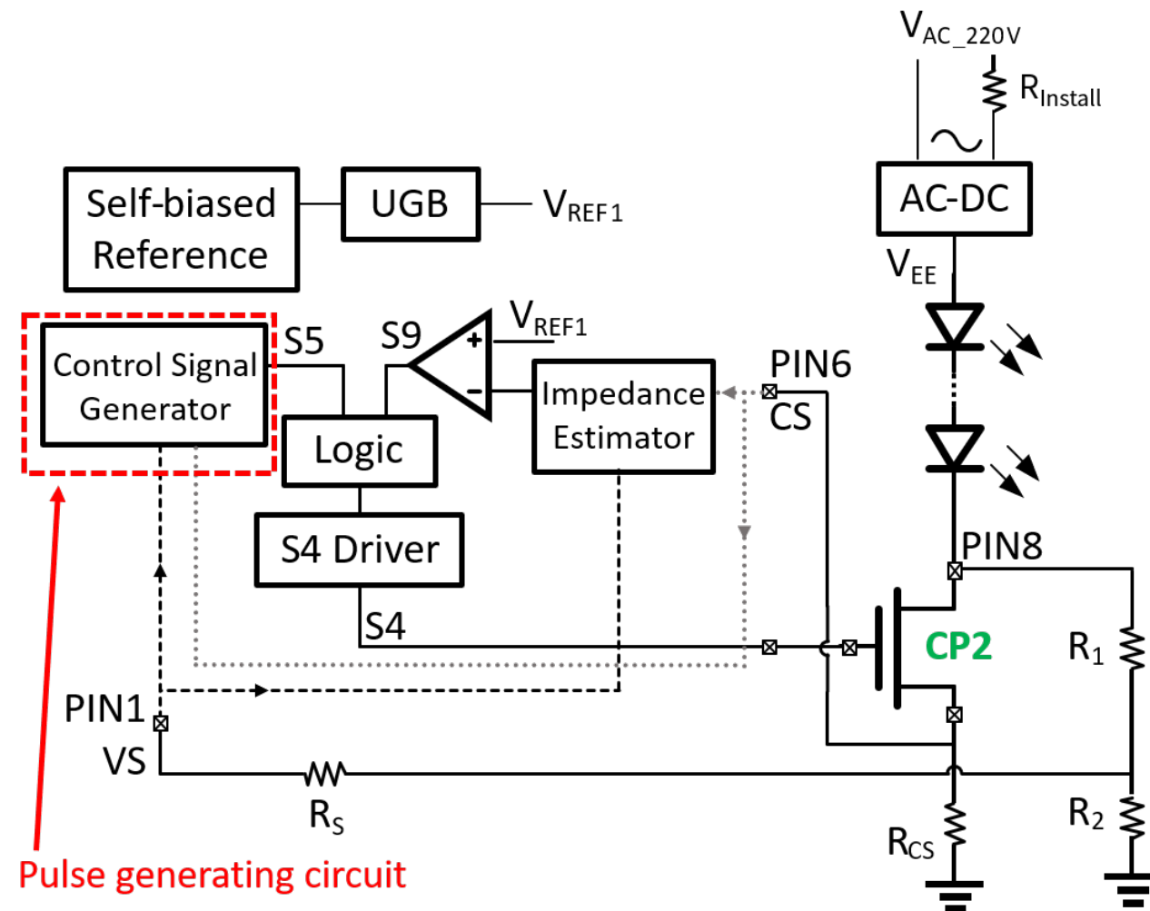
Figure 14. The pulse generating circuit is outline by the dashed red line and consists of circuitry contained on the CP1 die inside the LT2600G. The simulation result of signal S5 shown in Figure 15 further evident signal S5 outputted from control signal generator includes one or more pulse signals. The simulation was conducted based on the "BA12003_LT2600_CA_Report_v1.pdf" teardown report and the relevant raw data of the teardown analysis.
