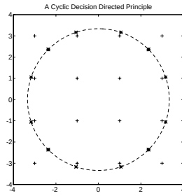
Figure 5: A CMA-DD hybrid principle: 16-QAM
