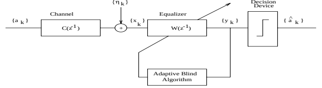
Figure 1: A typical blind equalization scheme
