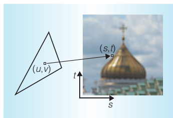
Figure 3. Texture mapping involves finding the corresponding color in a 2D image map in s, t coordinates using the texture coordinates u, v at the current pixel in a triangle.
