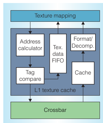
Figure 5. Overview of a texture cache architecture. The texture mapping unit provides texture coordinates for which a memory address is calculated. The address is sent to the tag compare to determine if the data is in the cache. If the data isn't in the cache, a request is sent via the crossbar to the L2 cache. Any state associated with the original request is sent into a first-in, first-out buffer (FIFO) to return to the texture mapping unit with the texel data. Once the data arrives in the cache, or is already available in the cache, it is returned to the texture mapping unit. If the data is compressed, it is decompressed and any necessary formatting is done.
