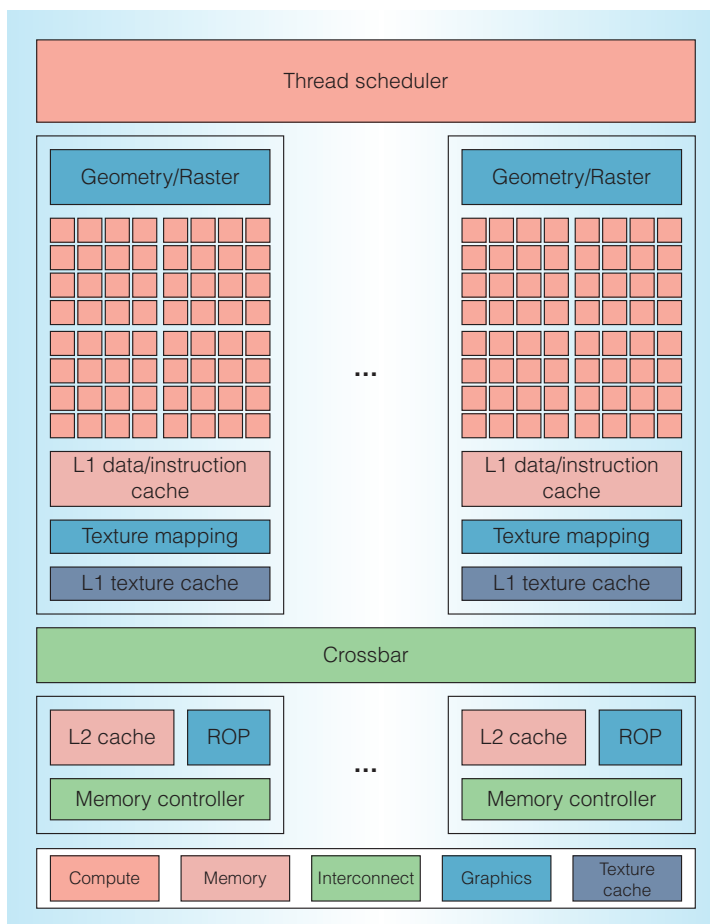
Figure 2. A simplified diagram of a modern GPU’s top-level architecture. The texture cache is located just above the crossbar and at the bottom of the shader. The thread scheduler collects workloads for the different stages of the graphics pipeline and loads them onto a variable number of graphics cores. The graphics cores have some fixed-function graphics logic in the geometry/raster unit, which contains geometry processing and rasterization. Underneath is the shader, which has control logic (not shown) and a grid of arithmetic logic units (ALUs) that process small programs in a single-instruction, multiple-data (SIMD) fashion. The shader uses the L1 data and instruction caches, texture mapping unit, and its associated texture cache as the programs are executed. The output of the shader and the connection of the L1s to the L2s goes via a crossbar, which is connected to a variable number of memory units containing the L2 cache, the ROP (fixed-function graphics), and the memory controller. The memory controller is connected to the external memory, where the framebuffer is stored. Most neighboring blocks are connected to each other, so interconnections between blocks are not shown.
