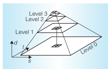
Figure 4. A sequence of images making a mipmap pyramid. Level 0 is the full resolution image, and each subsequent level is a half-size averaged version of the previous level. Texture filtering first calculates the level of detail, d , which selects two levels of the pyramid and then performs trilinear filtering between the two layers.
