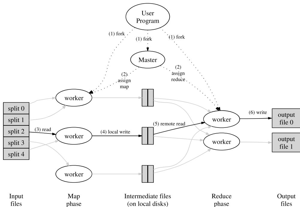
Figure 1: Execution overview
