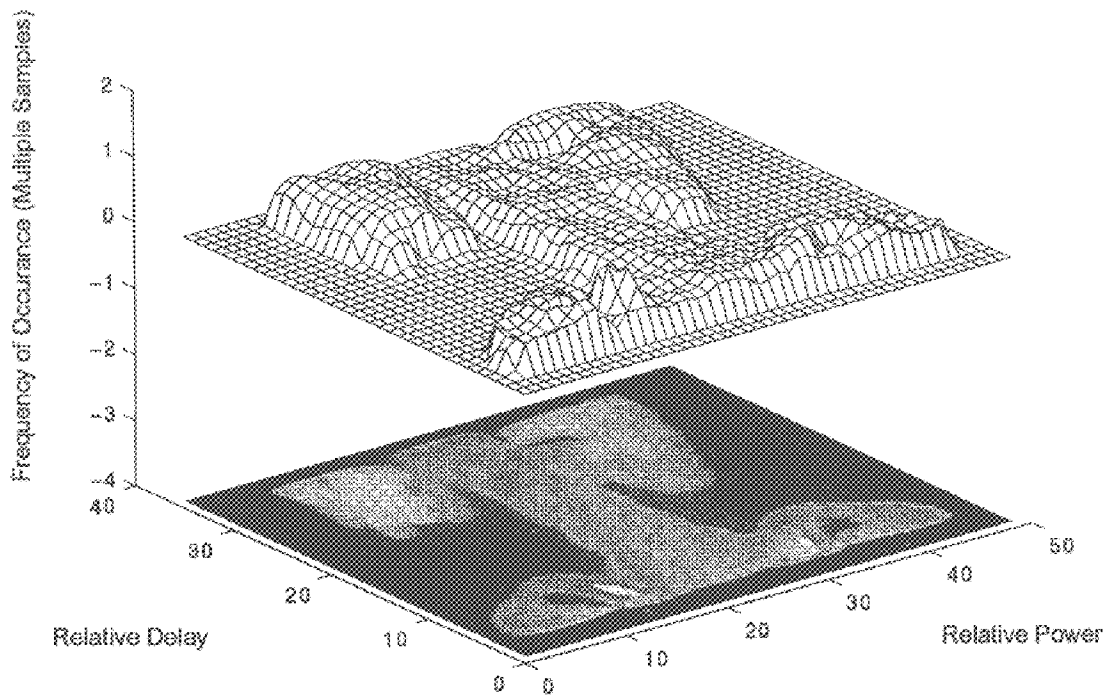
FIG. 28: IMAGE AND RELIEF REPRESENTATION OF A CDMA PROFILE
