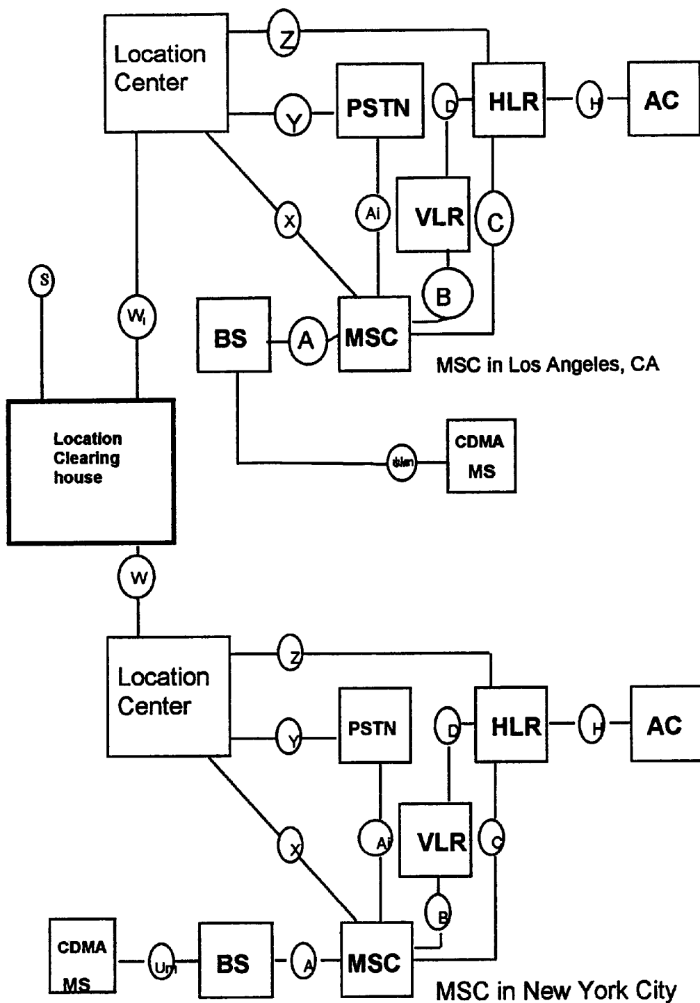
Figure 25: National Location Clearinghouse Structure
