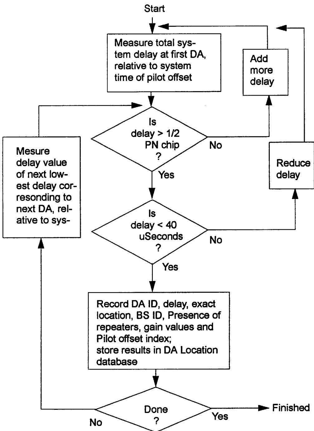
FIG. 8: DA Installation Procedure for Wireless Location
