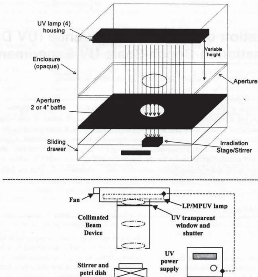
Fig. 1. Examples of bench scale devices for conducting UV experiments
