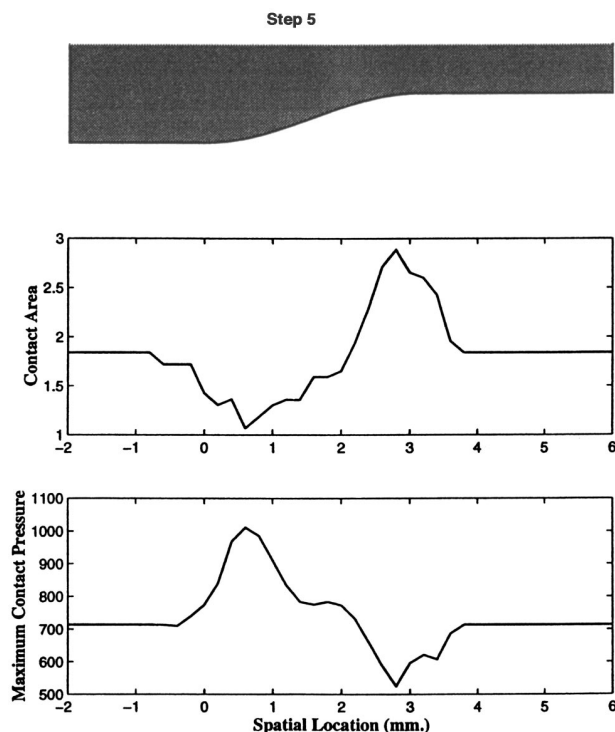
Fig. 12 The variation in contact area and maximum contact pressure for constant force of indentation of step 5 at various locations on the monkey fingertip model
