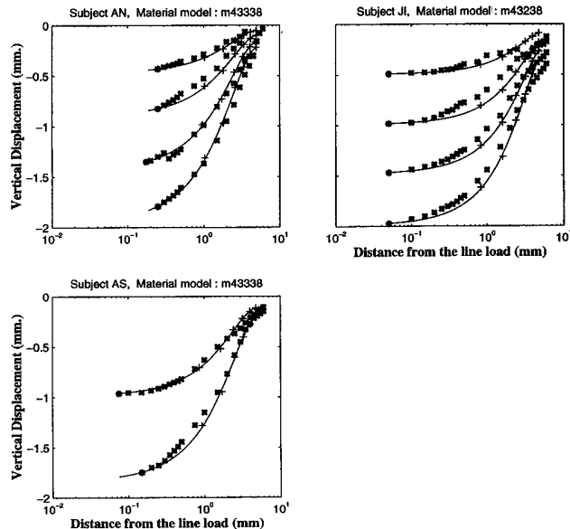
Fig. 10 Surface deformation of the human fingertip under line loads predicted by the finite-element model. The empirical data shown with crosses for three human subjects is from Srinivasan [3]. Same format as Fig. 9.
