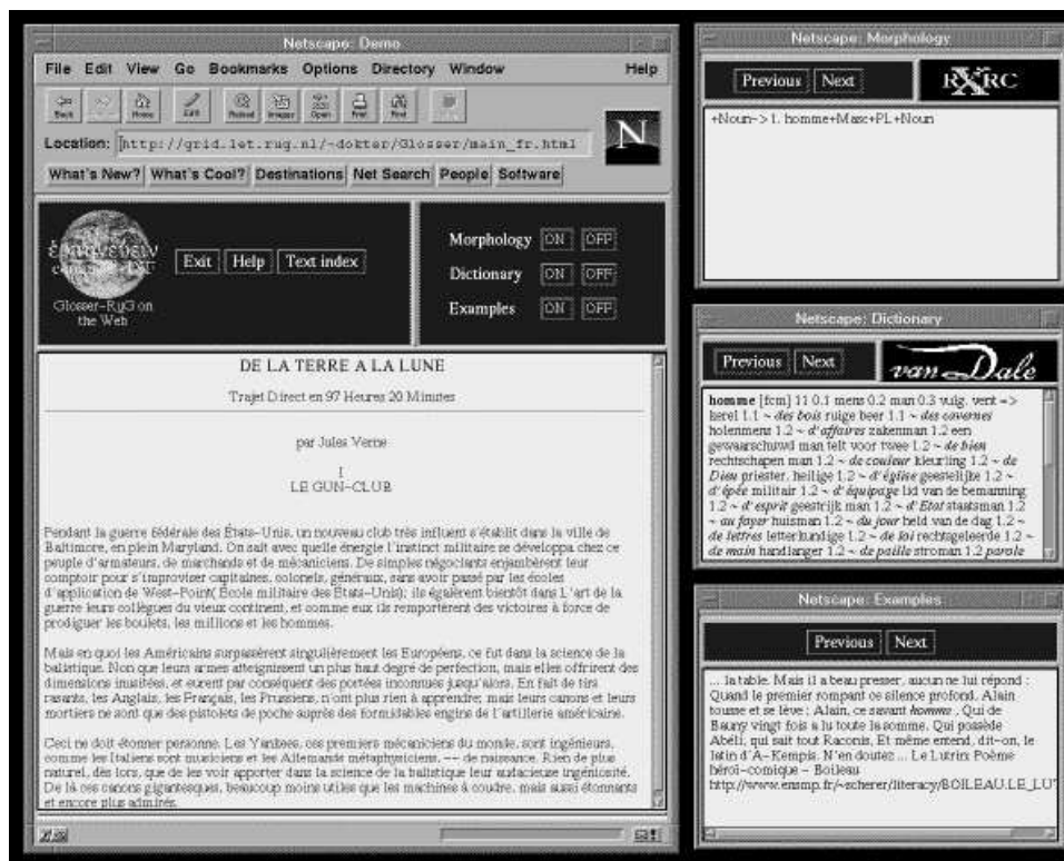
Figure 3: The front-end of Glosser-Web, provided that all sources of information are switched on. The help-window is omitted. The specific appearance is of course depending on the type of browser used.
