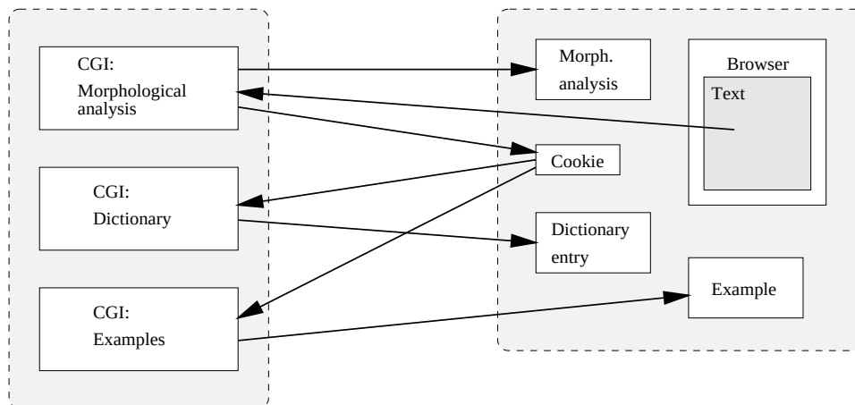
Figure 2: The flow of information between the major components of Glosser-Web.
