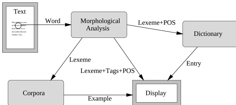
Figure 1: The flow of information for a single lookup within Glosser-RuG, given that all sources are activated.
