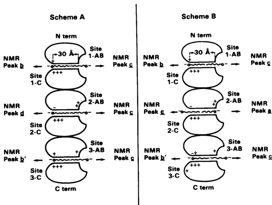
FIG. 6. Schematic diagram of the albumin molecule and its FA binding sites (modified from Brown and Schockley, 1982) depicting the three domains (six subdomains) and the postulated locations of FA binding sites which correspond to the observed ^{13}\text{C} NMR FA carboxyl peaks. The mouths of binding sites 1-AB, 2-AB, and 3-AB appear on the righthand side and the mouths of the binding sites 1-C, 2-C, and 3-C are on the left. Long-chain fatty acids are shown occupying three high-affinity long-chain binding sites on the left (1-C, 2-C, and 3-C) with their carboxyl headgroups at the entrance to the channel and their hydrocarbon chains within the channels. The lower affinity long-chain FA and short-chain FA binding sites are located on the right-hand side of the model (1-AB, 2-AB, and 3-AB). The bound FA molecules are scaled to represent 16:0 (~20 Å long). The length of the binding channel is 30 Å (Brown and Schockley, 1982), and this length cannot completely accommodate two 16:0 molecules. Hence, in some of the binding sites, the FA carboxyl group and several methylene groups protrude from the binding channel. Scheme A depicts a binding arrangement in domain 2 which would give rise to NMR peaks d and c . Scheme B represents an alternative binding affinity arrangement which would give rise to NMR peaks c and a . Within a given FA·BSA sample, a majority of individual FA·BSA complexes would have FA bound according to Scheme A and the remainder of complexes Scheme B. The proportion of complexes with FA bound according to Scheme A increases with increasing FA chain length.
