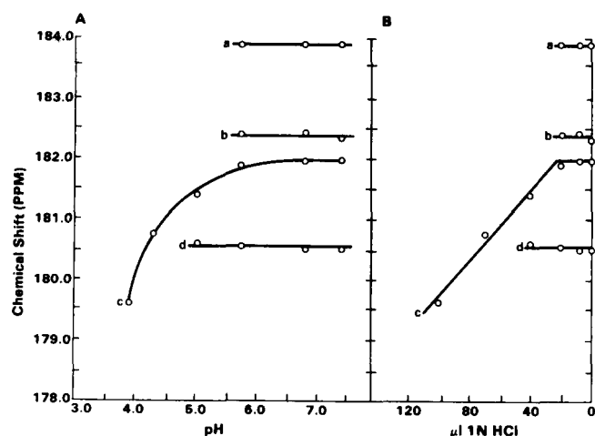
FIG. 6. ^{13}\text{C} NMR chemical shift titration curves for [1-^{13}\text{C}]\text{C}_{16:0}\text{-BSA} , 6:1 mol ratio, at 35^\circ\text{C} . A, FA carboxyl chemical shift plotted as a function of pH. B, FA carboxyl chemical shift plotted as a function of added HCl. The FA carboxyl peaks became undetectable below pH 4.0 (above 100 \mu\text{l} of HCl).
