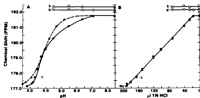
FIG. 5. ^{13}\text{C} NMR chemical shift titration curves for [1-^{13}\text{C}]\text{C}_{12:0}\text{-BSA} , 6:1 mol ratio, at 35^\circ\text{C} . Symbols are defined as described in the legend to Fig. 4. A, FA carboxyl chemical shifts as a function of pH. B, FA carboxyl chemical shifts plotted as a function of added HCl.
