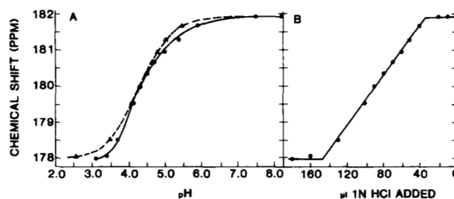
FIG. 2. 13 C NMR chemical shift titration curves for [ 1-13 C]C 8:0 ·BSA, 6:1 mol ratio, at 35 °C. A, FA carboxyl chemical shift plotted as a function of pH. ●—●, experimentally determined curve; ▲—▲, theoretically calculated Henderson-Hasselbalch curve. 2 B, FA carboxyl chemical shift plotted as a function of added HCl.
