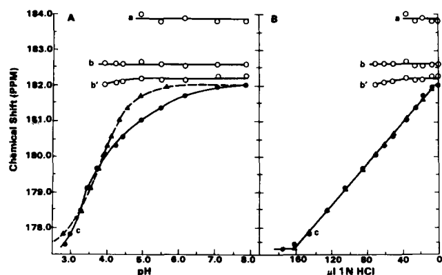
FIG. 4. ^{13}\text{C} NMR chemical shift titration curves for [1-^{13}\text{C}]\text{C}_{14:0}\text{-BSA} , 6:1 mol ratio, at 35^\circ\text{C} . \circ — \circ , experimentally determined curves for peaks a, b, and b' (see Fig. 3); \bullet — \bullet , experimentally determined curves for peak c (Fig. 3); \blacktriangle — \blacktriangle , theoretically calculated Henderson-Hasselbalch curves for peak c. 2 The experimental data points were derived from the NMR spectra shown in Fig. 3 as well as other spectra not shown. A, FA carboxyl chemical shifts plotted as a function of pH. B, FA carboxyl chemical shifts plotted as a function of added HCl.
