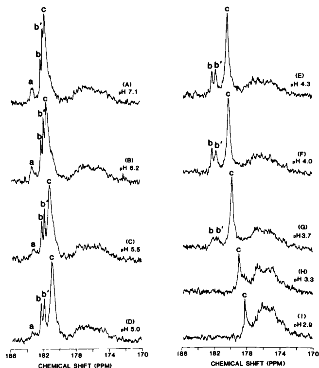
FIG. 3. Carboxyl/carbonyl region of ^{13}\text{C} NMR spectra for [1-^{13}\text{C}]\text{C}_{14:0}\text{-BSA} , 6:1 mol ratio, at different pH values at 34^\circ\text{C} . Spectra were recorded after 6,000 accumulations with a pulse interval of 2.5 s, 16,384 time domain points, and a spectral width of 10,000 Hz. Identical scaling and processing factors (including 3.0-Hz line broadening) were used for each spectrum. The lower case letters above certain peaks indicate specific FA carboxyl resonances with characteristic chemical shifts at pH 7.4 (Cistola et al. , 1987).
