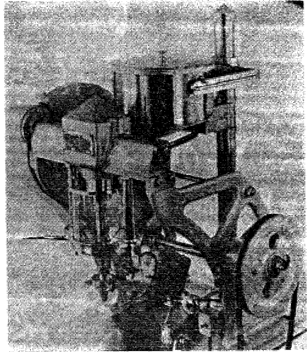
Figure 41-21. Auger-type powder filler (courtesy, Chase-Logeman).
