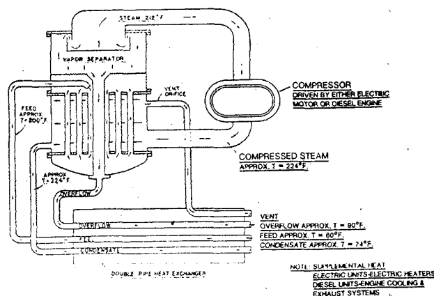
Figure 41-2. Vapor-compression still.
