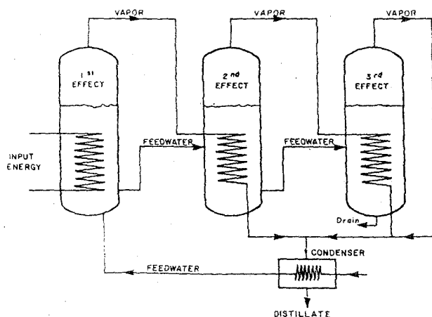
Figure 41-3. Multiple-effect still (courtesy, Dekker). (From Avis KE, Lieberman HA, Lachman L. Pharmaceutical Dosage Forms: Parenteral Medications . 2nd ed. New York: Dekker, 1993.)
