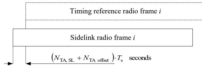
Figure 9.9-1: Sidelink timing relation.
