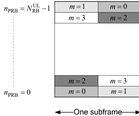
Figure 5.4.3-1: Mapping to physical resource blocks for PUCCH formats 1 – 3
