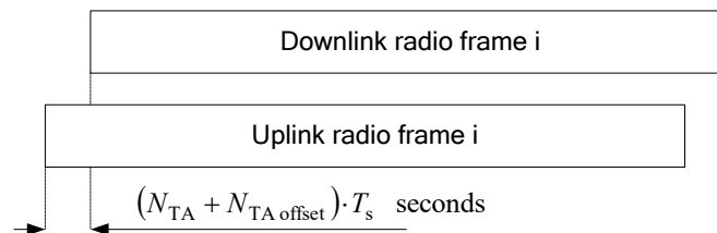
Figure 8.1-1: Uplink-downlink timing relation
