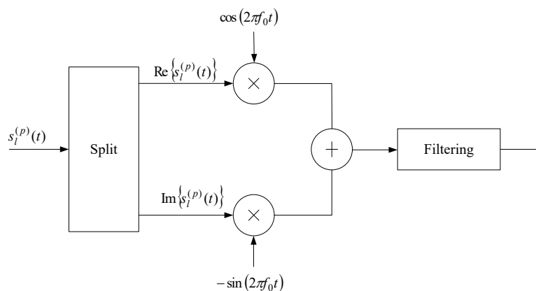
Figure 6.13-1: Downlink modulation
