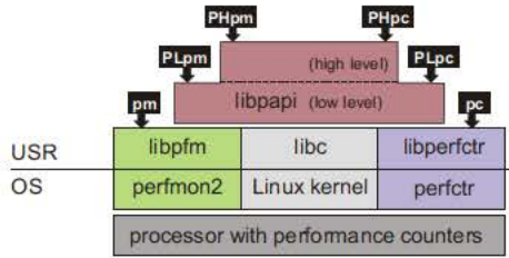
Figure 2. Counter access infrastructure
