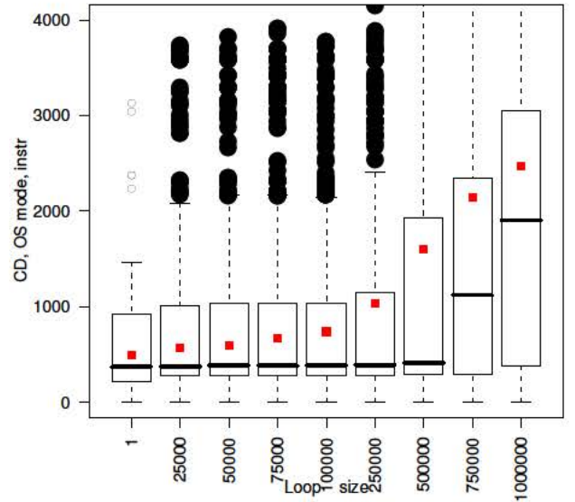
Figure 7. Kernel mode instructions by loop size (pc on CD)
