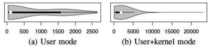
Figure 1. Number of overcounted instructions
