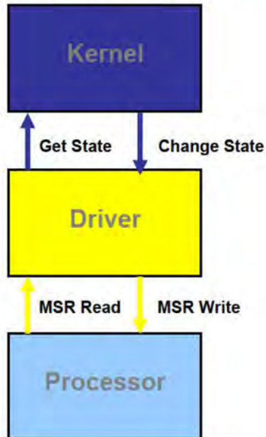
Figure 1.2 Software Model for Windows XP and Windows Server 2003
