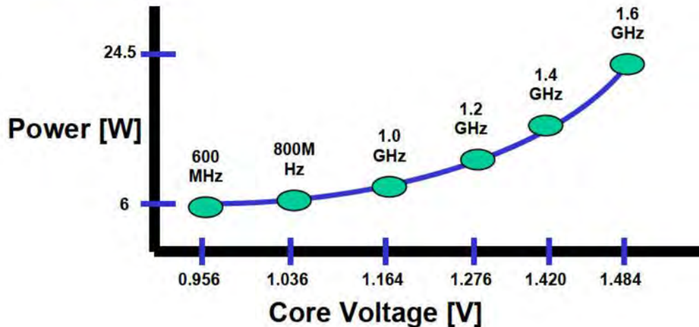
Figure 1.1 Power vs. Core Voltage for the Intel® Pentium® M Processor at 1.6GHz for its six frequency/voltage operating points (not to scale). HFM and LFM power values are TDP specifications.
