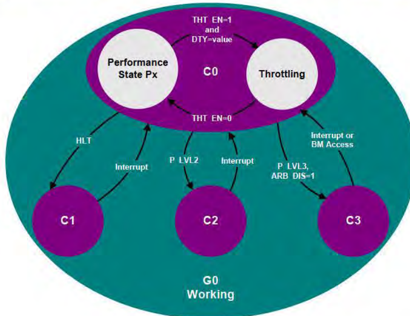
Figure 1.4 Processor Performance States (P-states) Discussed Herein Are Sub-States of C0
