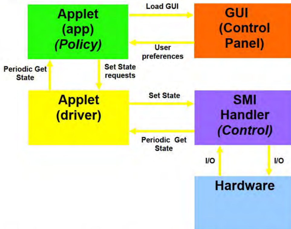
Figure 1.3 Software Model for the Enhanced Intel® SpeedStep® Technology Applet on Legacy Windows Platforms
