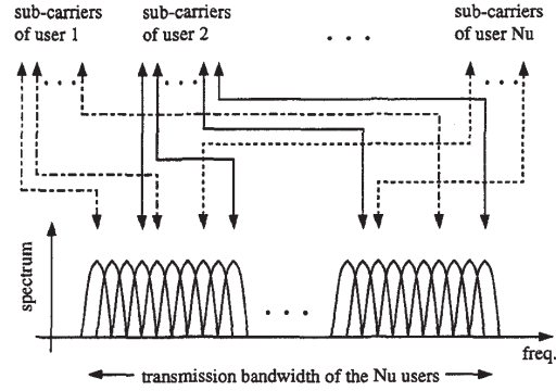
Figure 2: Pseudo-random user-specific frequency-mapping and -demapping.
