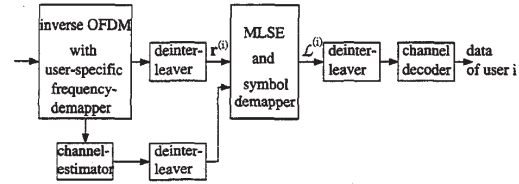
Figure 3: SS-MC-MA receiver for the data of user i .
