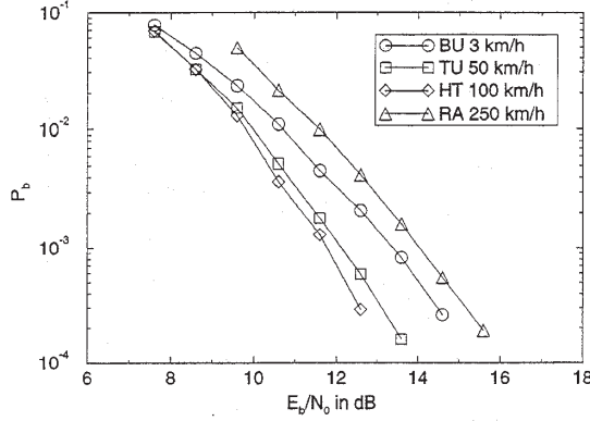
Figure 5: Performance of SS-MC-MA in different propagation scenarios with full system load.
