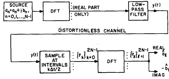
Fig. 2. Fourier transform communication system in absence of channel distortion.
