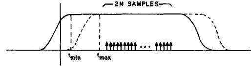
Fig. 7. Shifted versions of g_a(t) corresponding to subchannels with minimum and maximum delay and locations of samples taken by receiver. Here t_{\min} = \min_n \beta_n , t_{\max} = \max_n \beta_n .
