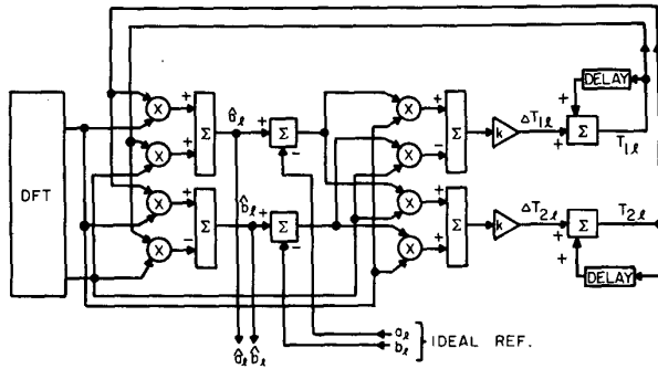
Fig. 8. Automatic equalizer for Fourier transform receiver. One such apparatus is required for each of the (n - 1) usable outputs of the discrete Fourier transformer.
