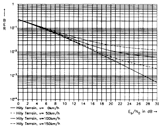
Fig. 6. Hilly Terrain channel: BER versus E_b/N_0
