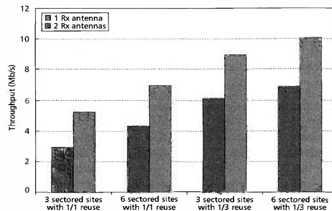
Figure 14–1: WirelessMAN-OFDM throughput per 5 MHz channel
