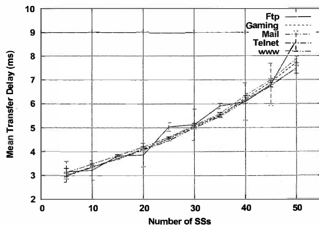
Figure 14-4: DL, IP traffic mean transfer delay
