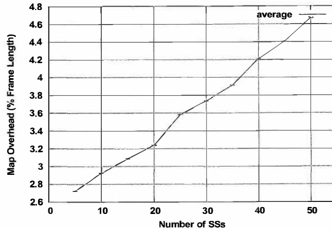
Figure 14-8: FCH + MAP overhead
