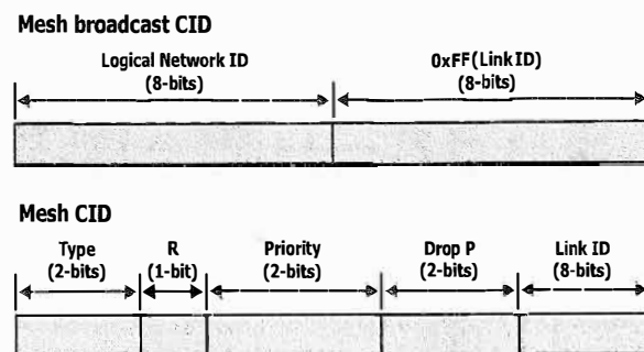
Figure 9-4: Mesh CIDs
