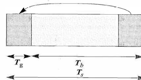
Figure 11-1: OFDM symbol structure
