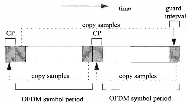
Figure 12-7: Single-slot initial ranging transmission for OFDMA
