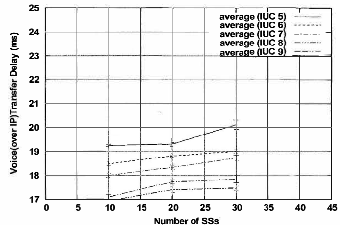
Figure 14-9: UL, full-duplex SSs, VoIP mean transfer delay
