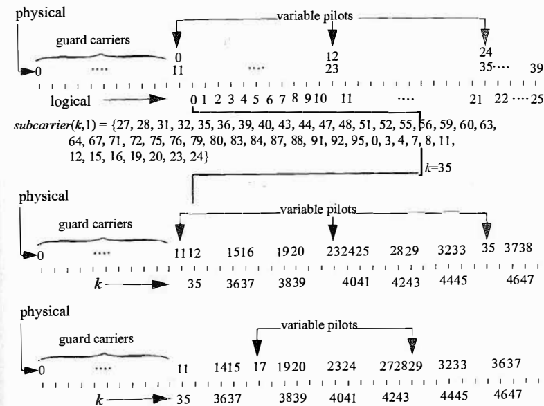
Figure 12-2: FUSC mapping example
