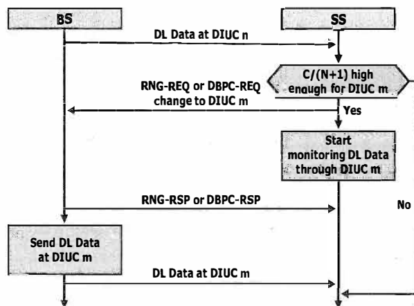
Figure 7-14: Transition to less robust burst profile
