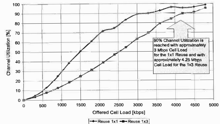
Figure 14-16: Channel utilization as function of offered load
