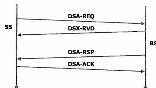
Figure 7-15: DSA message flow—SS initiated
