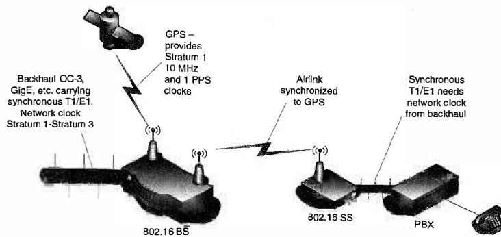
Figure 7-19: Clock comparison
