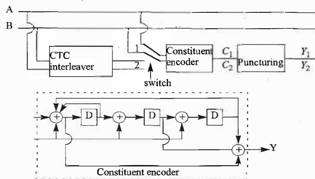
Figure 11-10: CTC encoder
