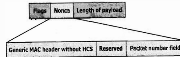
Figure 8-2: Initial CBC block and nonce
