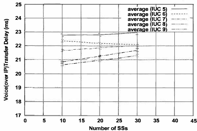
Figure 14-10: UL, half-duplex SSs, VoIP mean transfer delay
