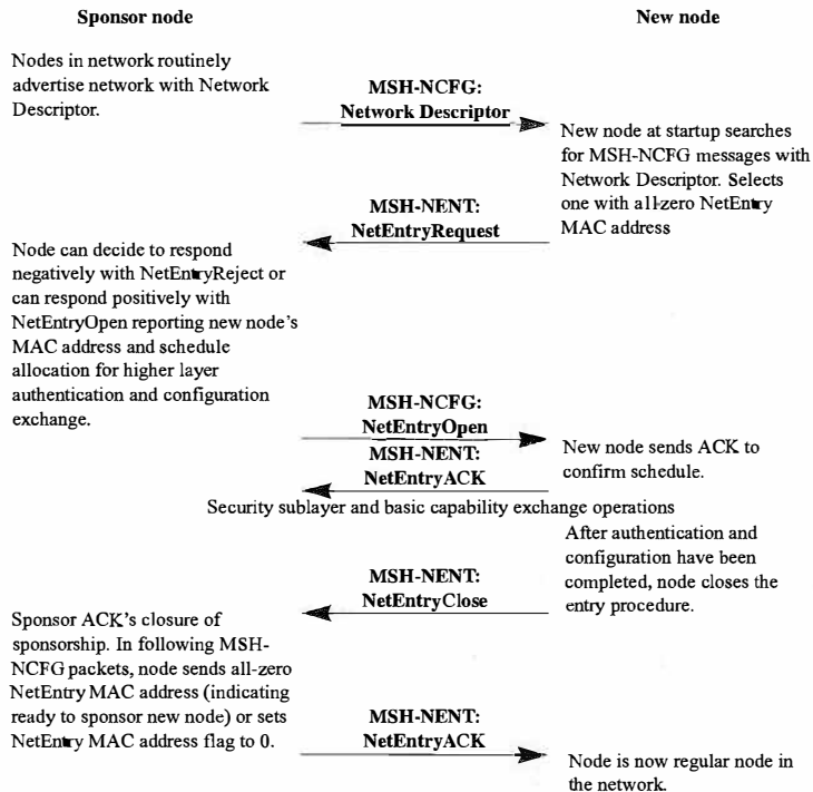
Figure 9–5: Mesh network entry: Opening a sponsor channel
