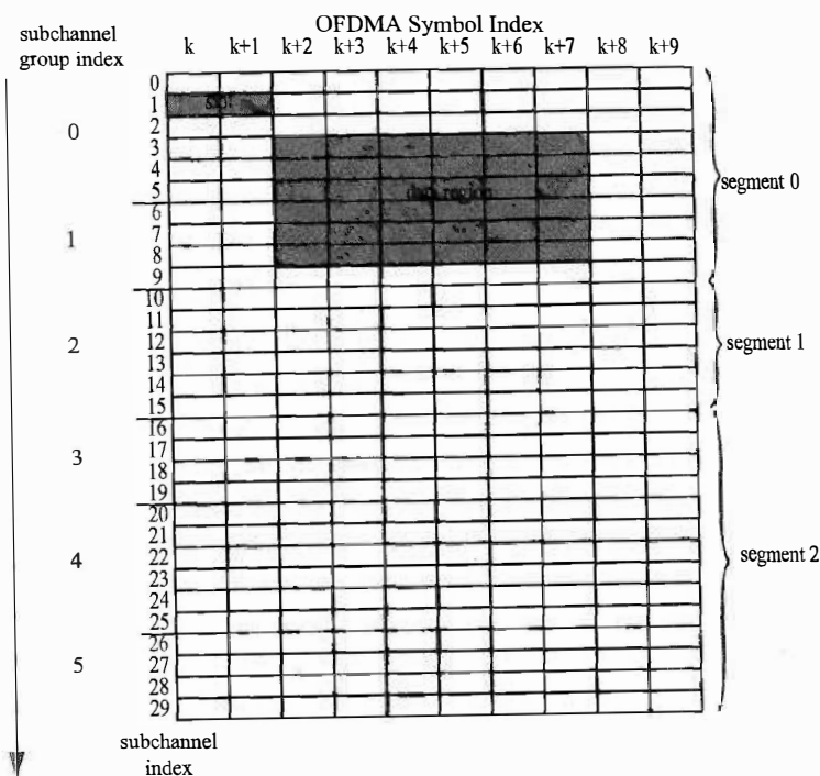
Figure 12-1: Schematic indication of logical mapping elements
