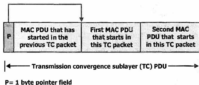
Figure 10-4: Format of DL transmission CS PDU
