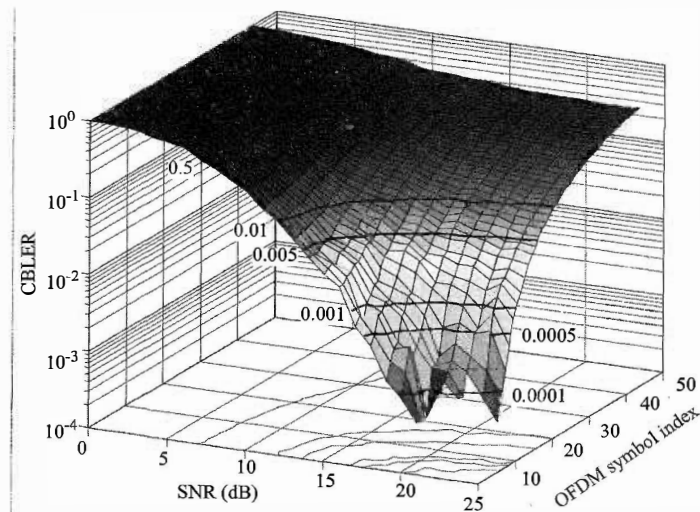
Figure 14-15: OFDM CBLERs—ITU VehA 30 km/h
