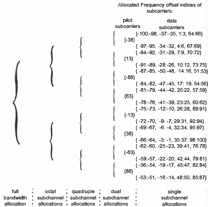
Figure 11-3: Subchannel subcarrier allocations
