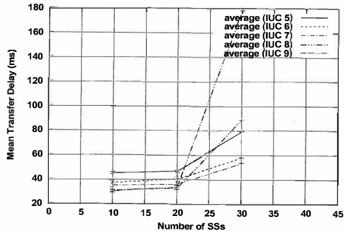
Figure 14-13: UL, half-duplex SSs, HTTP mean transfer delay w/ARQ
