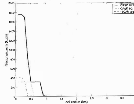
Figure 14-22: UL sector capacity per cell radius (ITU outdoor-indoor)
