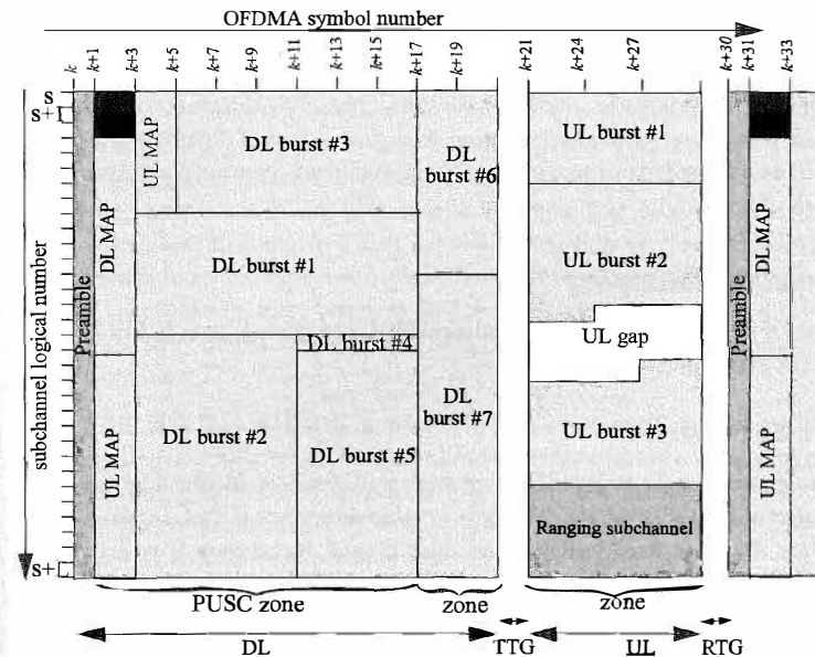
Figure 12-5: Frame structure (TDD)
