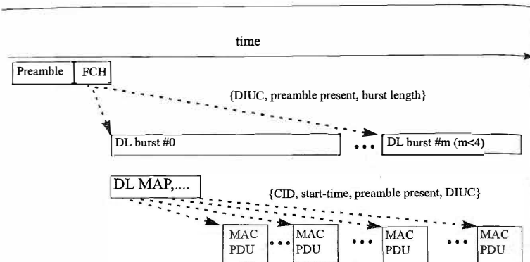
Figure 11-6: DL burst and MPDU mapping
