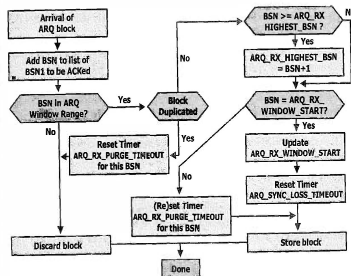
Figure 7-21: ARQ block reception
