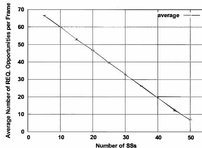
Figure 14-6: UL, Average transmit opportunities per frame
