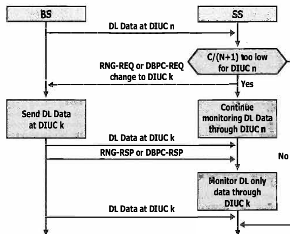
Figure 7-13: Transition to more robust burst profile
