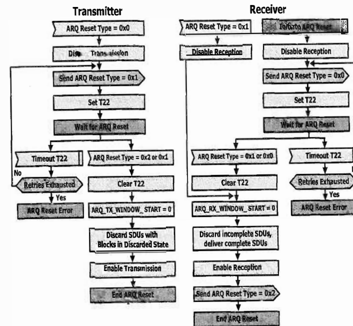
Figure 7-23: Receiver-initiated reset
