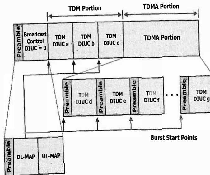
Figure 10-2: FDD DL subframe structure
