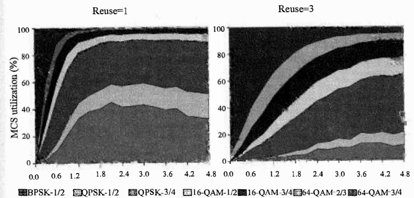
Figure 14-17: Modulation/coding utilization as function of offered load
