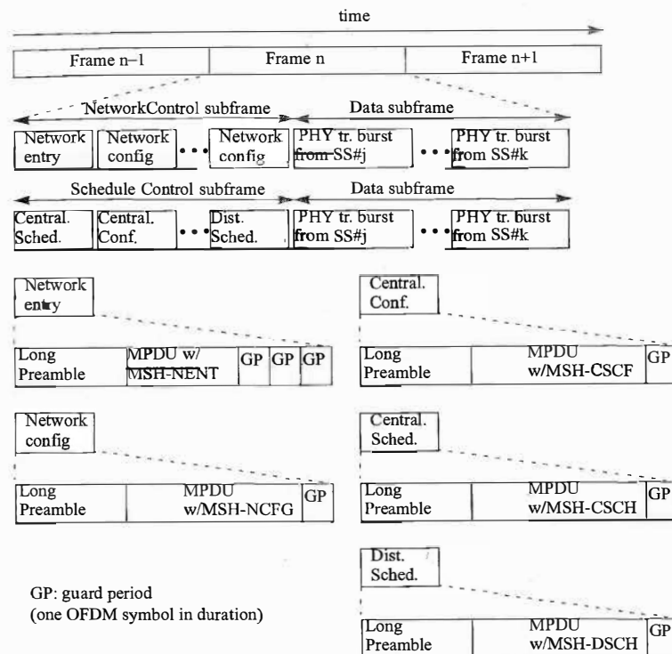
Figure 11-7: Mesh frame structure
