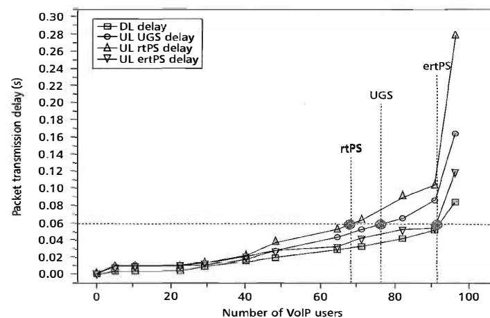
Figure 14-23: Delay for VoIP using rtPS, UGS, and ertPS
