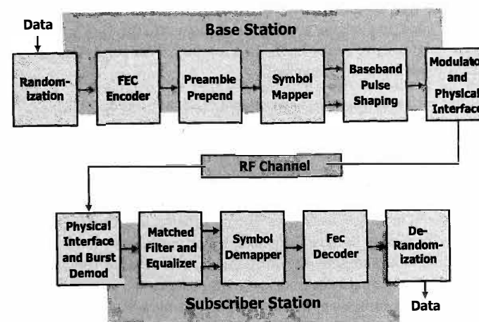
Figure 10-5: Conceptual block diagram of DL PHY
