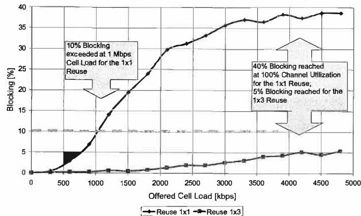
Figure 14–18: Call blocking (C/I < 1 dB) as function of offered load
