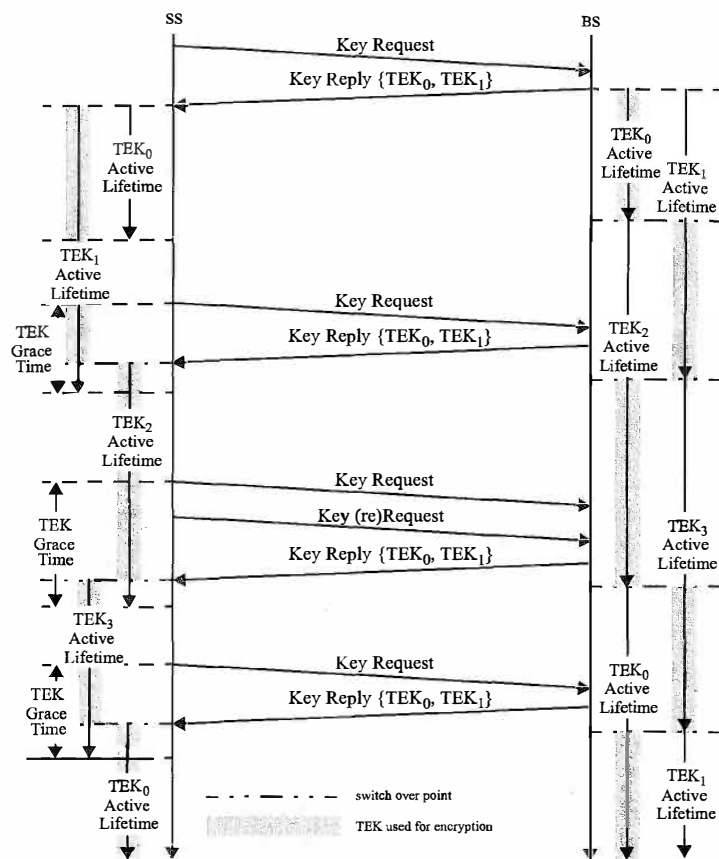
Figure 8-5: TEK management in BS and SS
