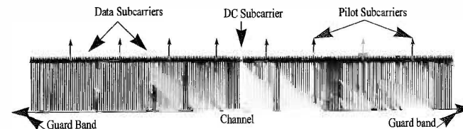
Figure 11-2: OFDM frequency description
