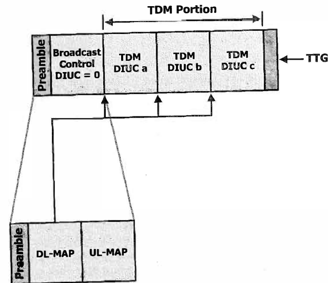
Figure 10-1: TDD DL subframe structure
