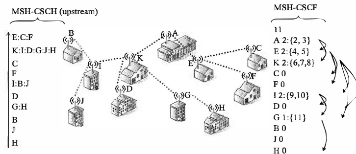
Figure 9-7: Centralized scheduling
