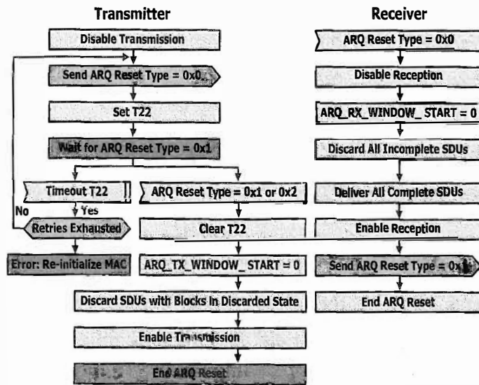
Figure 7-22: Transmitter-initiated reset
