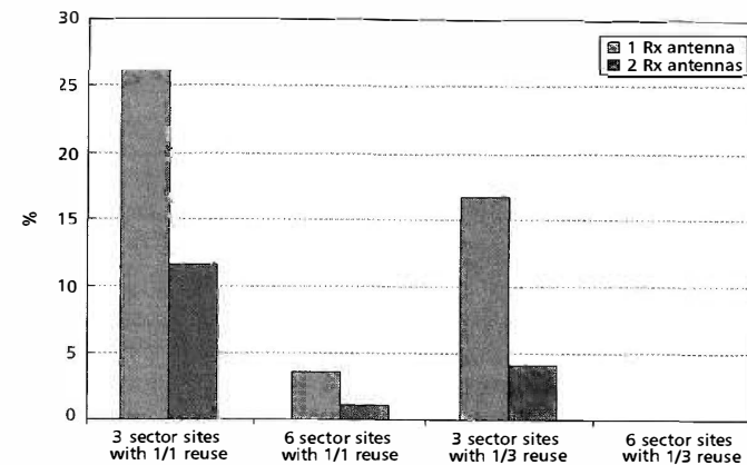
Figure 14–2: WirelessMAN-OFDM outage relative to 1.5 Mbit/s
