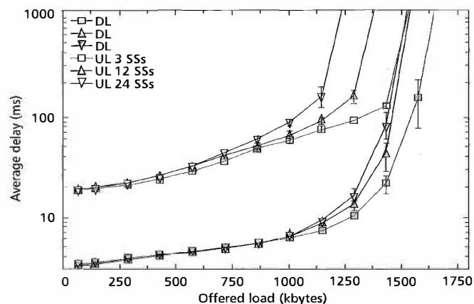
Figure 14-3: Average throughput delay vs offered load
