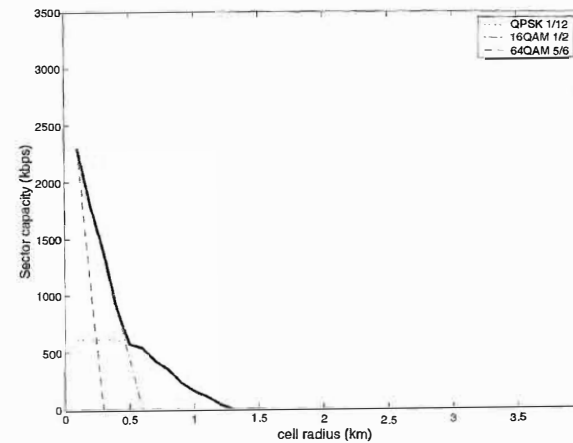
Figure 14-21: DL sector capacity per cell radius (ITU outdoor-indoor)
