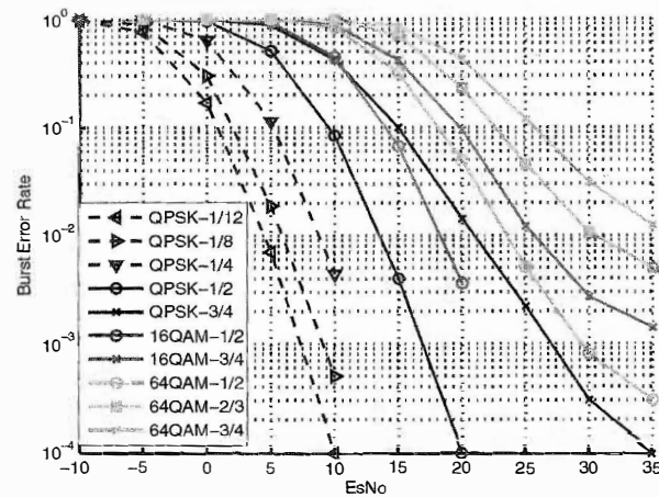
Figure 14-26: CBLER, UL PUSC, ITU VehA 3 km/h, CC, estimated
