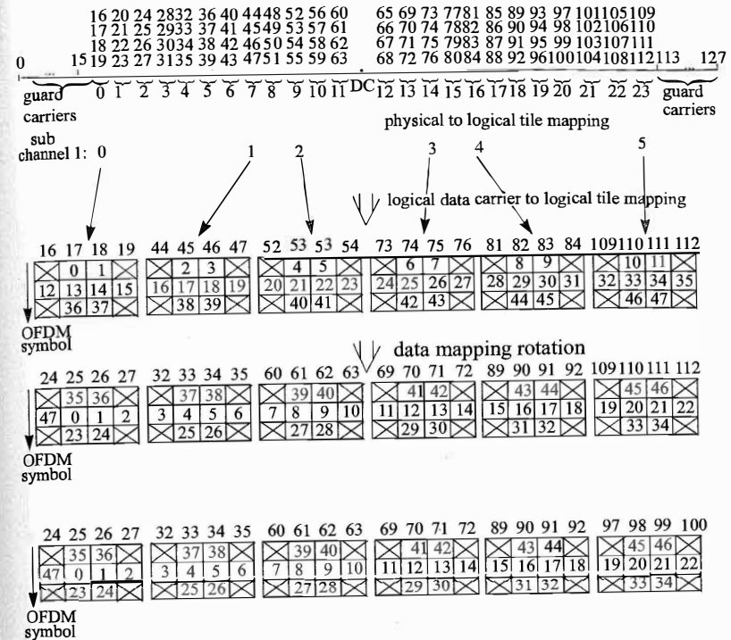
Figure 12-4: PUSC UL mapping example
