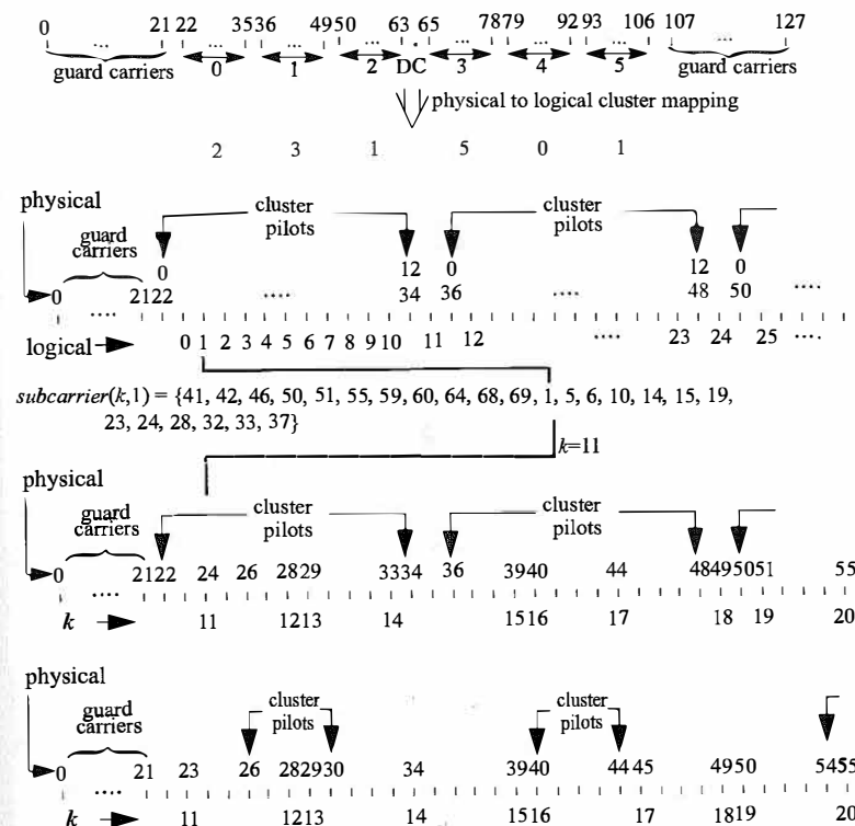
Figure 12-3: PUSC DL mapping example
