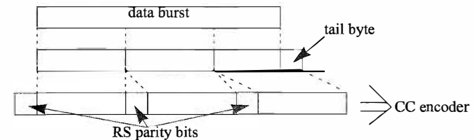
Figure 11–8: RS-CC encoding process
