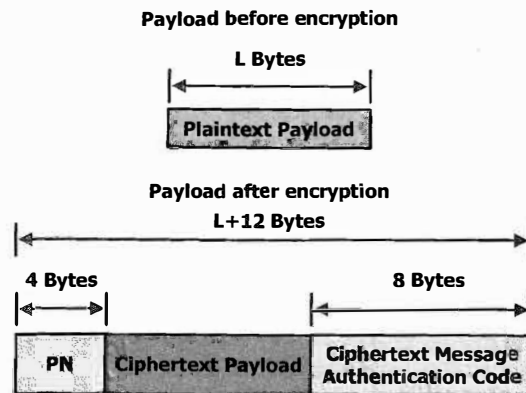
Figure 8-1: Encrypted payload format in AES-CCM mode
