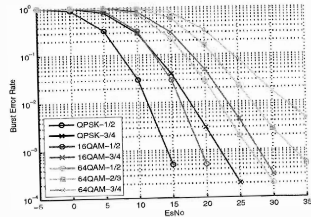
Figure 14-27: CBLER, UL PUSC, ITU VehA 120 Km/h, CC, ideal
