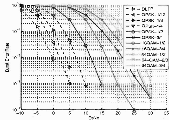
Figure 14-30: CBLER, DL PUSC, ITU VehA 3 km/h, CC, ideal
