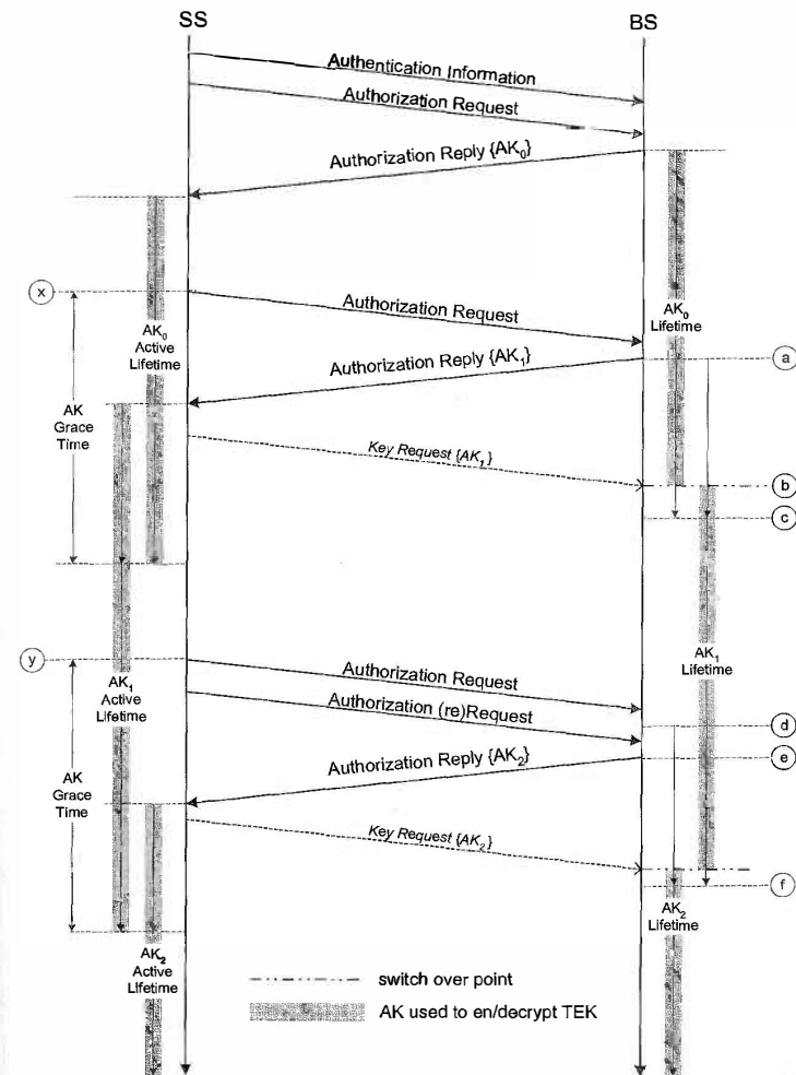
Figure 8-4: AK management in BS and SS
