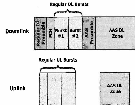
Figure 13-3: FDD framing for AAS systems
