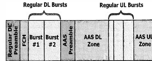
Figure 13-2: TDD framing for AAS Systems
