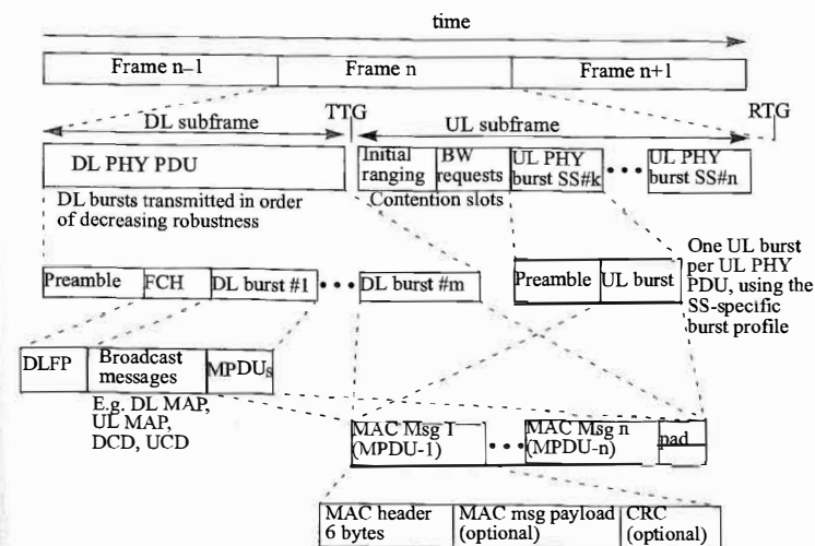
Figure 11-5: Example OFDM structure with TDD
