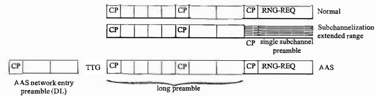
Figure 11–11: Initial ranging formats
