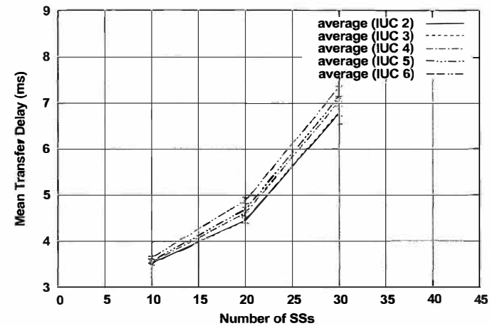
Figure 14-11: DL, half-duplex SSs, HTTP mean transfer delay
