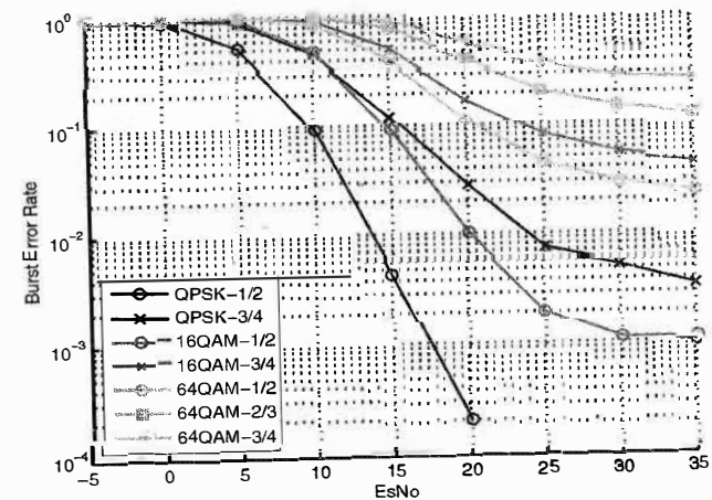
Figure 14-28: CBLER, UL PUSC, ITU VehA 120 km/h, CC, estimated
