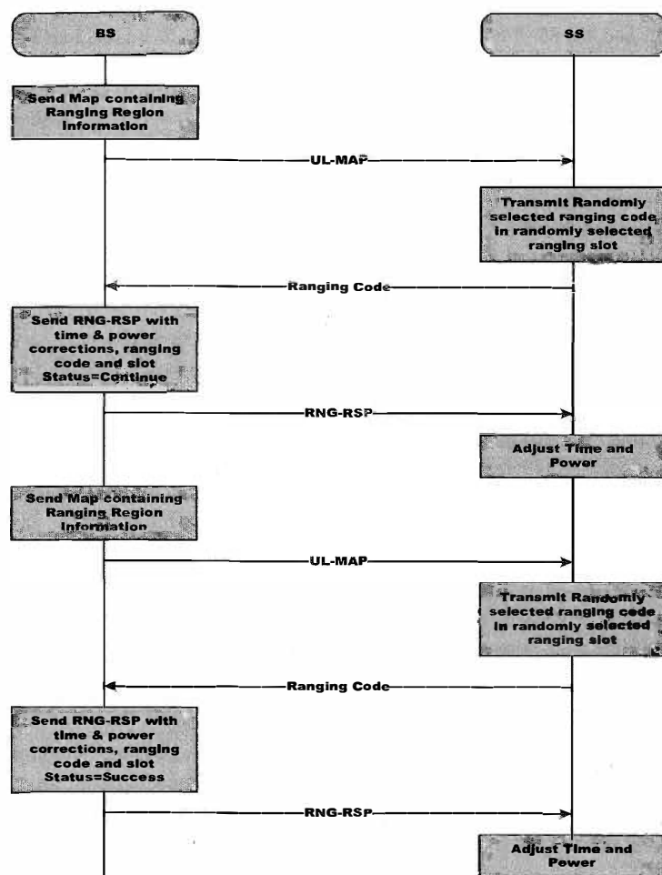
Figure 7-12: CDMA periodic ranging
