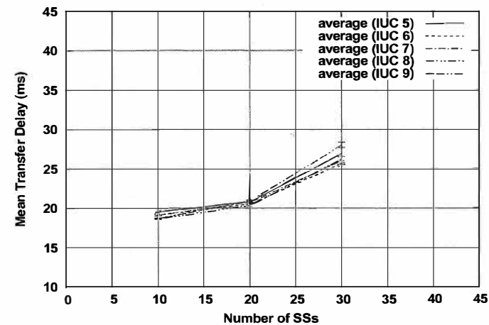
Figure 14-12: UL, half-duplex SSs, HTTP mean transfer delay
