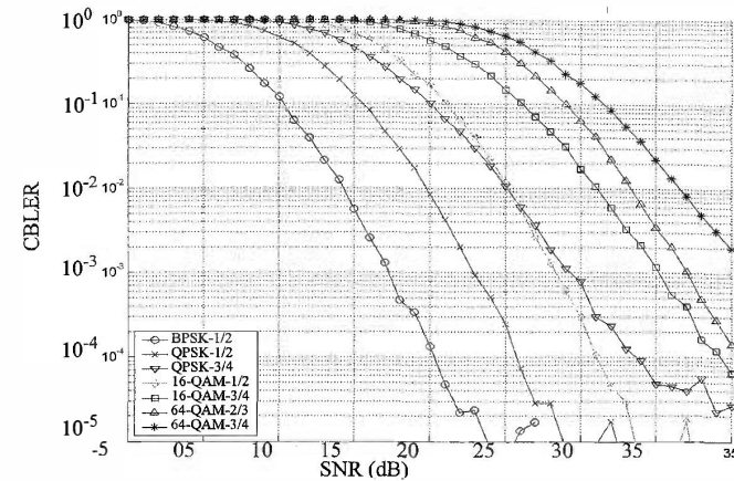
Figure 14-14: OFDM CBLERs—ITU VehA 3 km/h
