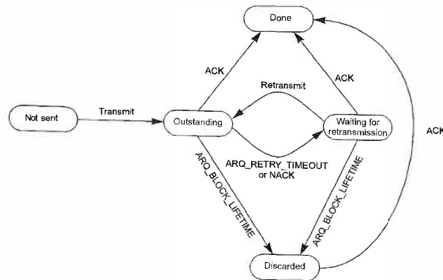
Figure 7-20: ARQ block states at the transmitter
