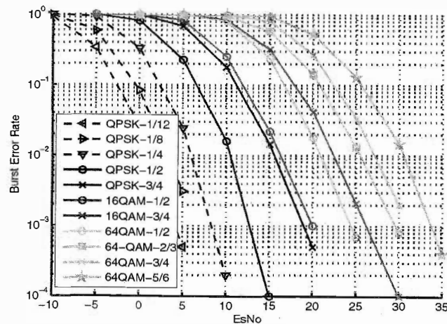
Figure 14-29: CBLER, UL PUSC, ITU VehA 3 km/h, CTC, ideal
