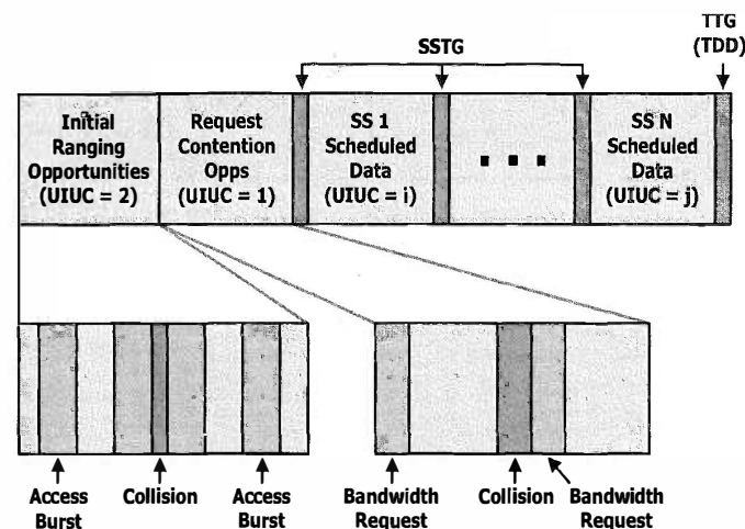
Figure 10-6: UL subframe structure
