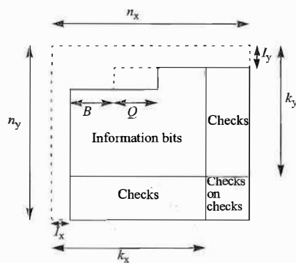
Figure 11-9: BTC encoding block
