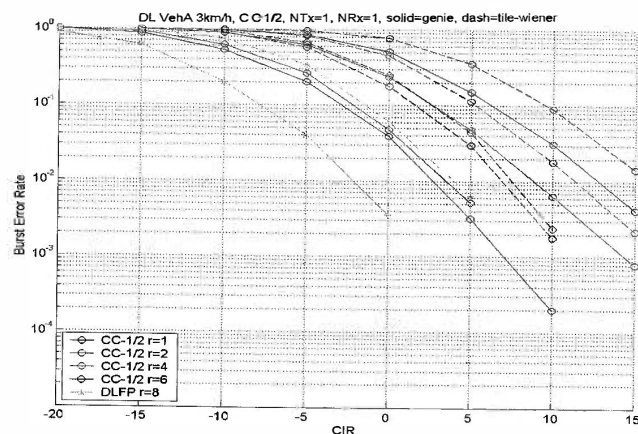
Figure 14-31: CBLER, DL PUSC, ITU VehA 3 km/h, CC, ideal
