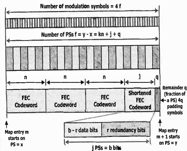
Figure 10-3: DL MAP usage with shortened FEC blocks—TDM case
