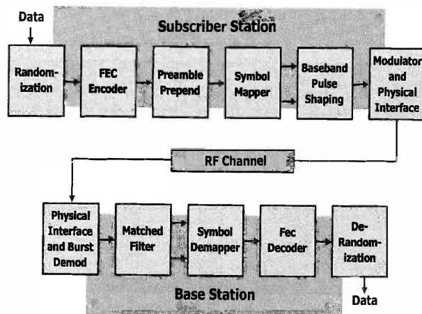
Figure 10-7: Conceptual block diagram of UL PHY
