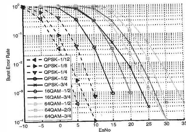
Figure 14-25: CBLER, UL PUSC, ITU VehA 3 km/h, CC, ideal
