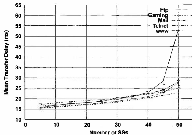
Figure 14-5: UL, IP traffic mean transfer delay
