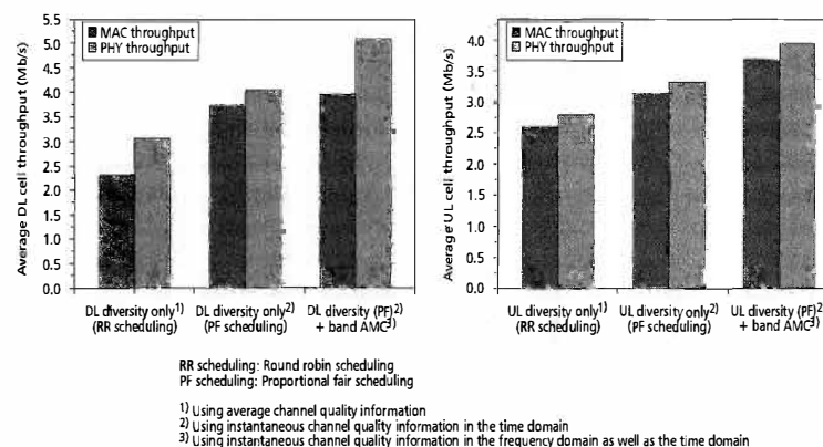
Figure 14-24: Average cell throughput for various schemes
