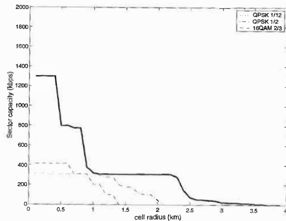
Figure 14-20: UL sector capacity per cell radius—ITU VehA (60 km/h)
