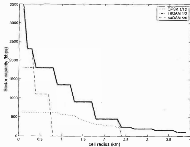
Figure 14-19: DL sector capacity per cell radius—ITU VehA (60 km/h)
