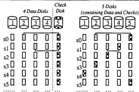
(a) Check information for Level 4 RAID for G=4 and C=1 . The sectors are shown below the disks. (The checked areas indicate the check information.) Writes to s0 of disk 2 and s1 of disk 3 imply writes to s0 and s1 of disk 5. The check disk (5) becomes the write bottleneck.
