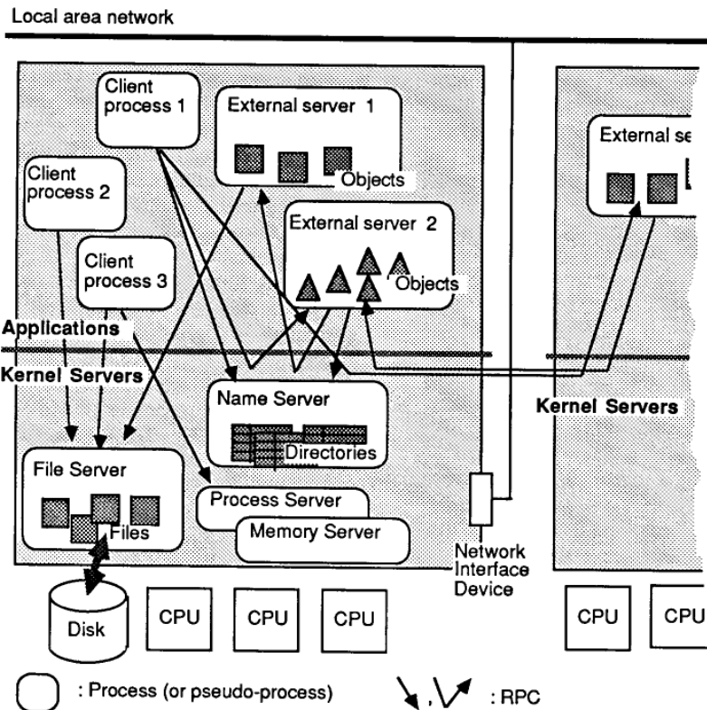
Figure 5: An overview of the ReSC distributed operating system.
