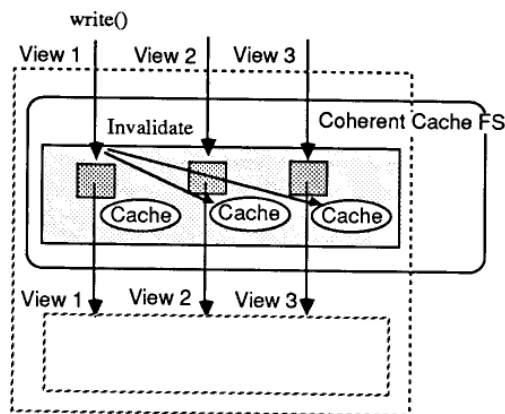
Figure 9: Coherent Cache File Server.
