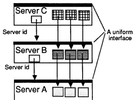
Figure 4-a: Server-stacking with objects.
