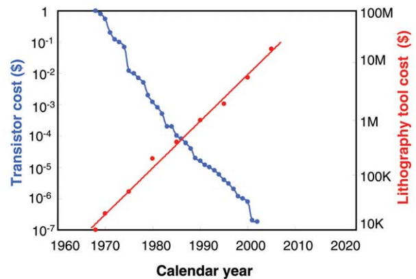
Fig. 2 Transistor cost and lithographic tool cost versus years. Note transistor cost has decreased seven orders of magnitude even while tool cost has increased.
