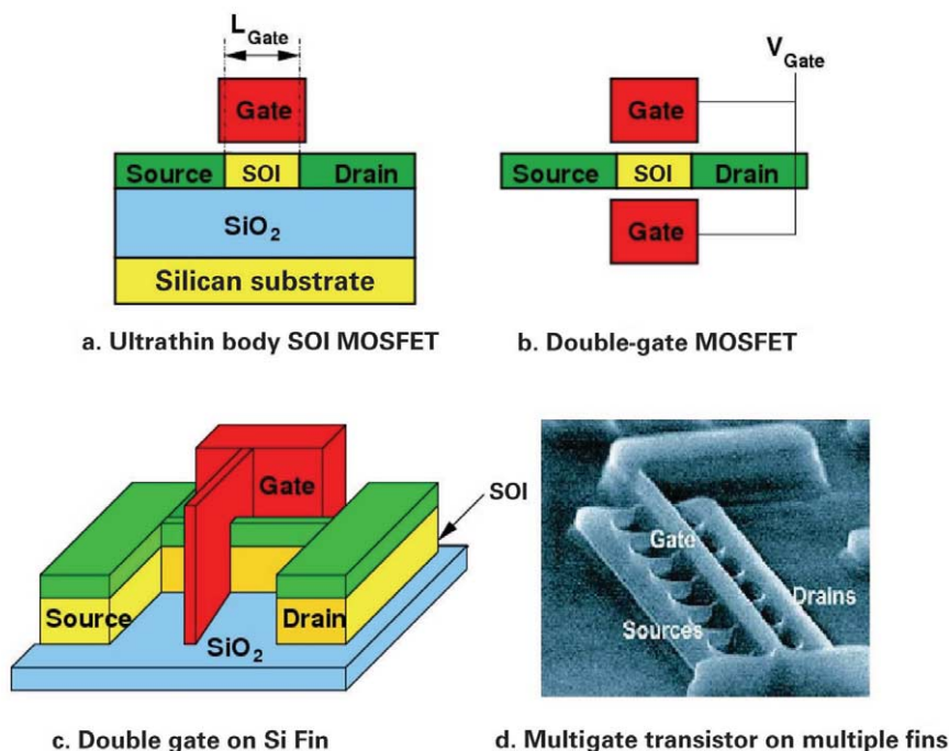
Fig. 3 Emerging alternative fully depleted CMOS structures for continue scaling: (a) one-, (b, c) two-, and (d) three-gate fully depleted devices. (Part (d) courtesy of R. Chau, Intel.)
