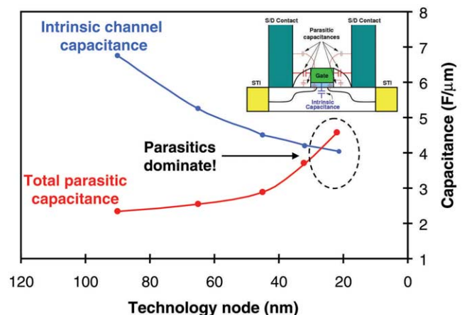
Fig. 6 Total planar CMOS parasitic and intrinsic channel capacitance versus technology node. Note parasitic capacitance is on course to become larger than intrinsic channel capacitance.
