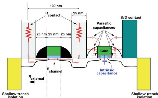
Fig. 4 Planar CMOS schematic showing the various parasitic resistances and capacitances (drawn to scale for the 32 nm process technology node, transistor pitch = 100 nm).
