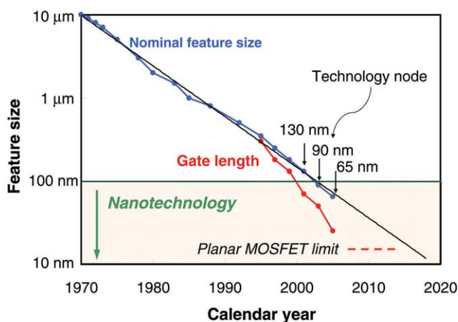
Fig. 1 Logic technology node and transistor gate length versus calendar year. Note mainstream Si technology is nanotechnology. (Published at the International Electron Devices Meeting.)
