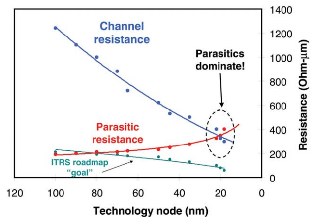
Fig. 5 Estimated total planar CMOS parasitic and channel resistance versus technology node. Note parasitic resistance is on course to become larger than the intrinsic channel resistance.
