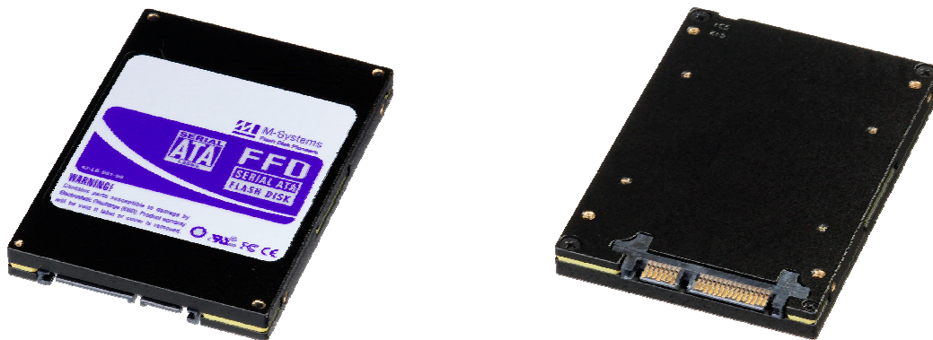
Figure 1: M-Systems' SATA solid-state flash disks incorporate the new SATA hot-swap connector.
