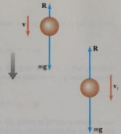
Figure 5.13 An object falling through air experiences a resistive drag force R and a gravitational force mg . The object reaches terminal speed (on the right) when the net force is zero, that is, when R = -mg , or R = mg . Before this occurs, the acceleration varies with speed according to Equation 5.9.
