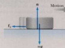
Figure 5.3 (Example 5.1) After the puck is given an initial velocity, the external forces acting on it are the weight, mg , the normal force, n , and the force of kinetic friction, f_k .
