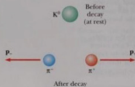
Figure 8.3 (Example 8.2) A kaon at rest decays spontaneously into a pair of oppositely charged pions. The pions move apart with momenta of equal magnitudes but opposite directions.
