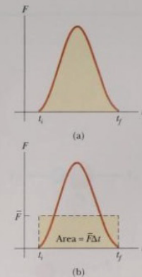
Figure 8.4 (a) A force acting on a particle may vary in time. The impulse is the area under the force-versus-time curve. (b) The average force (horizontal dashed line) gives the same impulse to the particle in the time \Delta t as the time-varying force described in (a).
