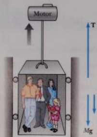
Figure 6.17 (Example 6.8) A motor exerts an upward force, equal in magnitude to the tension, T , on the elevator. A frictional force f and the force of gravity Mg act downward.
