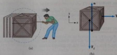
Figure 4.9 (a) A crate being pulled to the right on a frictionless surface. (b) The free-body diagram that represents the external forces on the crate.
