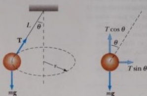
Figure 5.7 (Example 5.4) The conical pendulum and its free-body diagram.
