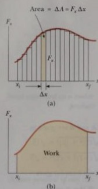
Figure 6.6 (a) The work done by the force F_x for the small displacement \Delta x is F_x \Delta x , which equals the area of the shaded rectangle. The total work done for the displacement from x_i to x_f is approximately equal to the sum of the areas of all the rectangles. (b) The work done by the variable force F_x as the particle moves from x_i to x_f is exactly equal to the area under this curve.
