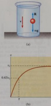
Figure 5.12 (a) A small sphere falling through a viscous fluid. (b) The speed-time graph for an object falling through a viscous medium. The object reaches a maximum, or terminal speed v_t , and \tau is the time it takes to reach 0.63v_t .
