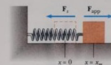
Figure 6.9 A block being pulled from x = 0 to x = x_m on a frictionless surface by a force F_{app} . If the process is carried out very slowly, the applied force is equal to and opposite the spring force at all times.
