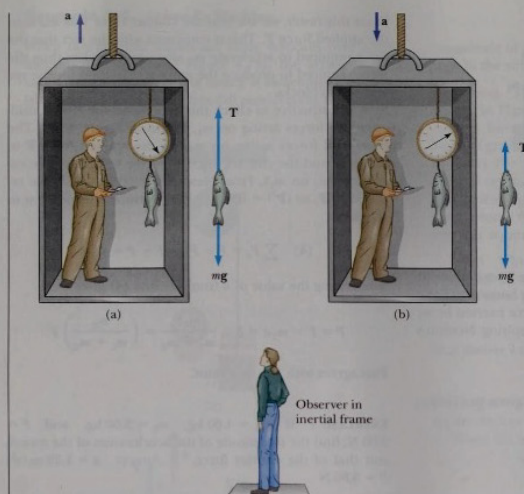
Figure 4.15 (Example 4.6). (a) When the elevator accelerates upward , the spring scale reads a value greater than the weight. (b) When the elevator accelerates downward , the spring scale reads a value less than the weight.
