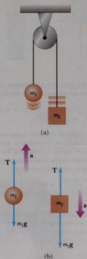
Figure 4.13 (Example 4.4) Atwood's machine. (a) Two masses connected by a light string over a frictionless pulley. (b) Free-body diagrams for m_1 and m_2 .
