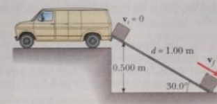
Figure 7.10 (Example 7.3) A crate slides down a ramp under the influence of gravity. The potential energy of the system decreases, and the kinetic energy of the crate increases.
