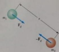
Figure 5.16 Two particles of masses m_1 and m_2 attract each other with a force of magnitude Gm_1m_2/r^2 .
