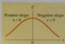
Figure 7.17 A plot of U versus x for a particle that has a position of unstable equilibrium, located at x = 0 . For any finite displacement of the particle, the force on the particle is directed away from x = 0 .
