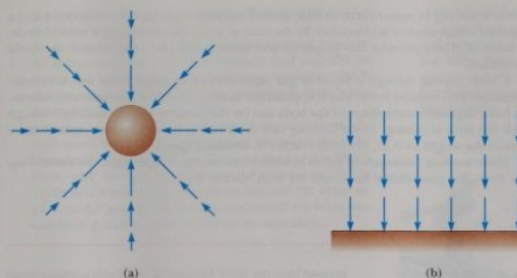
Figure 5.19 (a) The gravitational field vectors in the vicinity of a uniform spherical mass vary in both direction and magnitude. (b) The gravitational field vectors in a small region near the Earth's surface are uniform—that is, they match in both direction and magnitude.
