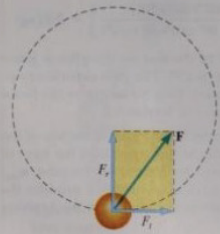
Figure 5.10 When the force acting on a particle moving in a circular path has a tangential component F_t , its speed changes. The total force on the particle also has a component F_r directed toward the center of the circular path. Thus, total force is \mathbf{F} = \mathbf{F}_r + \mathbf{F}_t .
