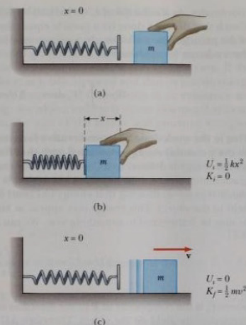
Figure 7.3 A block of mass m on a frictionless horizontal surface is pushed against a spring and then released. If x is the compression in the spring as in (b), the elastic potential energy stored in the spring is \frac{1}{2}kx^2 . This energy is transferred to the block in the form of kinetic energy as in (c).
