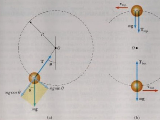
Figure 5.11 (Example 5.7) (a) Forces acting on a mass m connected to a string of length R and rotating in a vertical circle centered at O . (b) Forces acting on m when it is at the top and bottom of the circle. Note that the tension at the bottom is a maximum and the tension at the top is a minimum.
