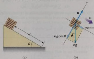
Figure 4.12 (Example 4.3) (a) A crate sliding down a frictionless incline. (b) Free-body diagram for the crate. Note that the magnitude of its acceleration along the incline is g \sin \theta .
