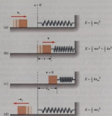
Figure 7.12 (Example 7.12) A block sliding on a smooth, horizontal surface collides with a light spring. (a) Initially the mechanical energy is all kinetic energy. (b) The mechanical energy is the sum of the kinetic energy of the block and the elastic potential energy in the spring. (c) The energy is entirely potential energy. (d) The energy is converted back to the kinetic energy of the block. The total energy remains constant throughout the motion.
