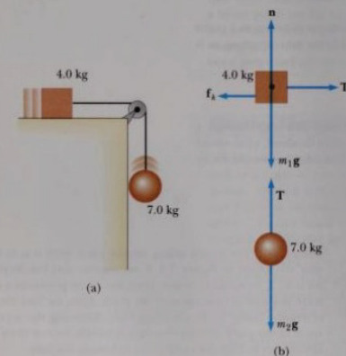
Figure 5.4 (Example 5.2) (a) Two objects connected by a light string that passes over a frictionless pulley. (b) Free-body diagrams for the objects.
