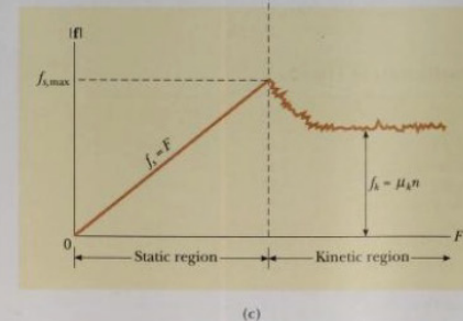
Figure 5.1 The force of friction, \mathbf{f} , between a block and a rough surface is opposite the applied force, \mathbf{F} . (a) The force of static friction equals the applied force. (b) When the applied force exceeds the force of kinetic friction, the block accelerates to the right. (c) A graph of the magnitude of the frictional force versus the applied force. Note that f_{s, \max} > f_k .
