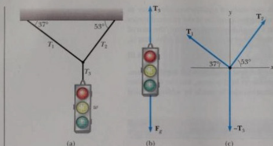
Figure 4.10 (Example 4.2) (a) A traffic light suspended by cables. (b) Free-body diagram for the traffic light. (c) Free-body diagram for the knot in the cable.
