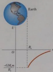
Figure 7.14 Graph of the gravitational potential energy, U_g , versus r for a particle above the Earth's surface. The potential energy of the system goes to zero as r approaches \infty .
