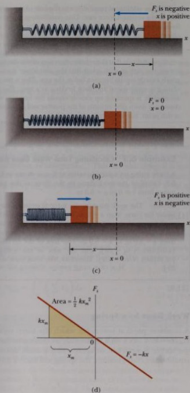
Figure 6.8 The force exerted by a spring on a block varies with the block's displacement from the equilibrium position x = 0 . (a) When x is positive (stretched spring), the spring force is to the left. (b) When x is zero, the spring force is zero (natural length of the spring). (c) When x is negative (compressed spring), the spring force is to the right. (d) Graph of F_s versus x for the mass-spring system. The work done by the spring force as the block moves from -x_m to 0 is the area of the shaded triangle, \frac{1}{2} kx_m^2 .
