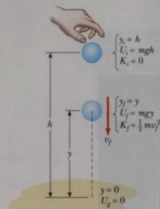
Figure 7.7 (Example 7.1) A ball is dropped from a height h above the ground. Initially, the total energy is gravitational potential energy, equal to mgh relative to the ground. At the elevation y , the total energy is the sum of kinetic and potential energies.
