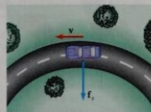
Figure 5.8 (Example 5.5) The force of static friction directed toward the center of the arc keeps the car moving in a circle.
