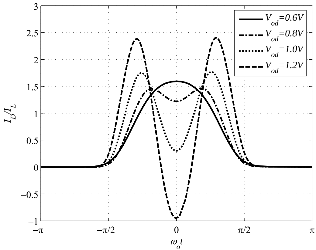
Figure 3.25: I_D/I_L vs. \omega_o t for the tail- and top-biased N/PMOS topologies (Figs. 3.24 (a) and (b)) for different swings ( V_{od} ) at 100MHz.
