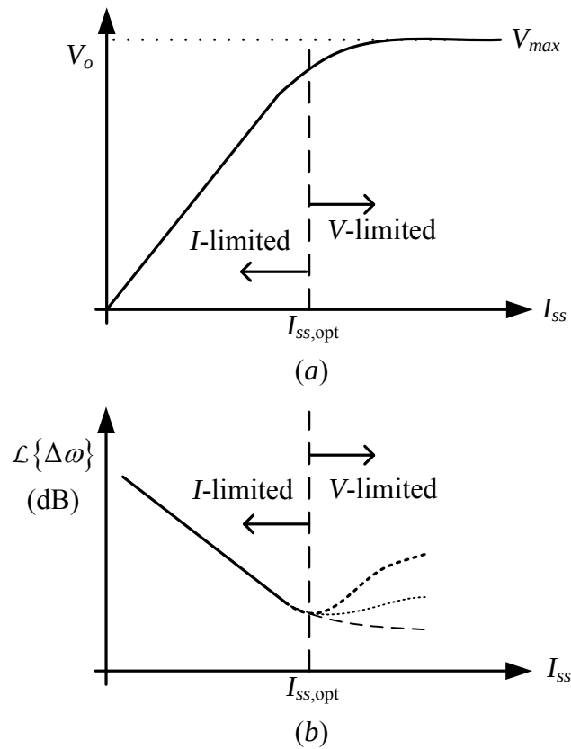
Figure 4.3: (a) V_o vs. I_{ss} and (b) \mathcal{L}\{\Delta\omega\} vs. I_{ss} , across current- and voltage-limited regimes.
