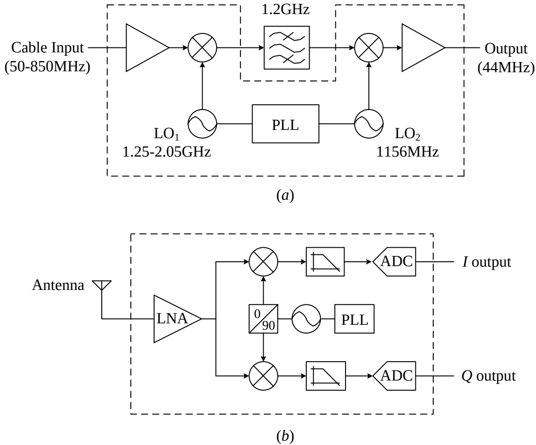
Figure 1.2: Two common applications of PLLs: (a) a cable TV tuner based on a dual-conversion architecture, (b) a wireless receiver based on a direct-conversion architecture.
