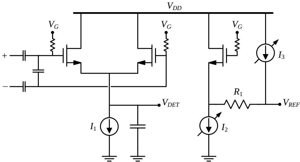
Figure 5.6: Simplified schematic of peak detector.
