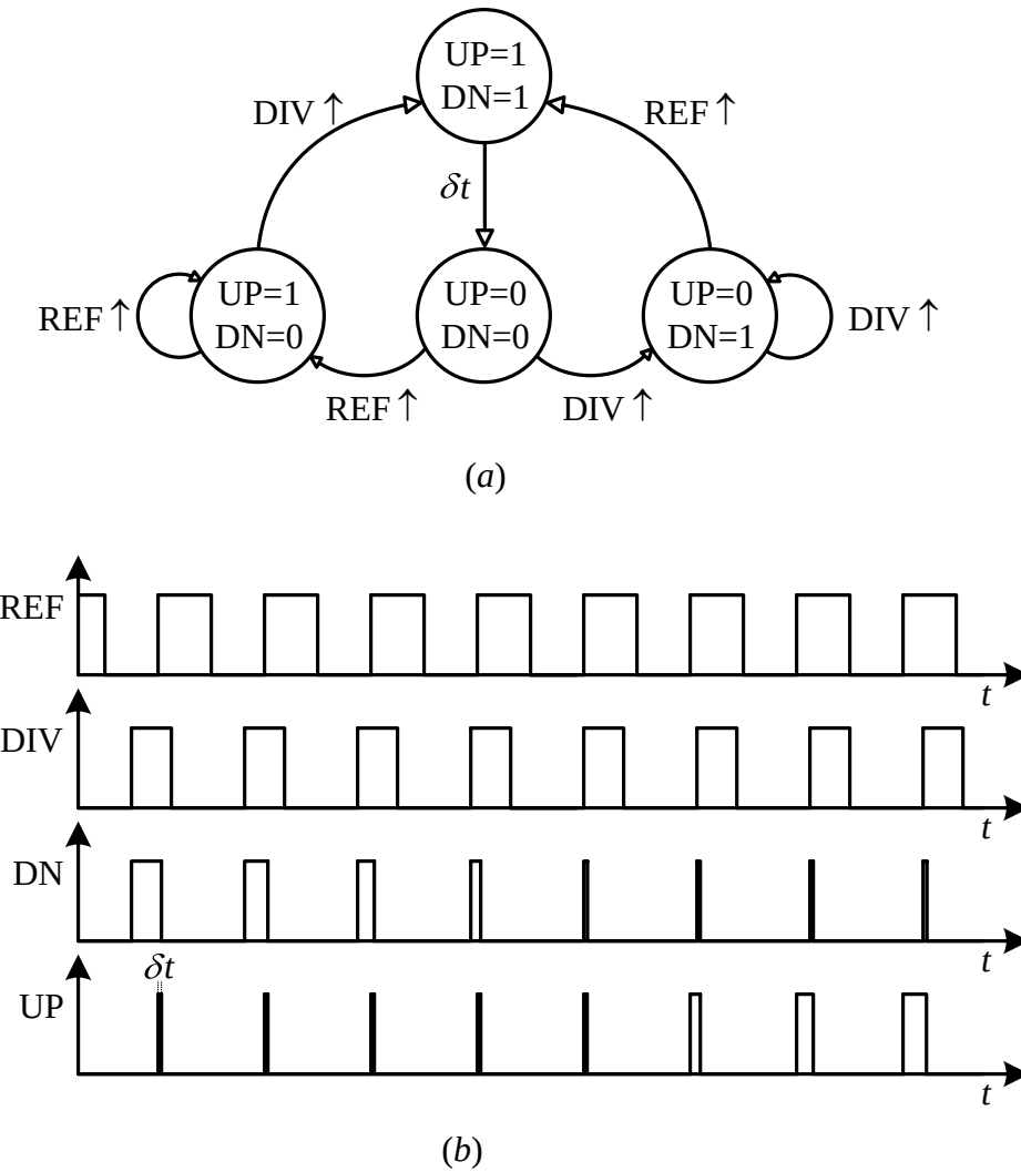
Figure 2.11: (a) Tri-state PFD transition state diagram and (b) signal waveforms.
