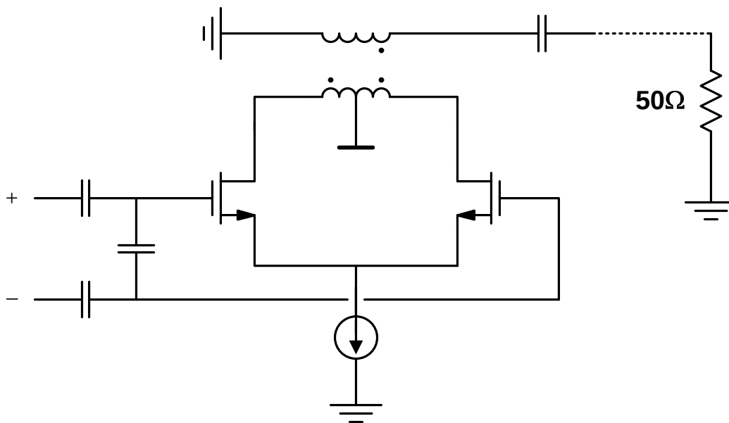
Figure 5.5: Simplified schematic of VCO output buffer.
