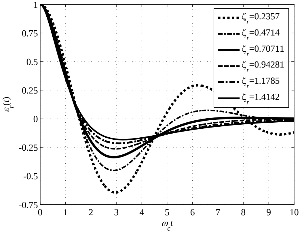
Figure 2.19: Unit step error response \varepsilon_r(t) vs. \omega_c t of third-order PLL with \zeta_r = (r-1)/2 , where r = \omega_c/\omega_z = \omega_1/\omega_c .
