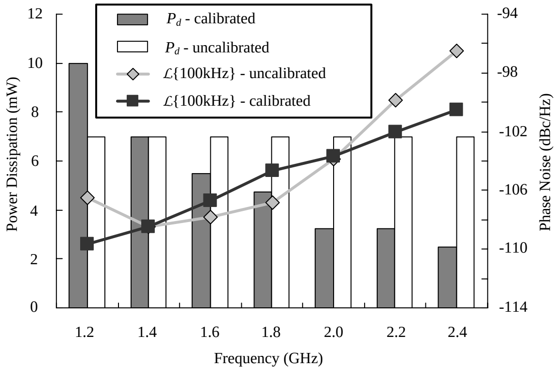
Figure 5.14: Measured phase noise at 100 kHz offset and core power consumption vs. frequency for calibrated and uncalibrated cases.
