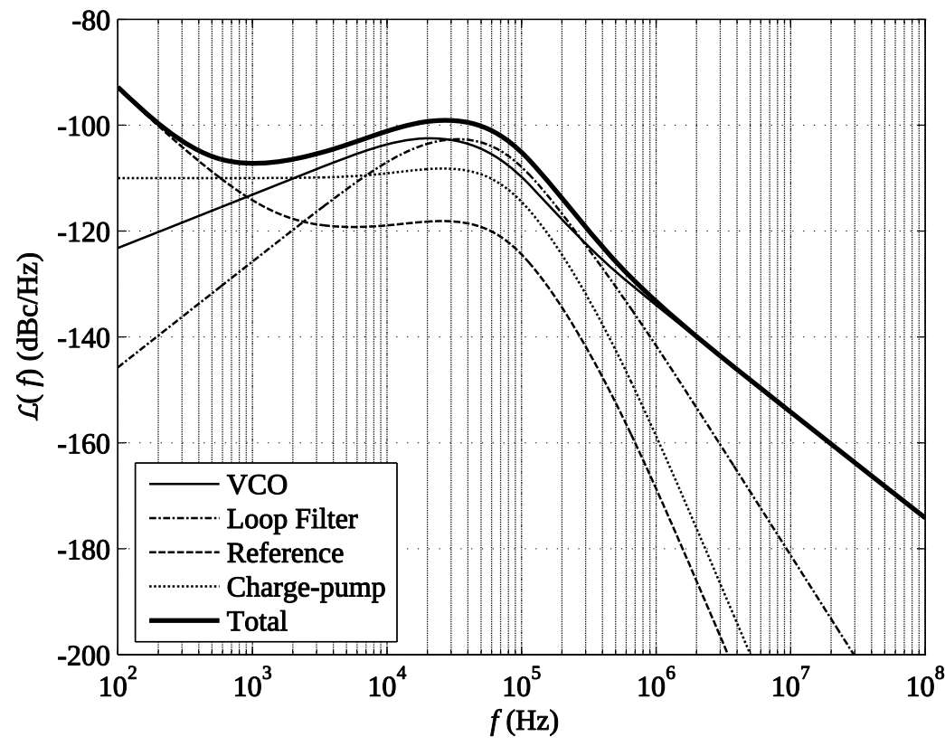
Figure 2.23: Typical PLL noise.
