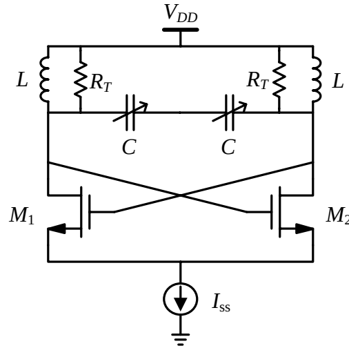
Figure 4.2: Differential cross-coupled NMOS tail-biased LC VCO.
