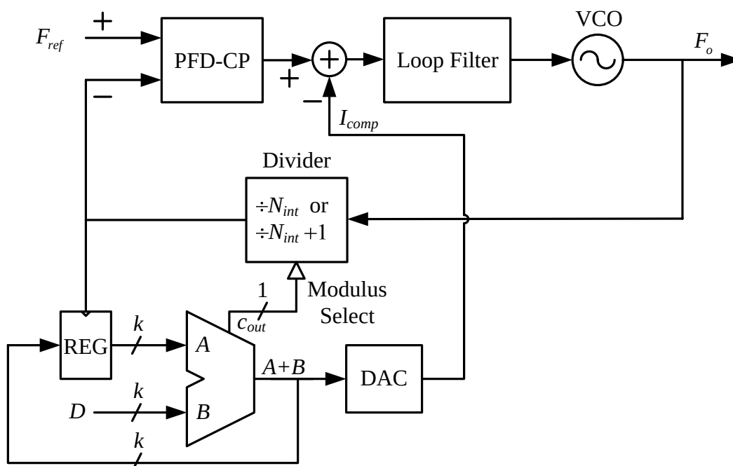
Figure 2.26: Fractional-N PLL with phase error compensation.
