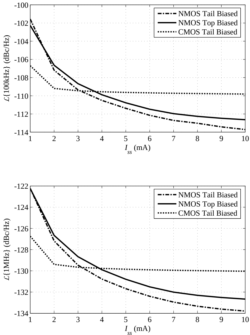
Figure 3.32: Simulated Phase Noise at 0.1- and 1-MHz offsets, for each of the three basic configurations (Fig. 3.18), resized at each value of I_{ss} to keep g_m constant.
