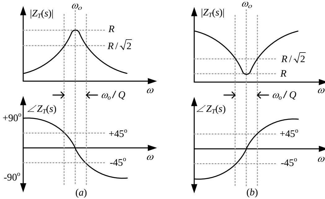
Figure 3.3: Magnitude and phase of LC tank impedance for Parallel (a) and Series (b) configurations.
