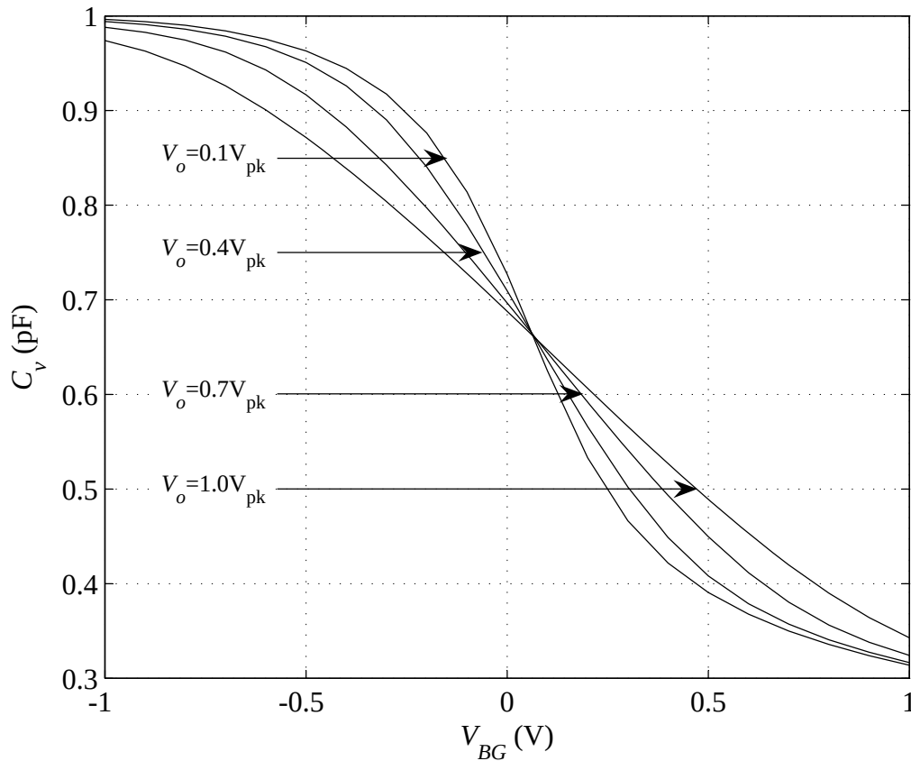
Figure 3.12: C - V characteristics for different V_o .
