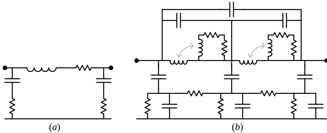
Figure 3.9: On-chip inductor models (a) pi-equivalent, (b) wideband lumped equivalent.
