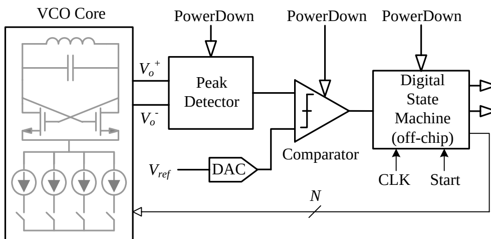
Figure 4.6: Proposed calibration-based amplitude control scheme.
