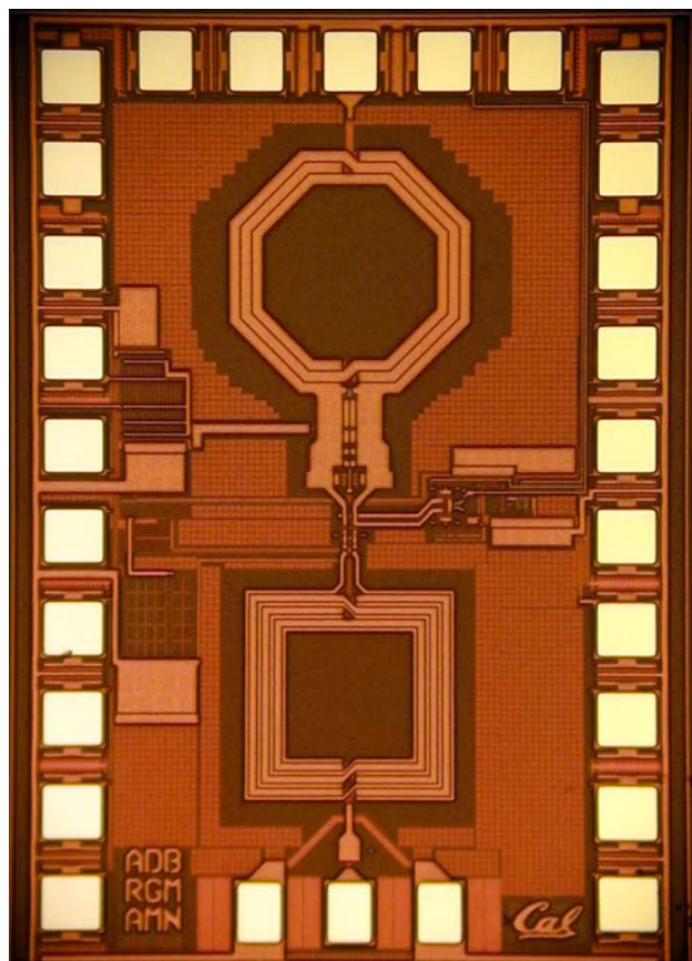
Figure 5.9: Die photograph.
