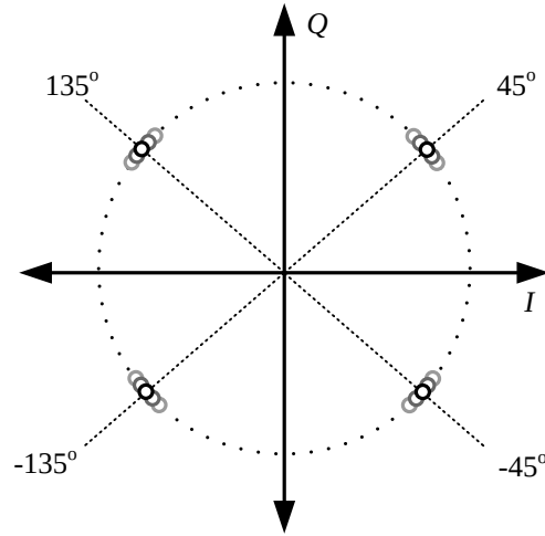
Figure 2.5: QPSK symbol constellation showing rotational error due to finite phase noise \phi(t) on the LO.
