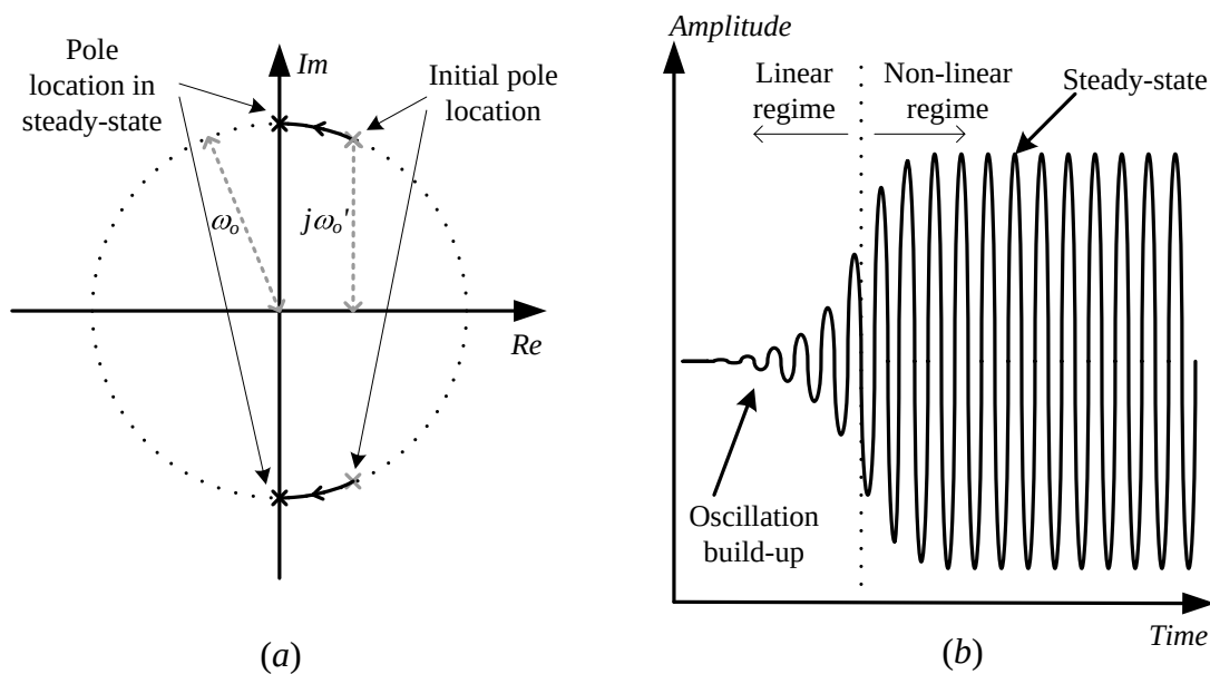
Figure 3.16: (a) Root locus of LC oscillator. (b) Output waveform of LC oscillator.
