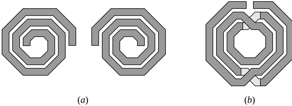
Figure 3.5: A pair of single-ended inductors (a) and a differential inductor (b) with similar total inductance.
