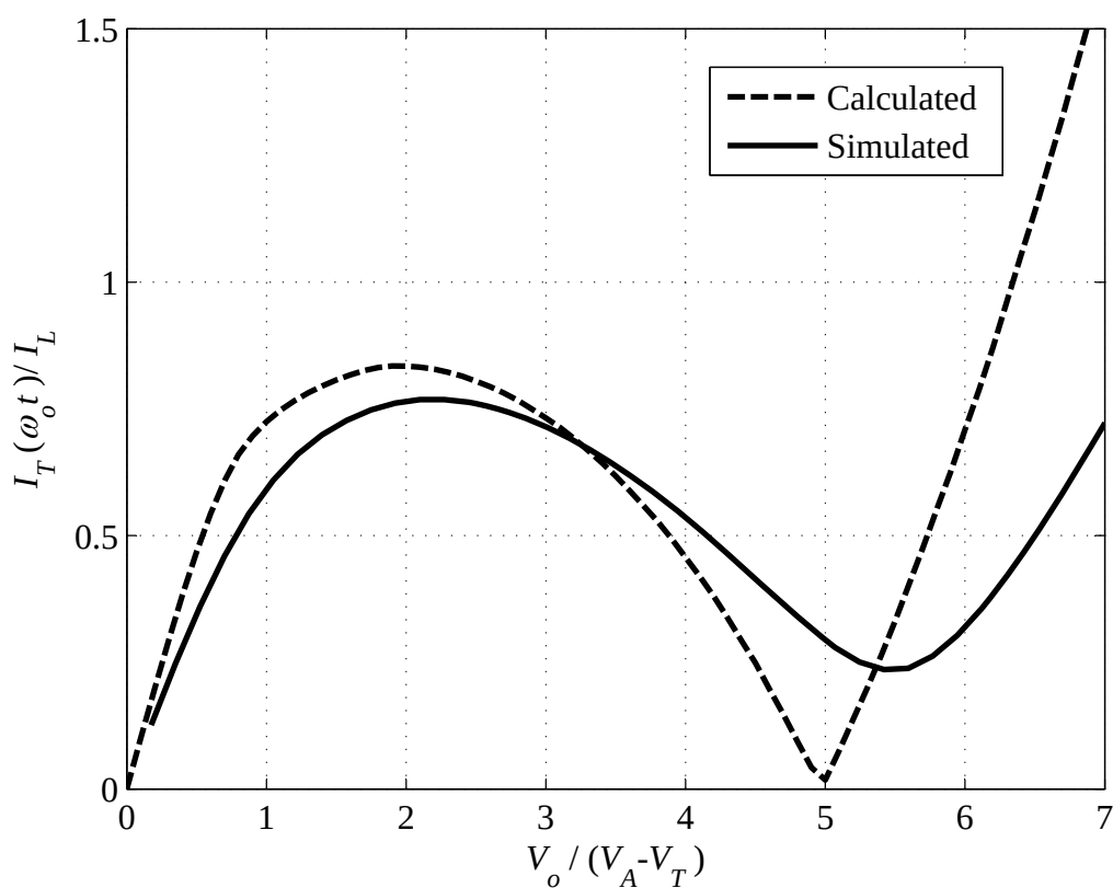
Figure 3.31: Calculated and simulated |I_T(\omega_o)|/I_L vs. V_o/(V_A - V_T) for the NMOS tail-biased configuration shown in Figs. 3.18(a), for V_T/(V_A - V_T) \approx 3 , where V_T = 0.45\text{V} and V_A \approx 0.6\text{V} .
