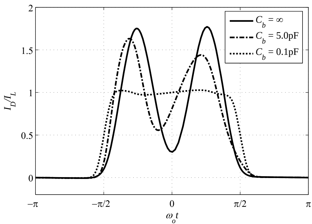
Figure 3.22: I_D/I_L vs. \omega_o t for the tail- and top-biased N/PMOS topologies (Figs. 3.18 (a) and (c)) for different values of C_b at 100MHz.
