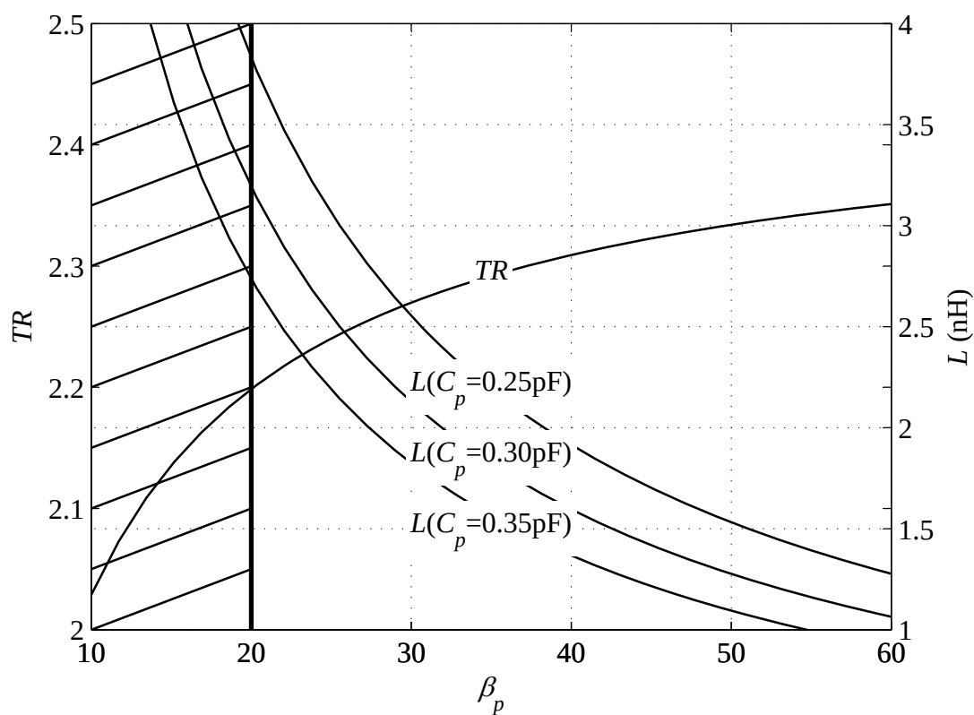
Figure 5.3: TR and L vs. \beta_p for \beta_a = 7 , \beta_v = 2.5 , n = 4 , k = 1.1 , and f_{o,\min} = 1.10\text{GHz} .
