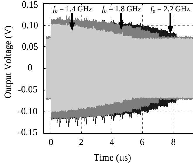
Figure 5.13: Measured amplitude calibration runs at 1.4, 1.8 and 2.2GHz.
