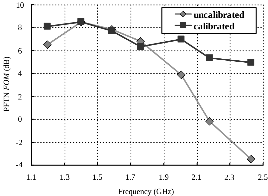
Figure 5.15: FOM vs. frequency for calibrated and uncalibrated cases.
