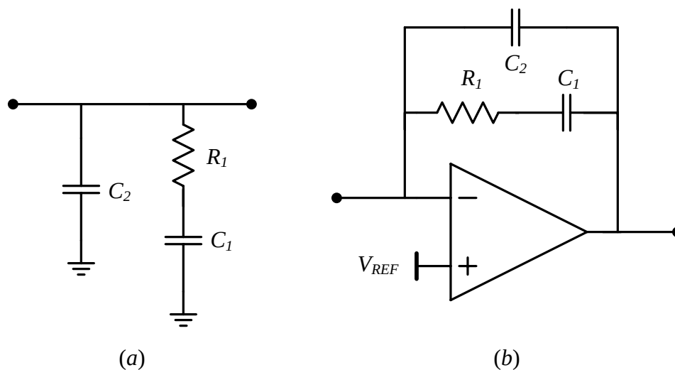
Figure 2.14: (a) second-order passive loop filter. (b) second-order active loop filter.
