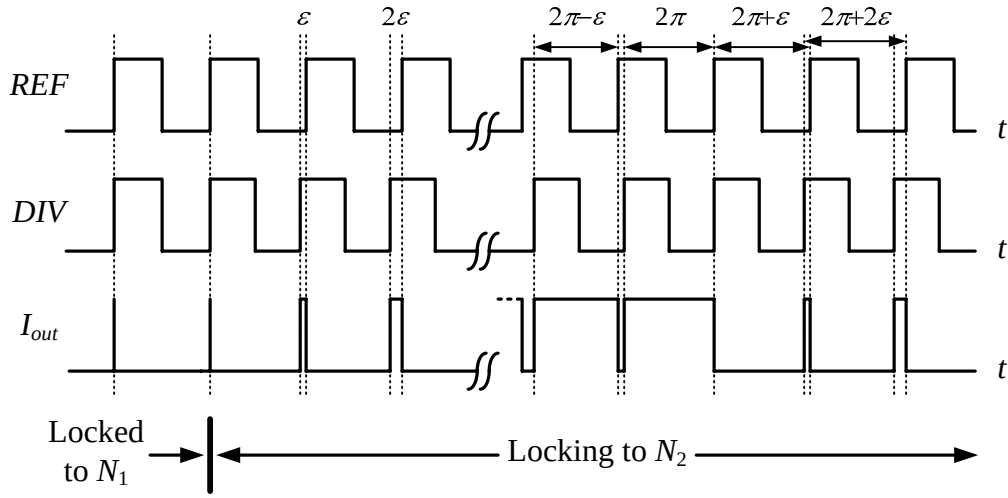
Figure 2.20: Timing diagram of REF and DIV (inputs to the PFD) and I_{out} (charge-pump output current) during cycle-slip, where \omega_c is assumed to be infinitely large.
