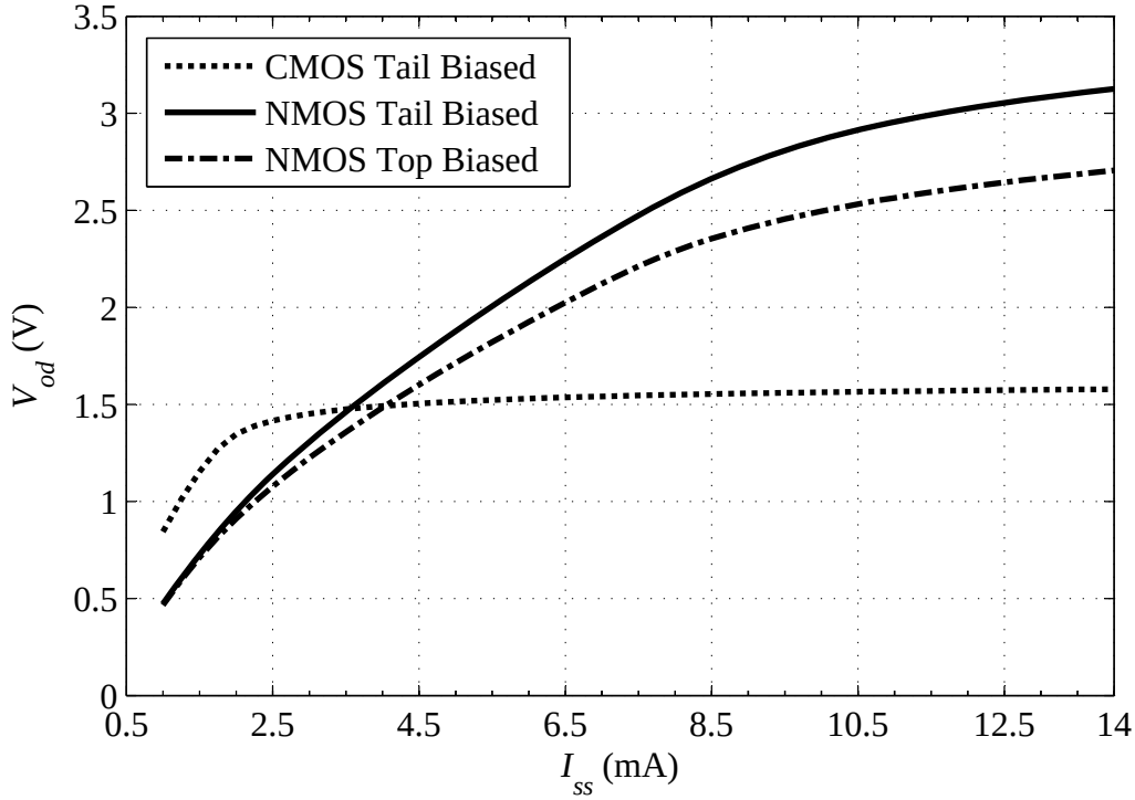
Figure 3.21: Simulated differential output swing for reference designs of each of the three basic configurations (Fig. 3.18(a)-(c)).
