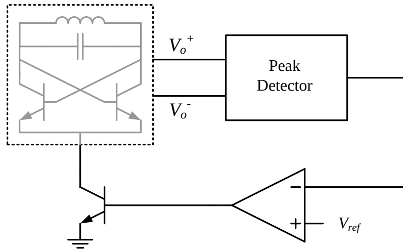
Figure 4.5: Conventional continuous-time automatic amplitude control (AAC) loop.
