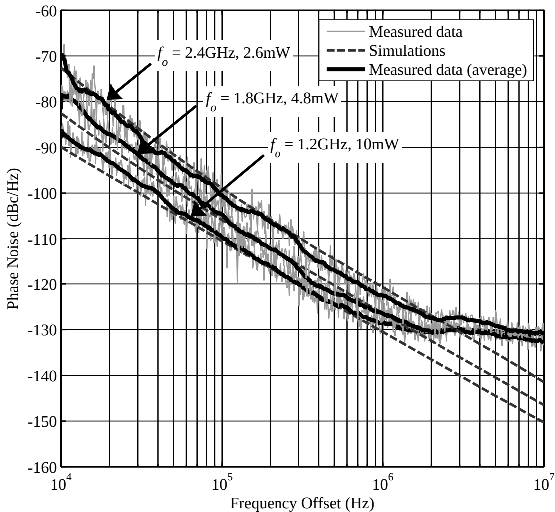
Figure 5.11: Phase Noise at 1.2, 1.8, and 2.4GHz for a core power consumption of 10, 4.8, and 2.6mW, respectively.
