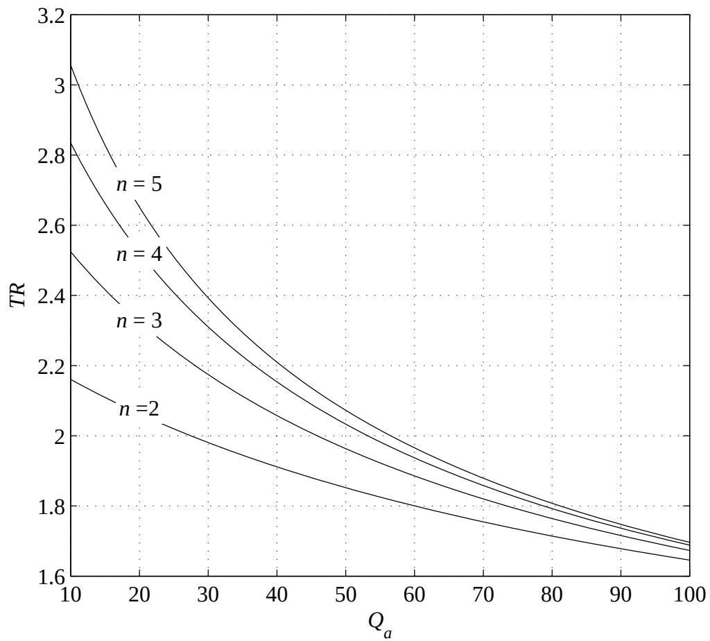
Figure 5.2: TR vs. Q_a for \beta_v = 2.5 , \beta_p = 20 , k = 1.1 , and R_{on}C_d = 300 \times 10^{-15} (1/rad).
