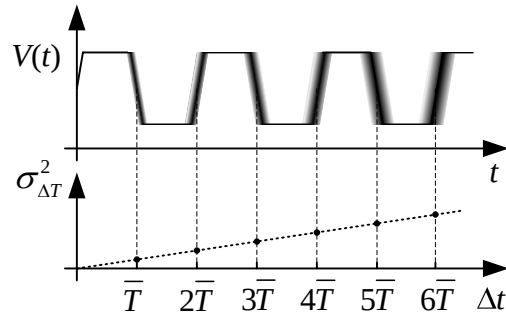
Figure 2.6: Time waveform showing jitter with statistics underneath.
