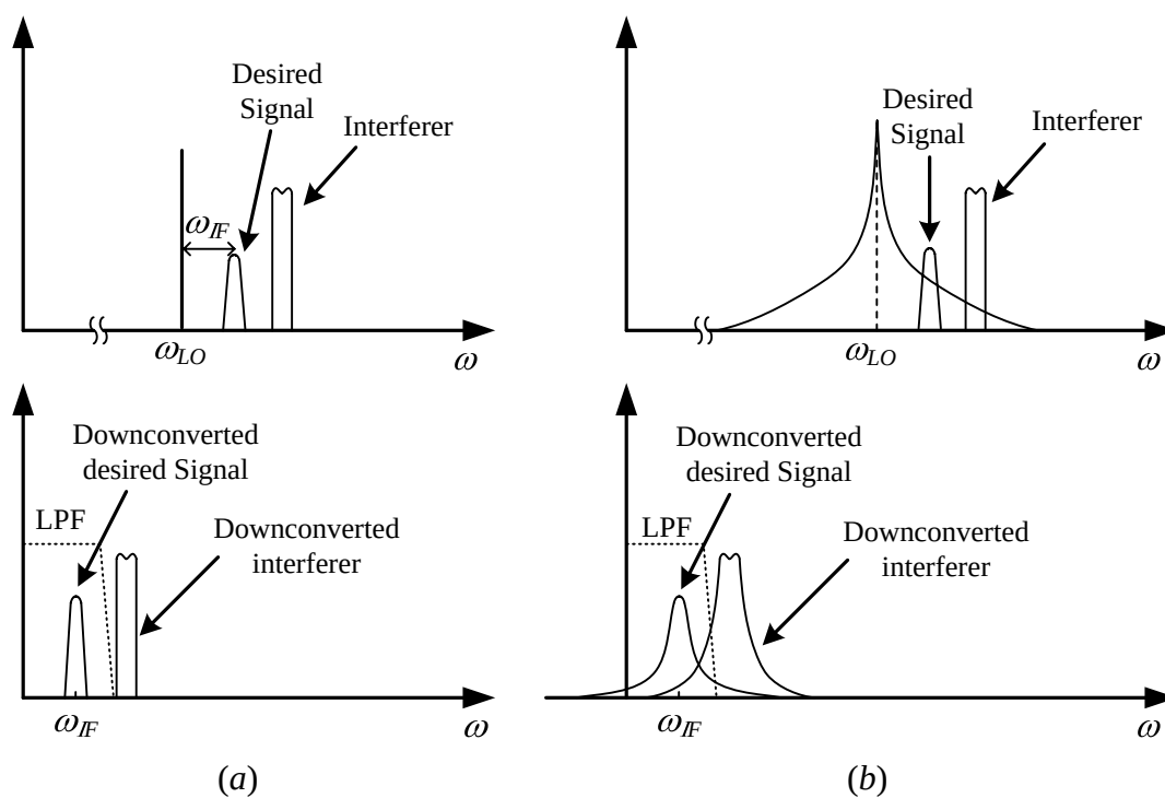
Figure 2.4: SNR degradation due to reciprocal mixing of unwanted signal.
