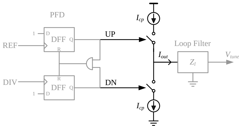
Figure 2.12: Simplified schematic of a charge-pump driven by a PFD and loaded by an arbitrary loop filter.
