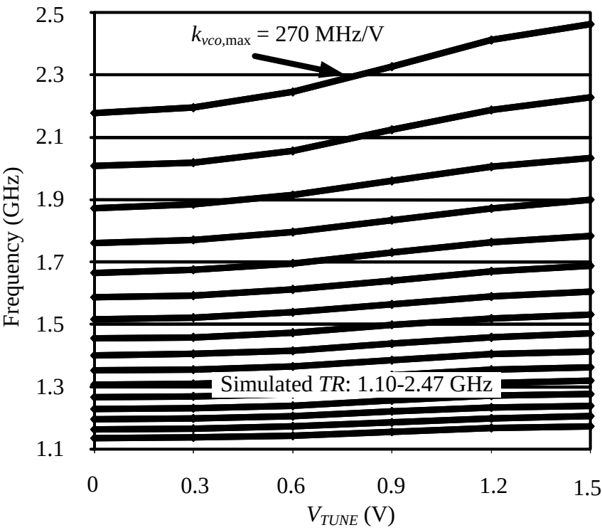
Figure 5.12: Measured frequency tuning range.
