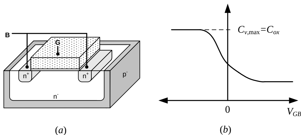
Figure 3.11: MOS varactor. (a) Physical structure. (b) C - V characteristic.
