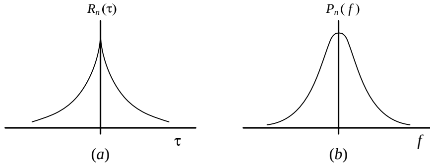
Figure 2.2: (a) R_n(\tau) and (b) P_n(f) of the thermal noise from a generic RC lowpass filter.
