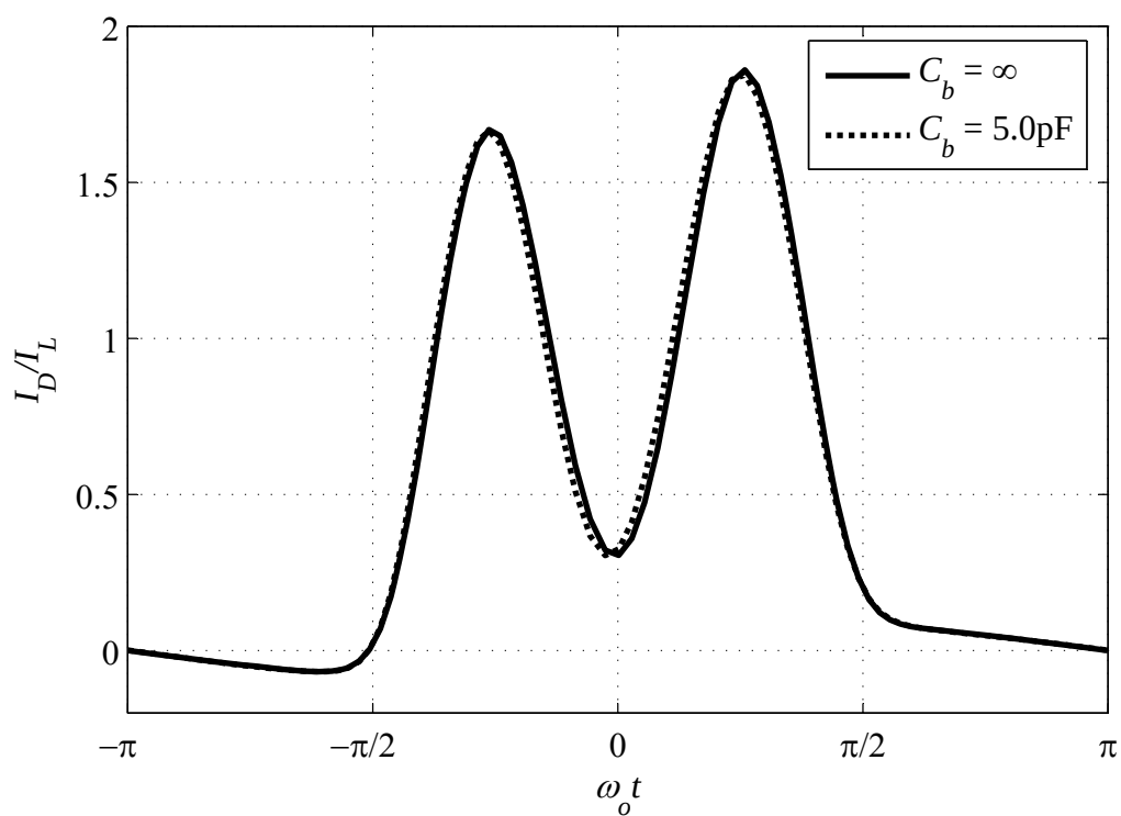
Figure 3.23: I_D/I_L vs. \omega_o t for the tail- and top-biased N/PMOS topologies (Figs. 3.18 (a) and (c)) for different values of C_b at 1GHz.
