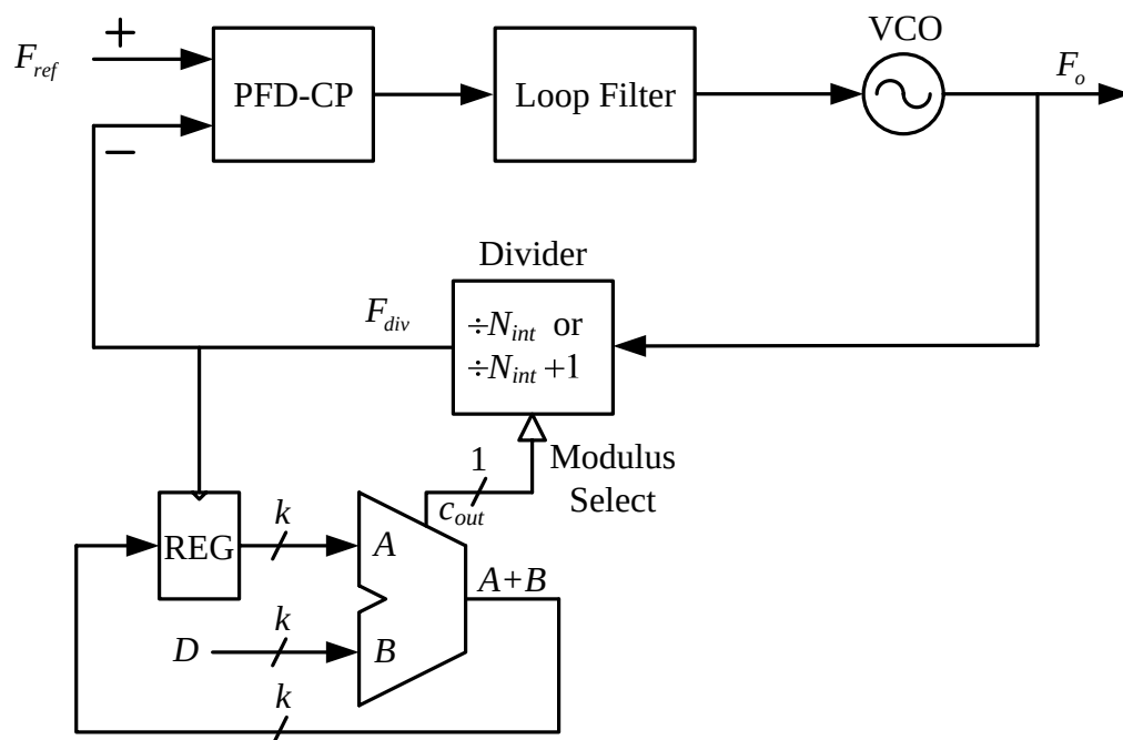
Figure 2.24: Basic Fractional-N PLL showing digital k -bit accumulator.
