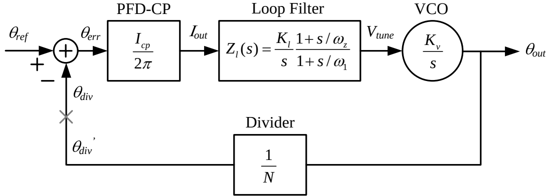
Figure 2.15: Linear model of third-order PLL.
