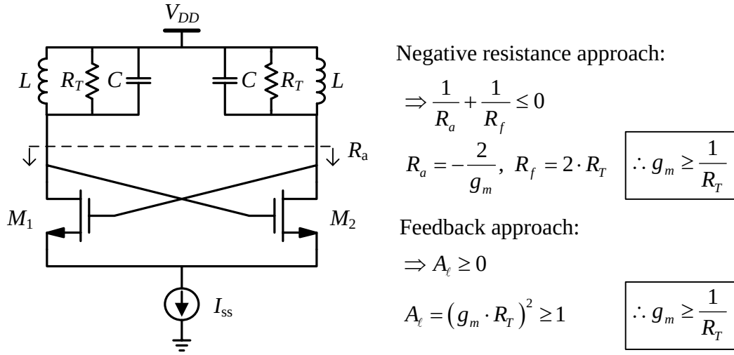
Figure 3.15: Start-up requirements of an NMOS cross-coupled LC VCO based on two different methods, the negative resistance approach and the feedback approach.
