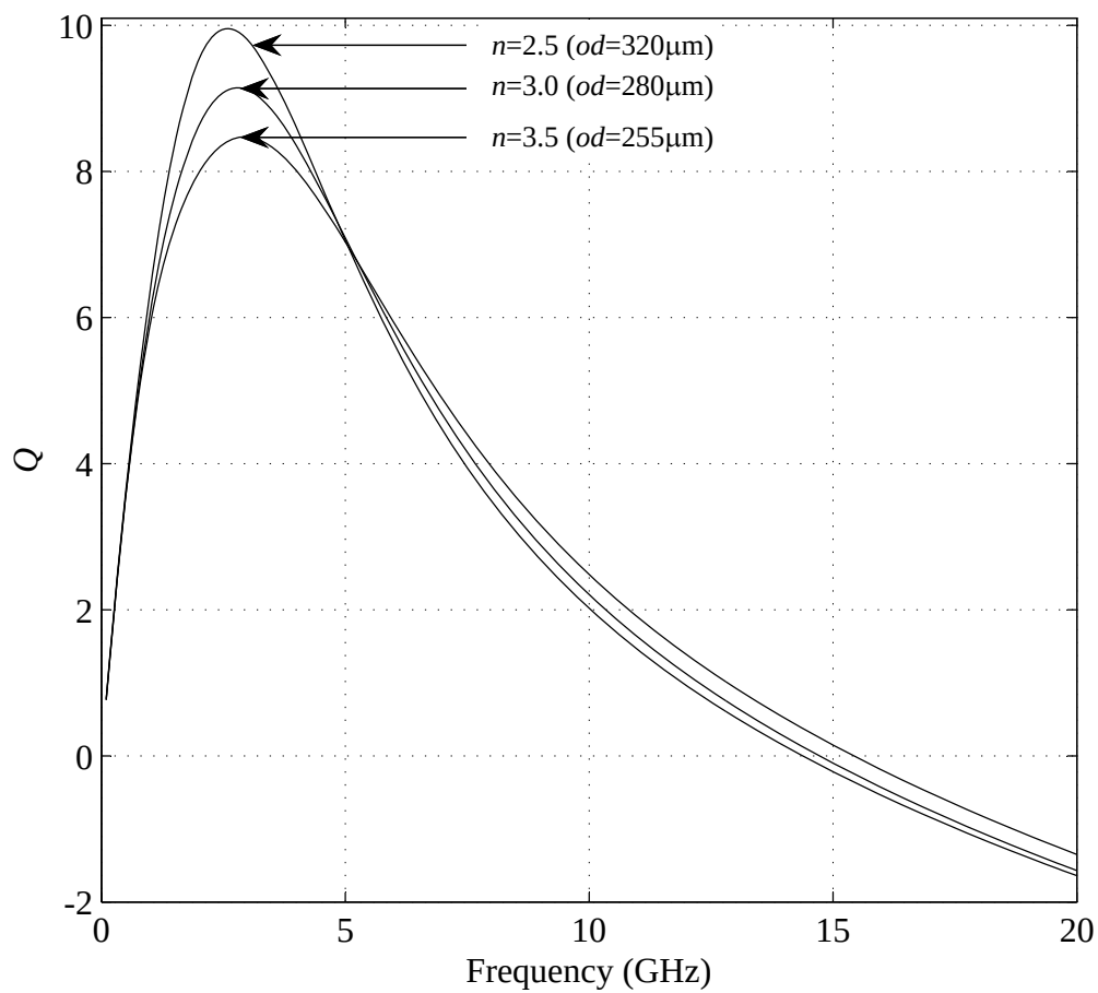
Figure 3.8: Q vs. f of 3nH inductor for different number of turns ( n ), and w = 15\mu\text{m} , s = 4.5\mu\text{m} .
