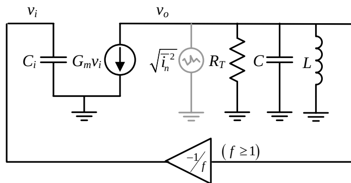
Figure 4.4: Generic LC oscillator with equivalent noise source \overline{i_n^2} .
