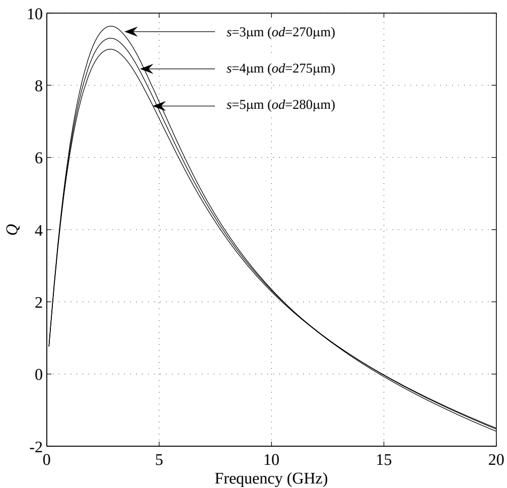
Figure 3.7: Q vs. f of 3nH inductor for different turn-turn spacing ( s ), and n = 3 , w = 15\mu\text{m} .
