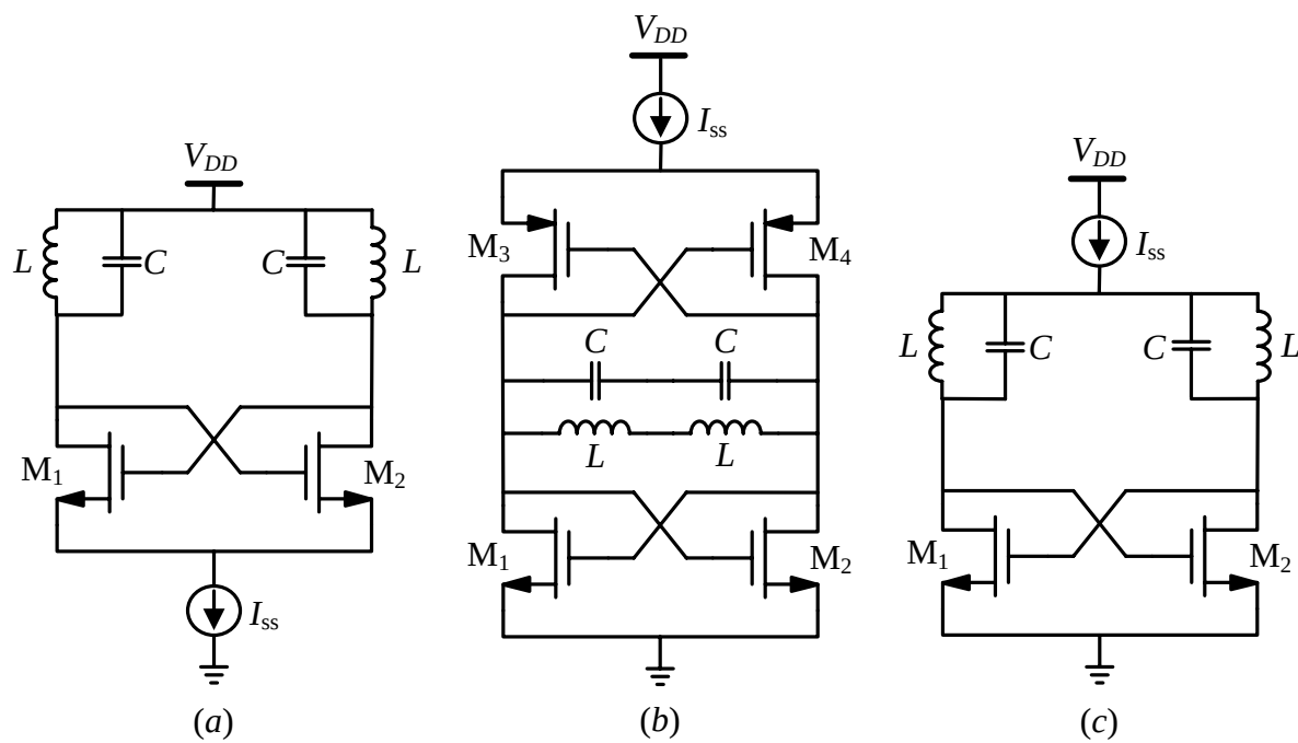
Figure 3.18: LC VCO topologies: (a) tail-biased cross-coupled, (b) complementary cross-coupled, (c) top-biased cross-coupled.
