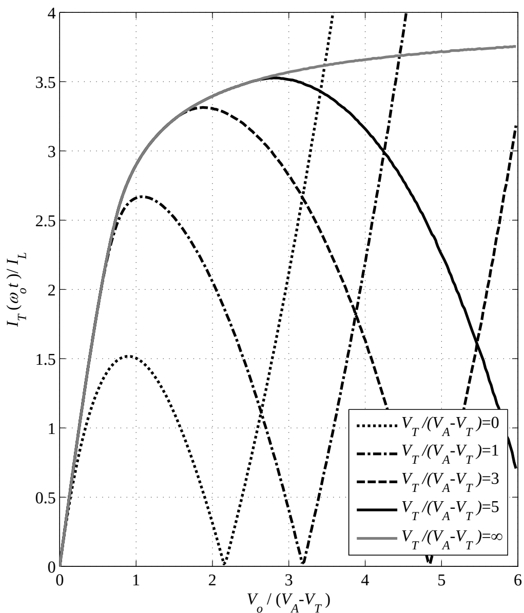
Figure 3.30: |I_T(\omega_o)|/I_L vs. V_o/(V_A - V_T) for the CMOS configuration shown in Figs. 3.27, for different values of V_T/(V_A - V_T) .
