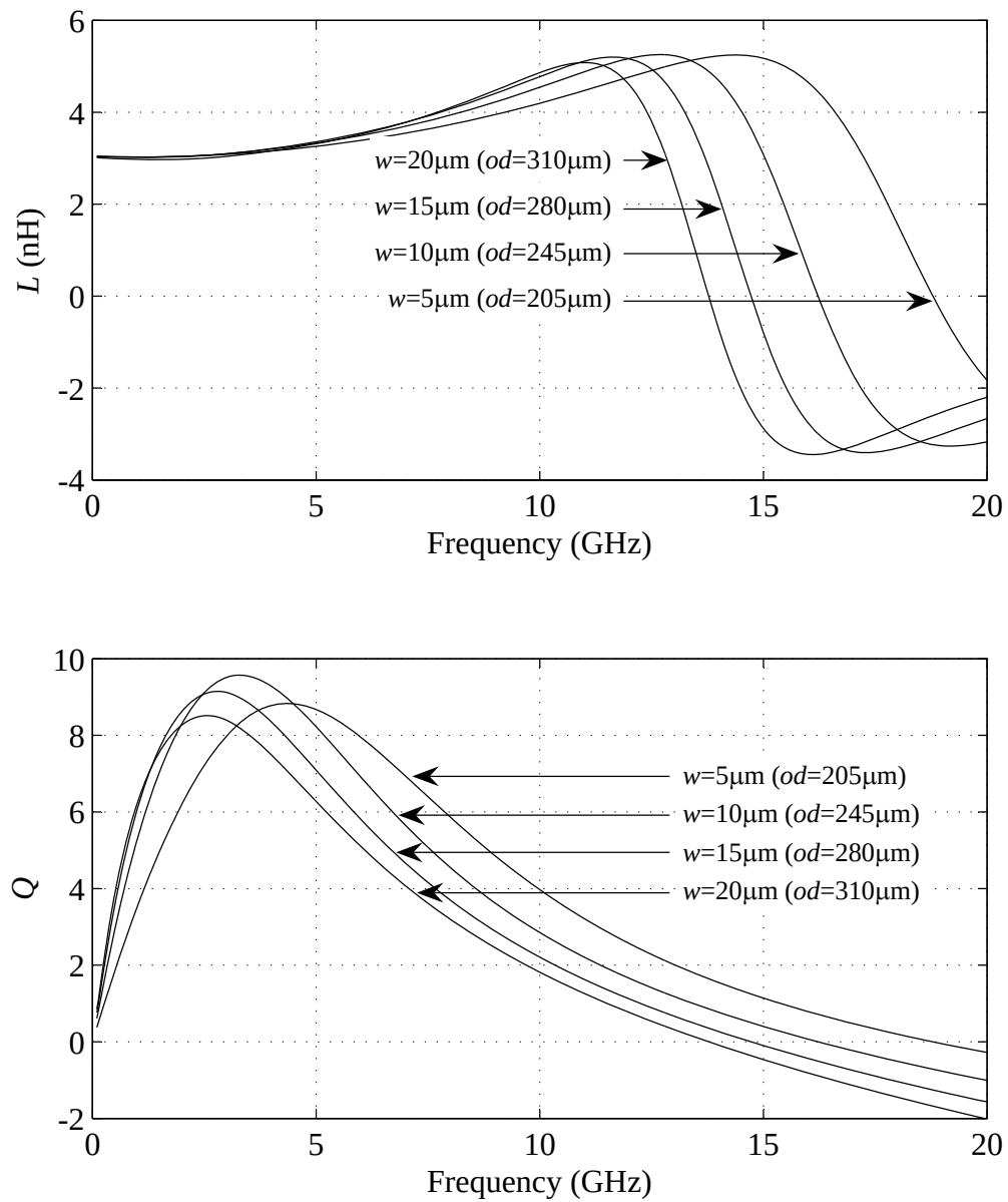
Figure 3.6: Q and L vs. f of 3nH inductor for different widths ( w ), and n = 3 , s = 4.5\mu\text{m} .
