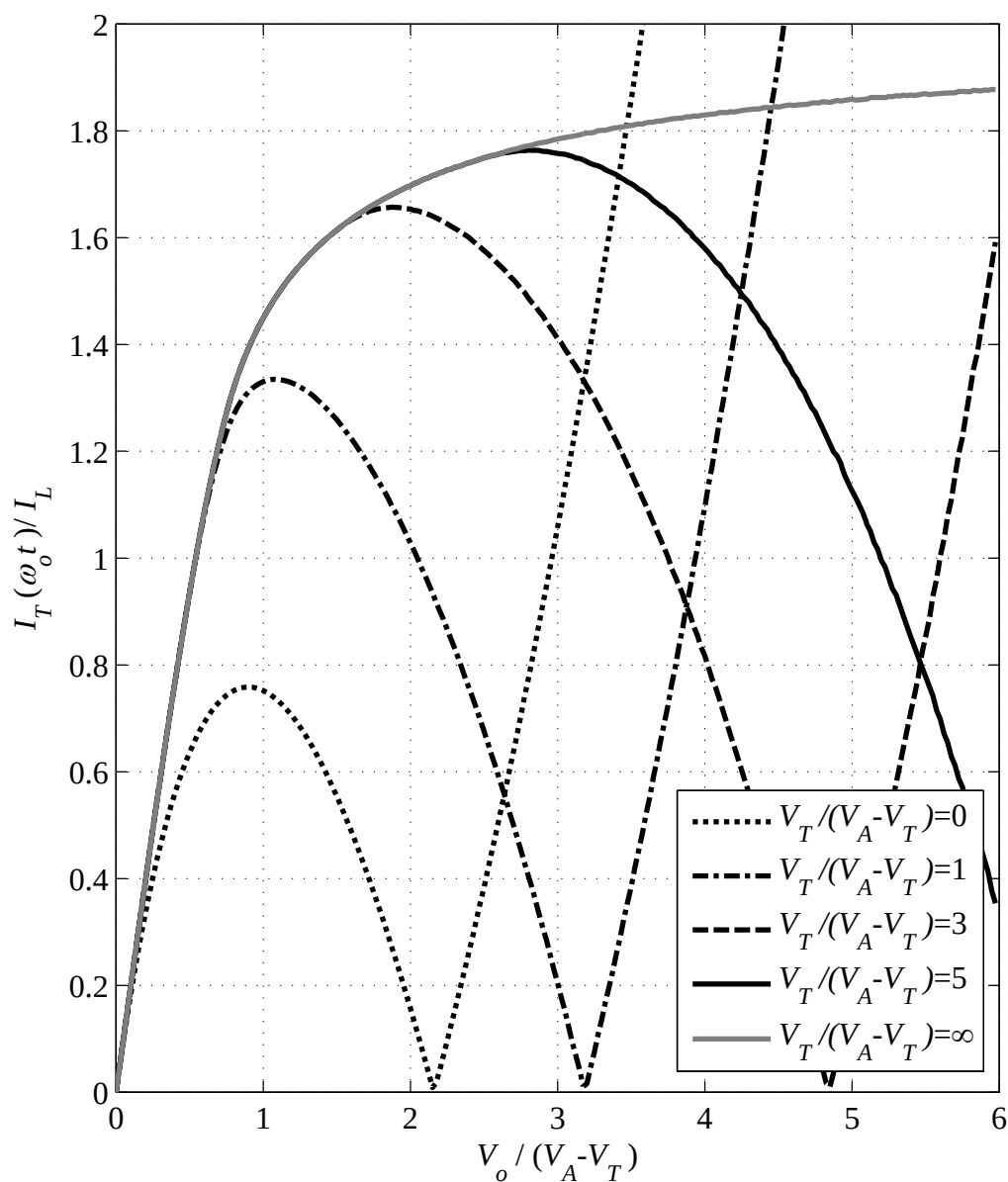
Figure 3.29: |I_T(\omega_o)|/I_L vs. V_o/(V_A - V_T) for the N/PMOS configurations shown in Fig. 3.24, for different values of V_T/(V_A - V_T) .
