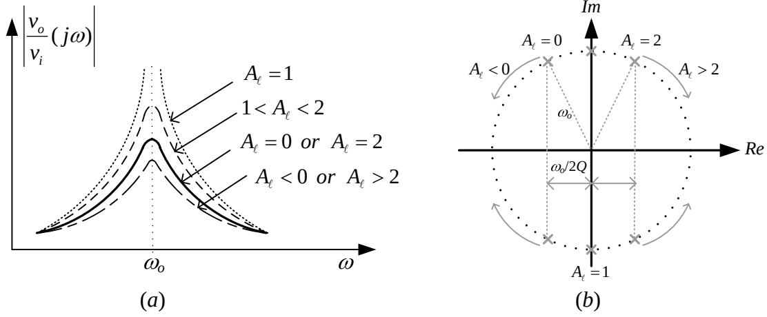
Figure 3.14: (a) Magnitude of transfer function for different values of loop gain. (b) Root locus of transfer function for different values of loop gain.
