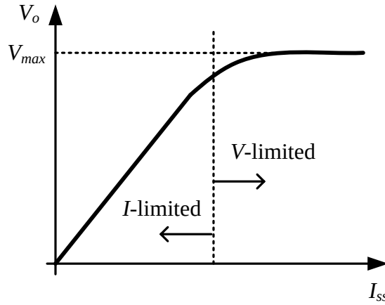
Figure 3.19: Steady-state voltage amplitude vs. I_{ss} for typical LC VCO.
