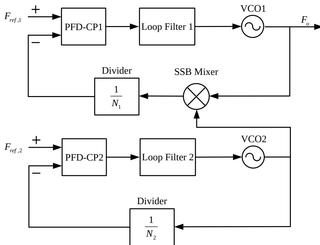
Figure 2.28: Example of a dual-loop PLL.
