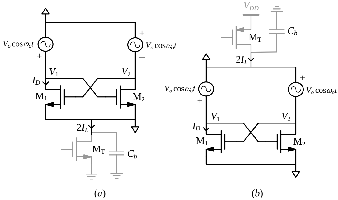
Figure 3.24: (a) Tail- and (b) top-biased NMOS configurations with current source AC shorted.
