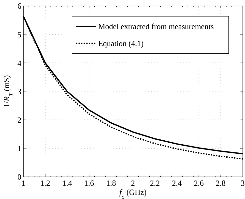
Figure 4.1: 1/R_T vs. f_o of typical LC tank obtained using a physical inductor model compared to that obtained using (4.1).
