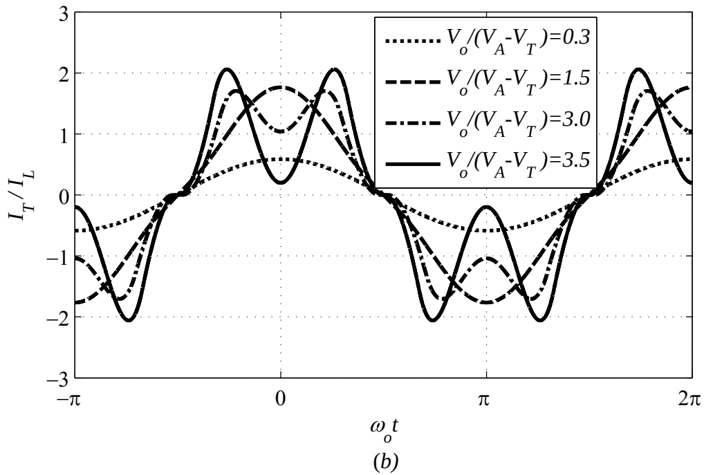
Figure 3.28: I_T/I_L vs. \omega_o t for different values of V_o/(V_A - V_T) and V_T/(V_A - V_T) = 3.6 for N/PMOS (a) and CMOS (b) configurations.
