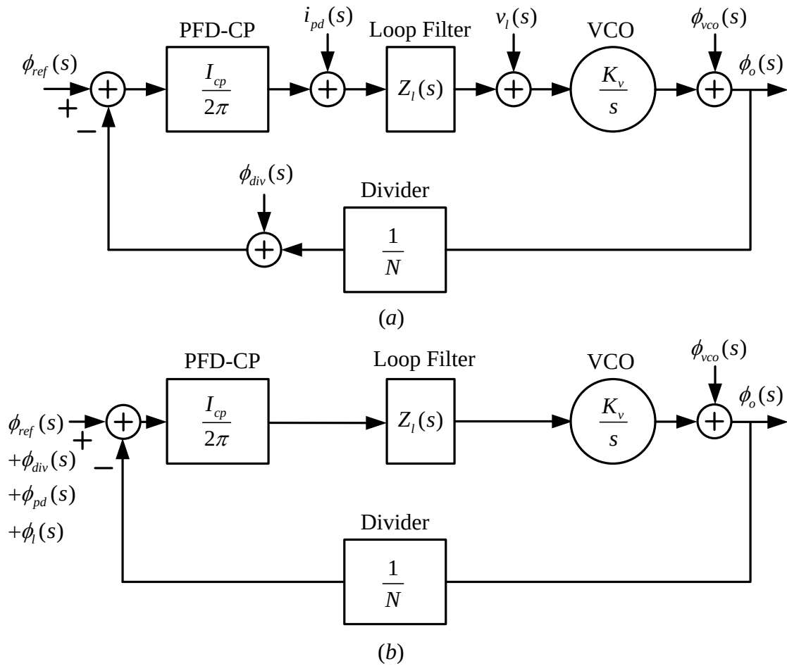
Figure 2.22: PLL linear noise model (a), and equivalent model with input- and output-referred noise sources (b).
