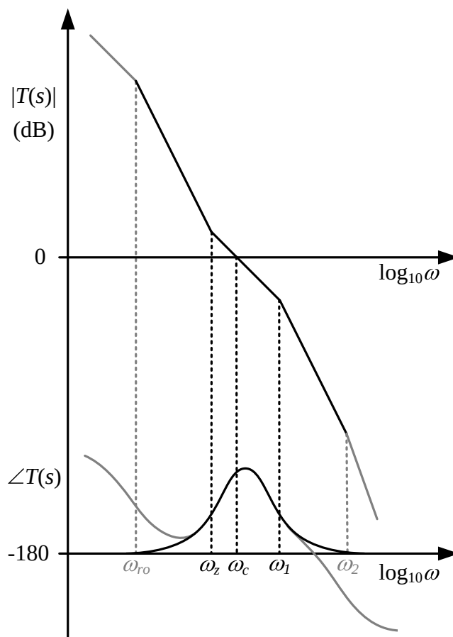
Figure 2.16: 20 \log_{10}(|T(s)|) and \angle T(s) for third-order PLL. The effects of parasitic poles from the finite output resistance of the charge-pump ( \omega_{ro} ) and an out-of-band RC filter ( \omega_2 ) are shown in grey.
