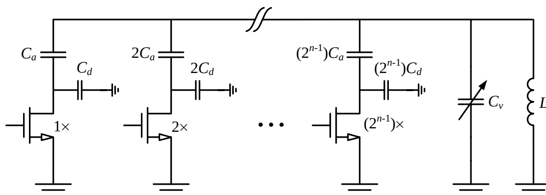
Figure 4.7: Generic binary-weighted band-switching LC tank configuration.
