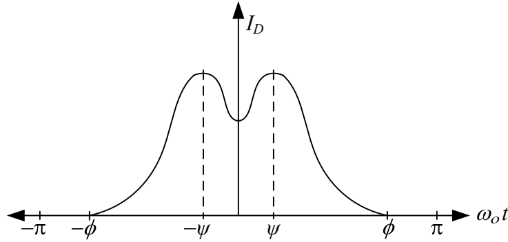
Figure 3.26: Typical I_D vs. \omega_o t waveform.
