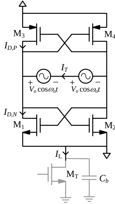
Figure 3.27: Tail-biased CMOS configuration of Fig. 3.18(b) with current source AC shorted.
