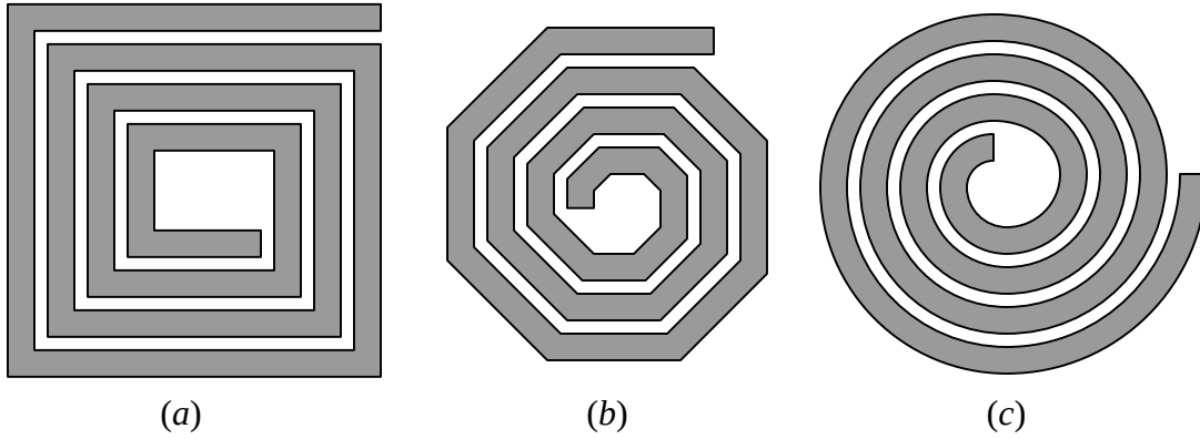
Figure 3.4: Typical integrated inductors: (a) square, (b) octagonal, and (c) circular spirals.
