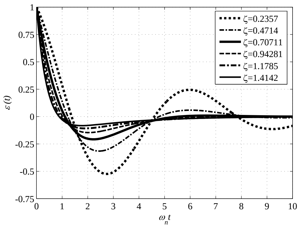
Figure 2.18: Unit step error response \varepsilon(t) vs. \omega_n t of second-order PLL.
