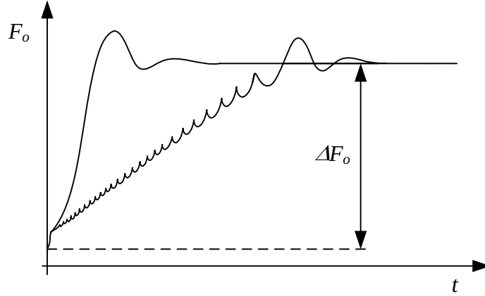
Figure 2.21: Typical locking response with and without cycle-slipping.
