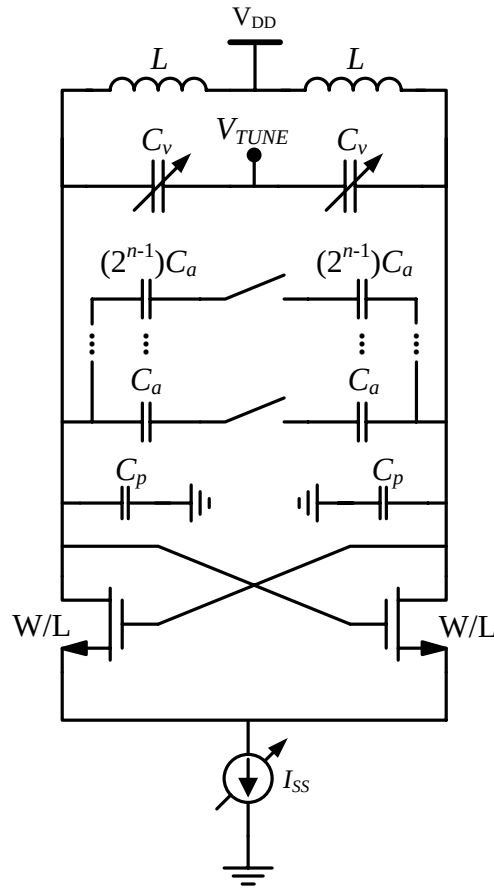
Figure 5.1: Simplified schematic of the VCO core.
