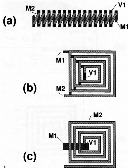
Figure 1. Schematic plan views of (a) a solenoidal inductor, (b) a multilevel-spiral (MLS) inductor, and (c) a planar spiral coil.
