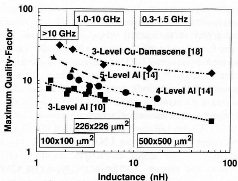
Figure 9. Q_{\max} vs. inductance values for different inductor geometries and fabrication processes.
