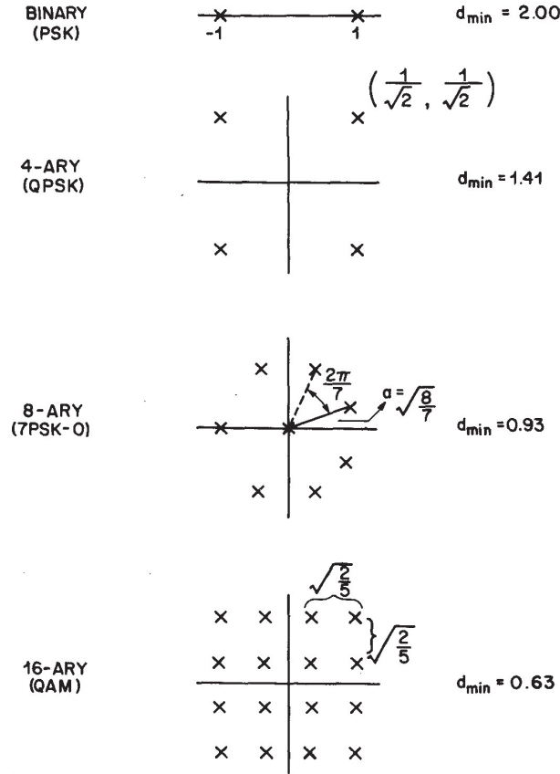
Fig. 11. Modulation formats used in simulations (average energy = 1).
