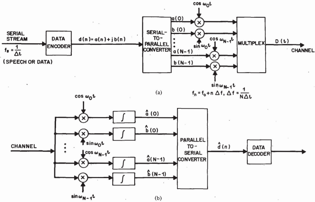
Fig. 1. Basic OFDM system. (a) Transmitter. (b) Receiver.
