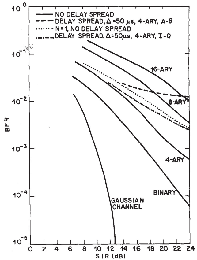
Fig. 12. Simulation results ( N = 128 , v = 30 mph, f_s = 7.5 kHz).
