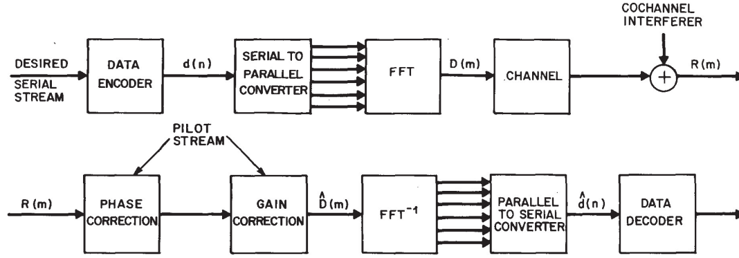
Fig. 2. OFDM system implemented with an FFT.
