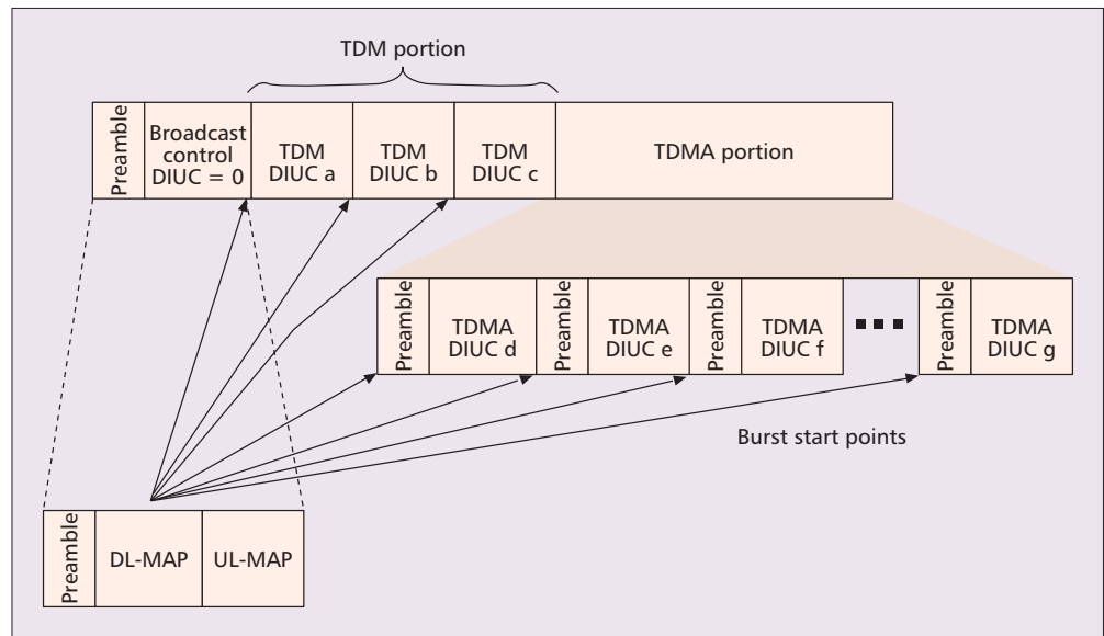
■ Figure 1. The downlink subframe structure.
