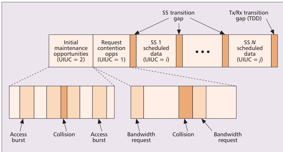
■ Figure 2. The uplink subframe structure.
