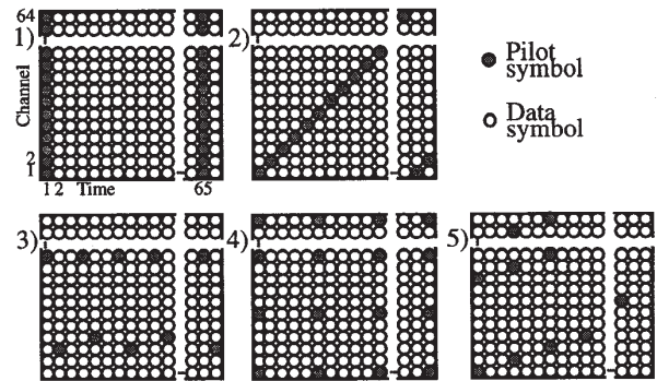
Fig. 2 Examples of pilot patterns analyzed.
