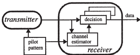
Fig. 1 The pilot pattern is known both by the receiver and the transmitter. The purpose is to minimize the number of transmitted pilot symbols without increasing the bit error rate.
