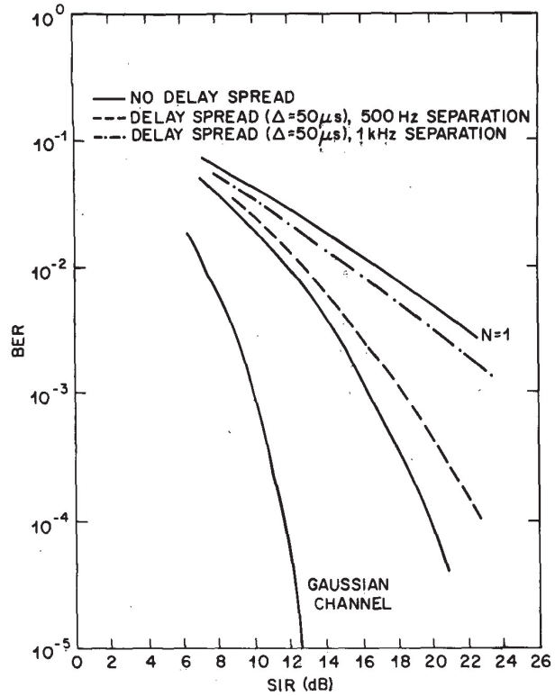
Fig. 7. Simulation results in a frequency-selective environment (QPSK, f_s = 7.5 \text{ kHz} , N = 512 , v = 60 \text{ mph} , gain-limited correction).
