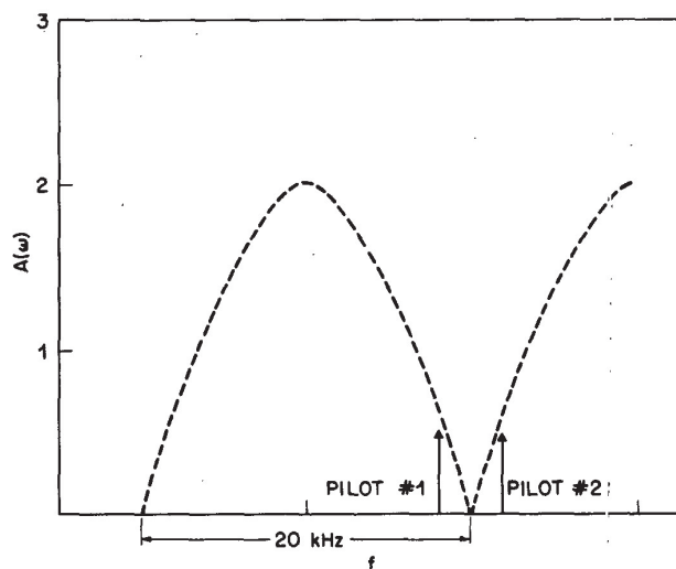
Fig. 9. Possible amplitude response for two-impulse channel model for delay spread, \Delta = 50 \mu\text{s} , A(\omega) = 2 |\cos \omega \Delta / 2| .
