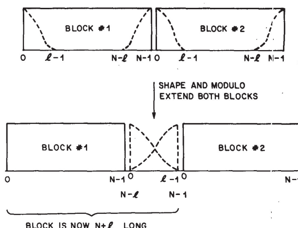
Fig. 8. Modulo extension and shaping of data block to reduce interchannel interference caused by impairment of orthogonality.
