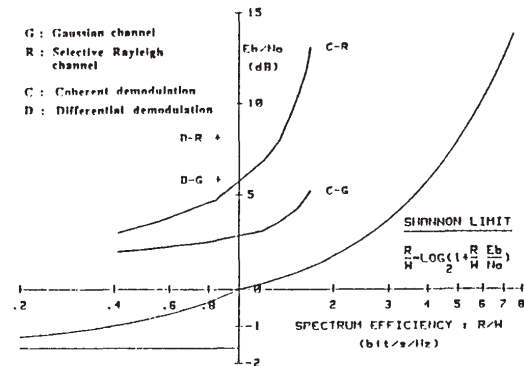
Figure 5 COFDM performances
