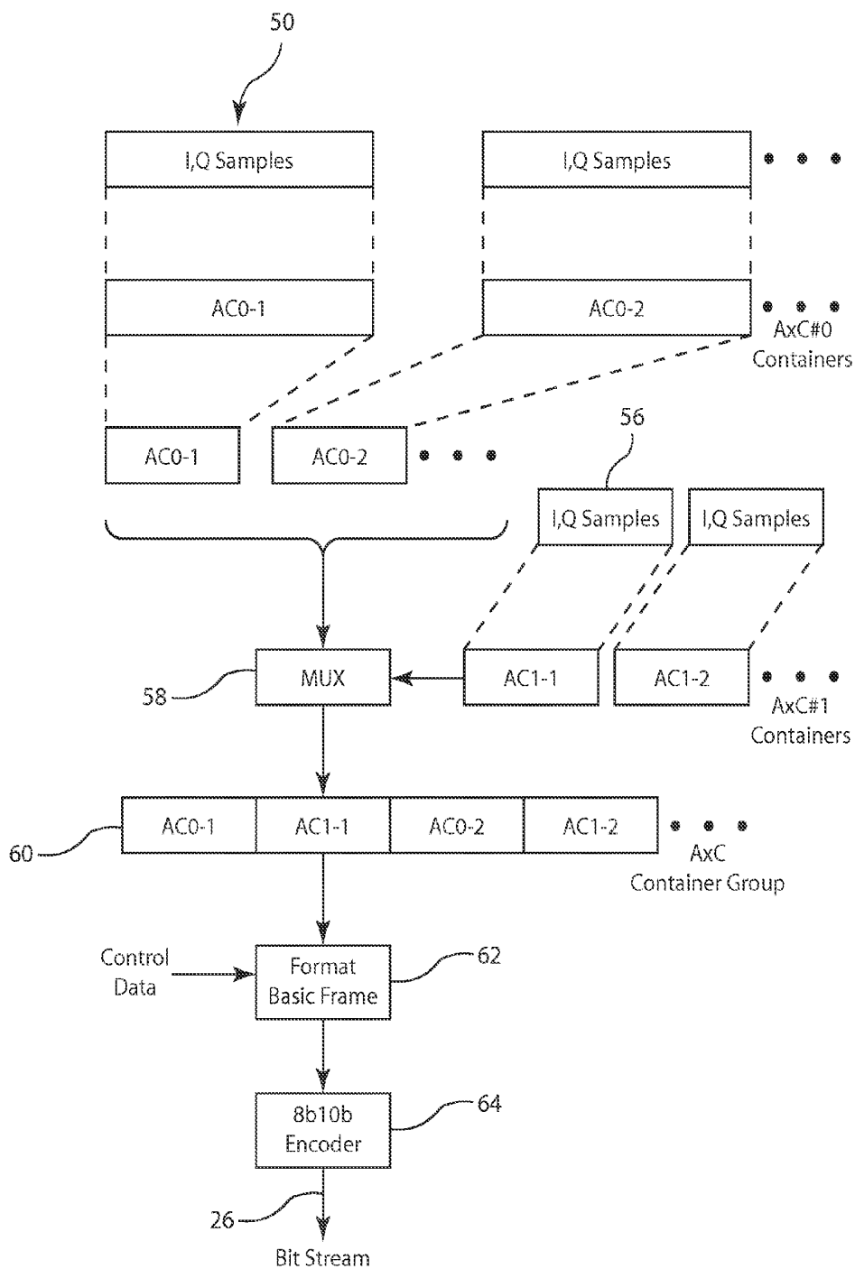
Figure 11 Prior Art
