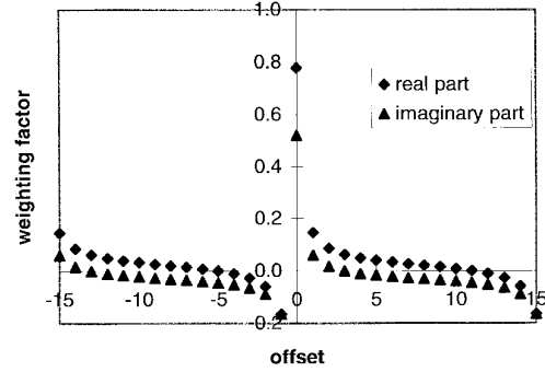
Fig. 2. Real and imaginary components of the complex weighting factors c_0 \cdots c_{N-1} for the case of \Delta f T = 0.2 and N = 16 .
