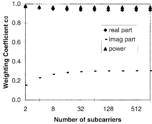
Fig. 3. c_0 as function of number of subcarriers for \Delta fT = 0.1 .
