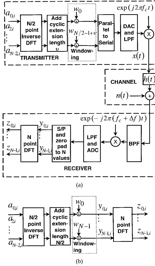
Fig. 4. (a) Windowing to reduce sensitivity to frequency offset. (b) Simplified block diagram of windowing.
