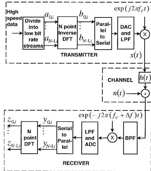
Fig. 1. Structure of an OFDM communication system.
