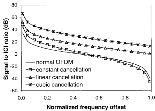
Fig. 5. Wanted signal power/uncancelled ICI power as a function of f/\Delta fT .
