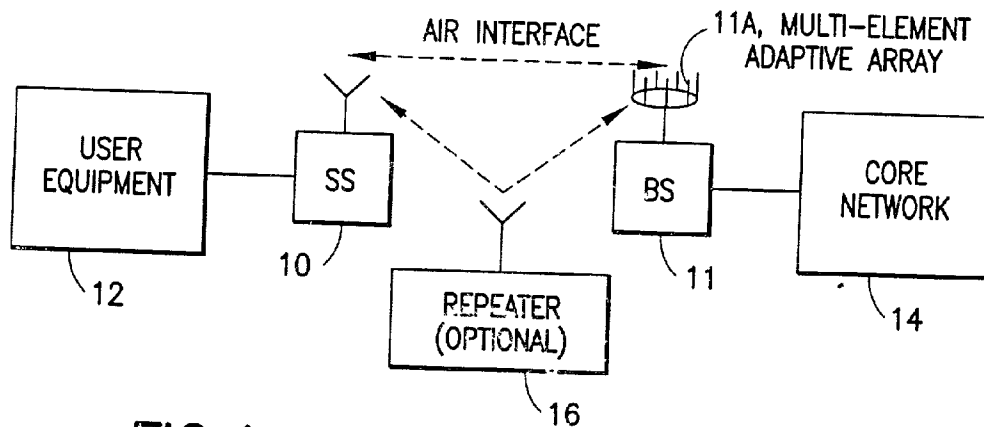
FIG. 1 WIRELESS ACCESS REFERENCE MODEL
