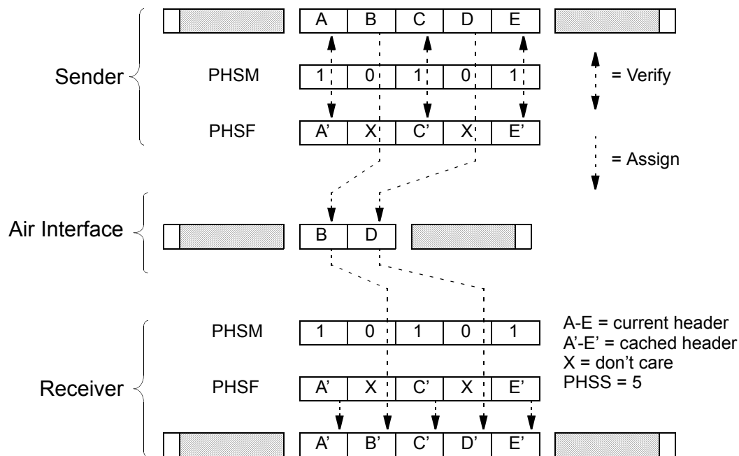
Figure 10—Payload header suppression with masking
