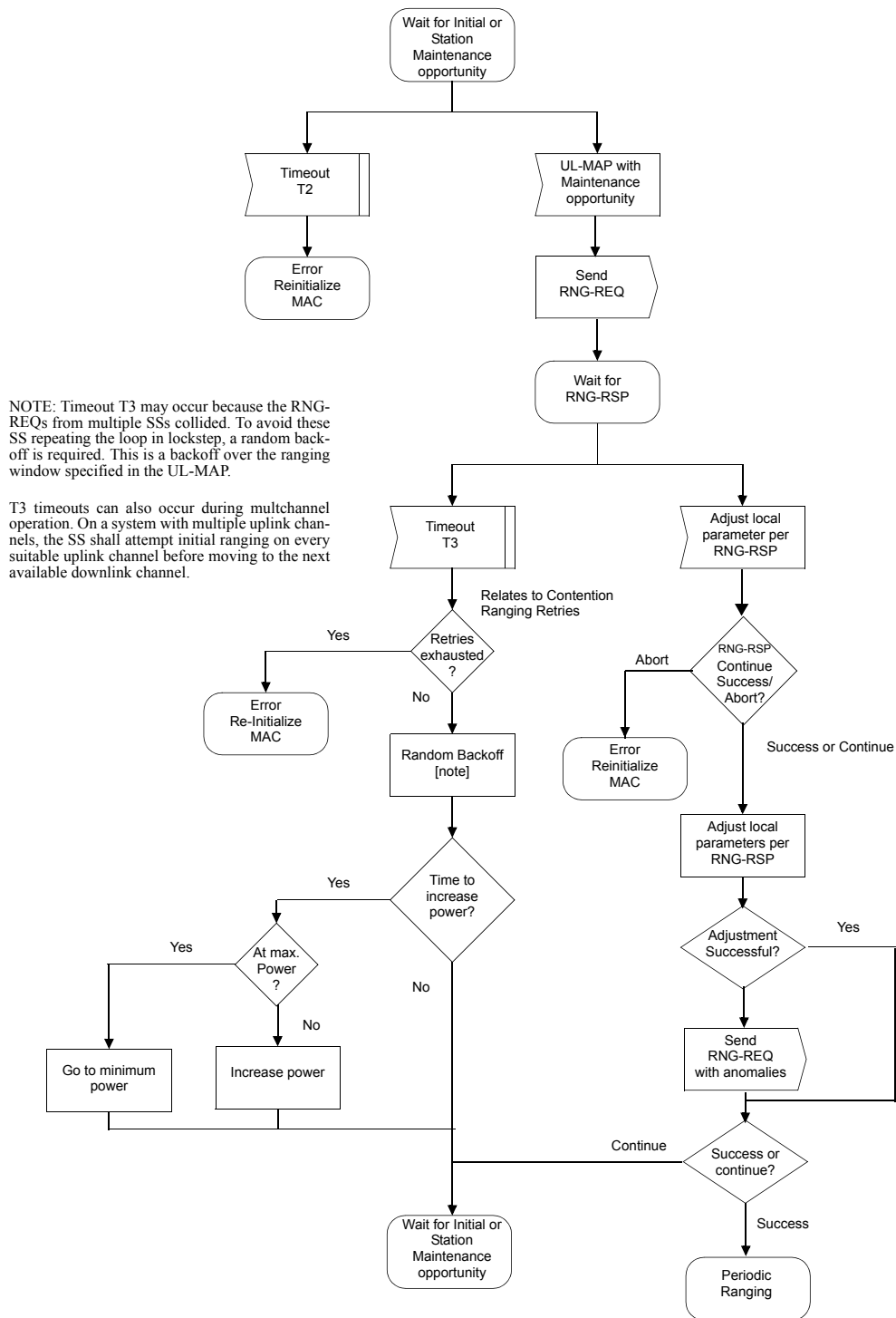
Figure 50—Initial Ranging—SS
