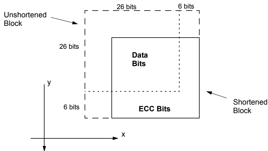
Figure 125—Structure of shortened 2 D block
