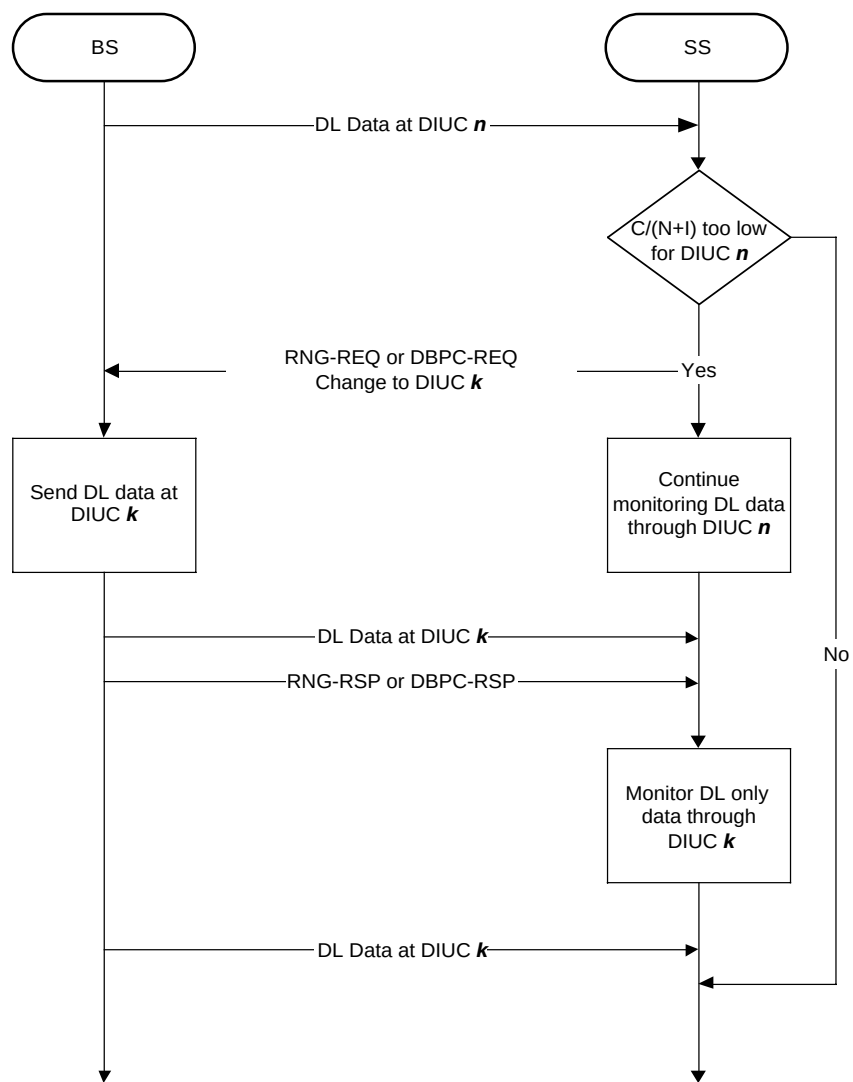
Figure 57—Transition to a more robust burst profile
