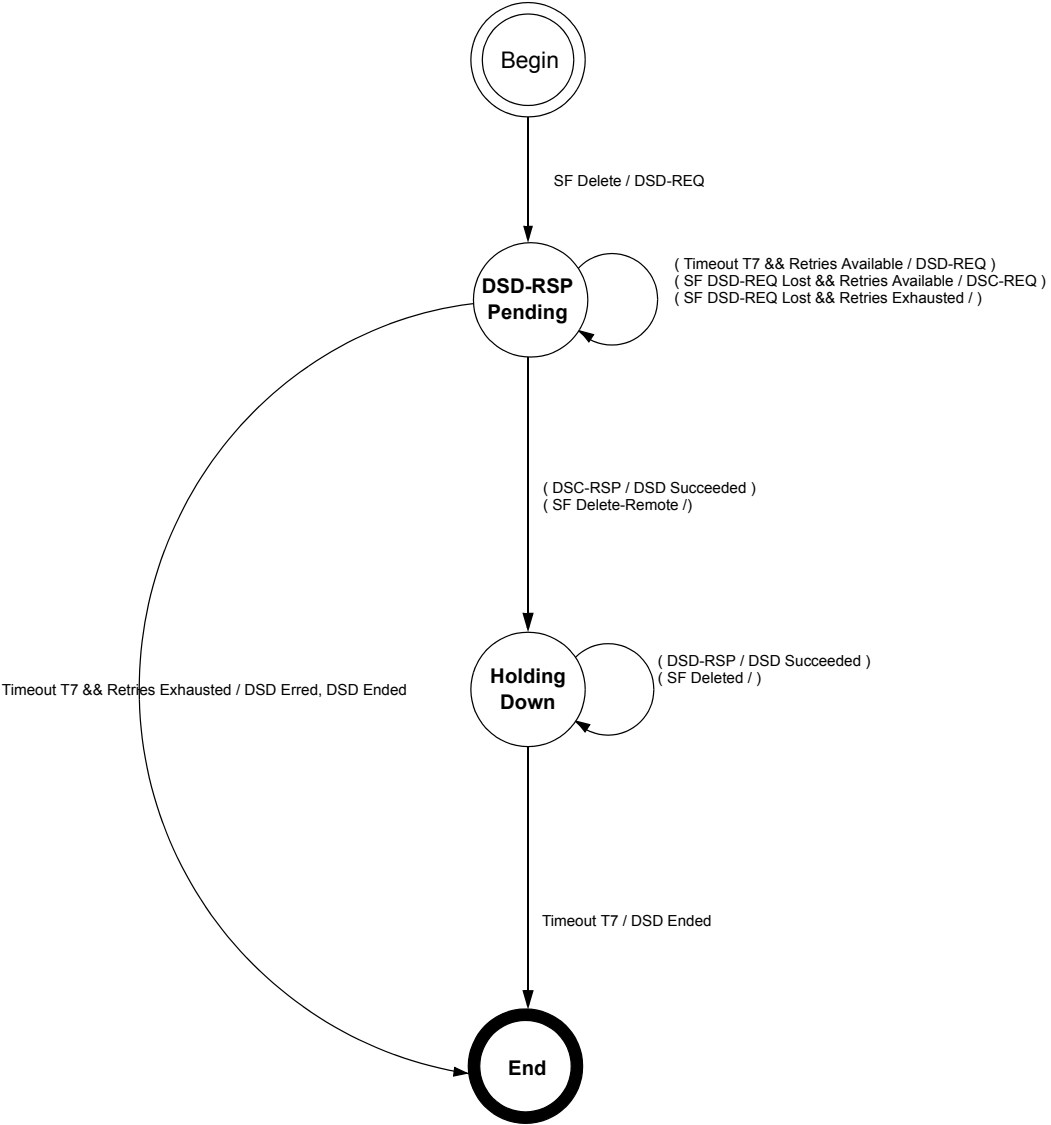
Figure 73—DSD—Locally initiated transaction state transition diagram
