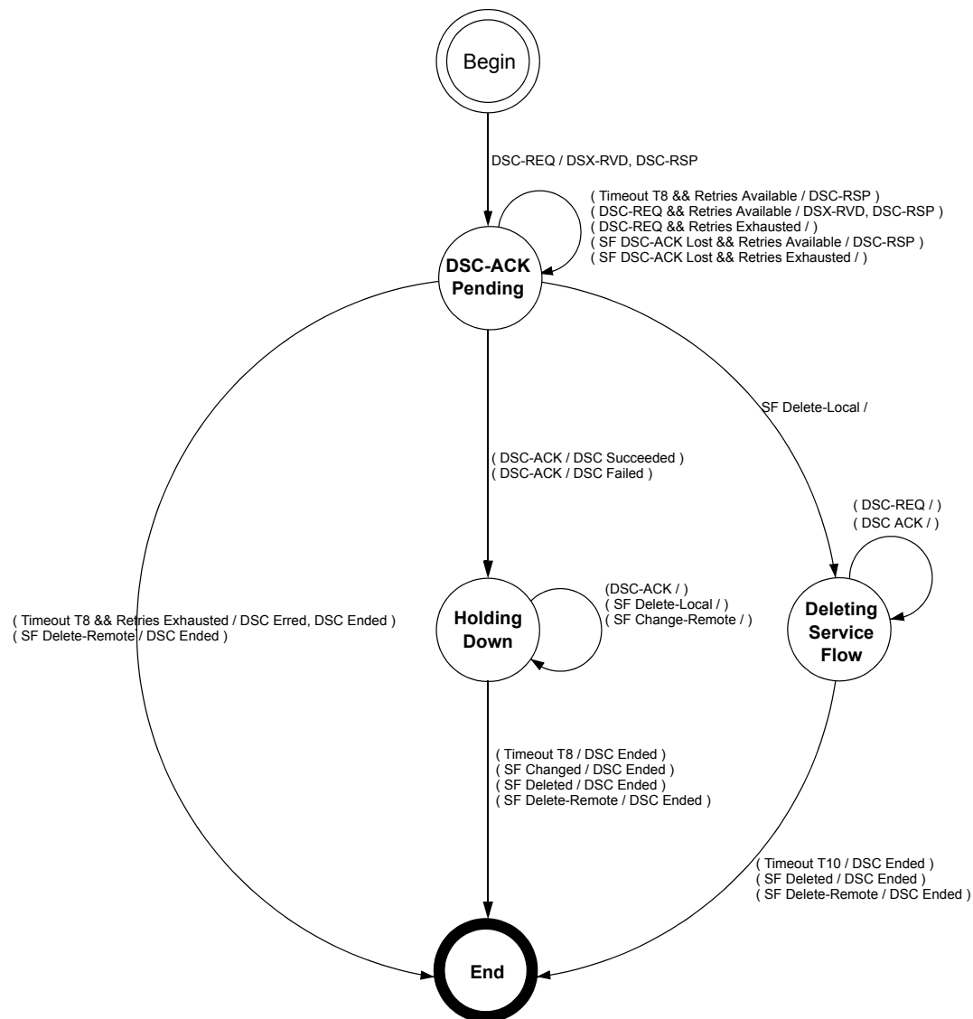
Figure 72—DSC—Remotely initiated transaction state transition diagram
