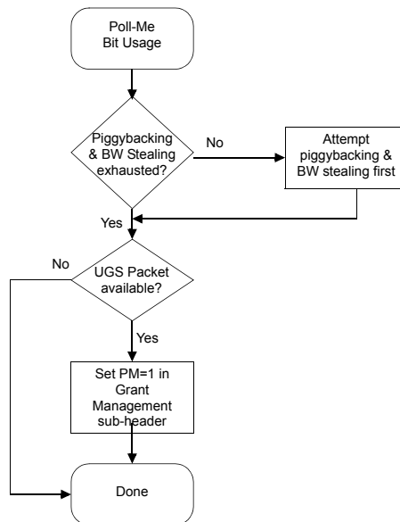
Figure 36—Poll-Me bit usage
