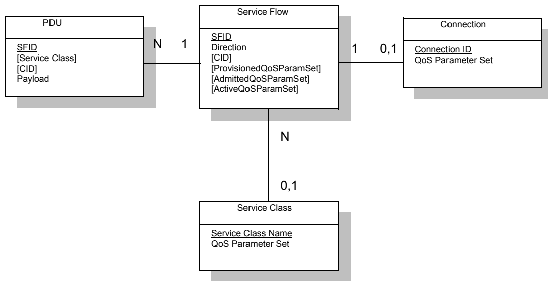
Figure 64—Theory of Operation Object Model
