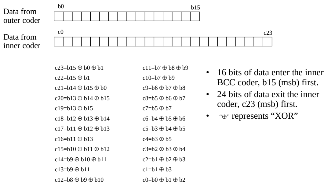
Figure 116—Inner code for Code Type 2 in the downlink
