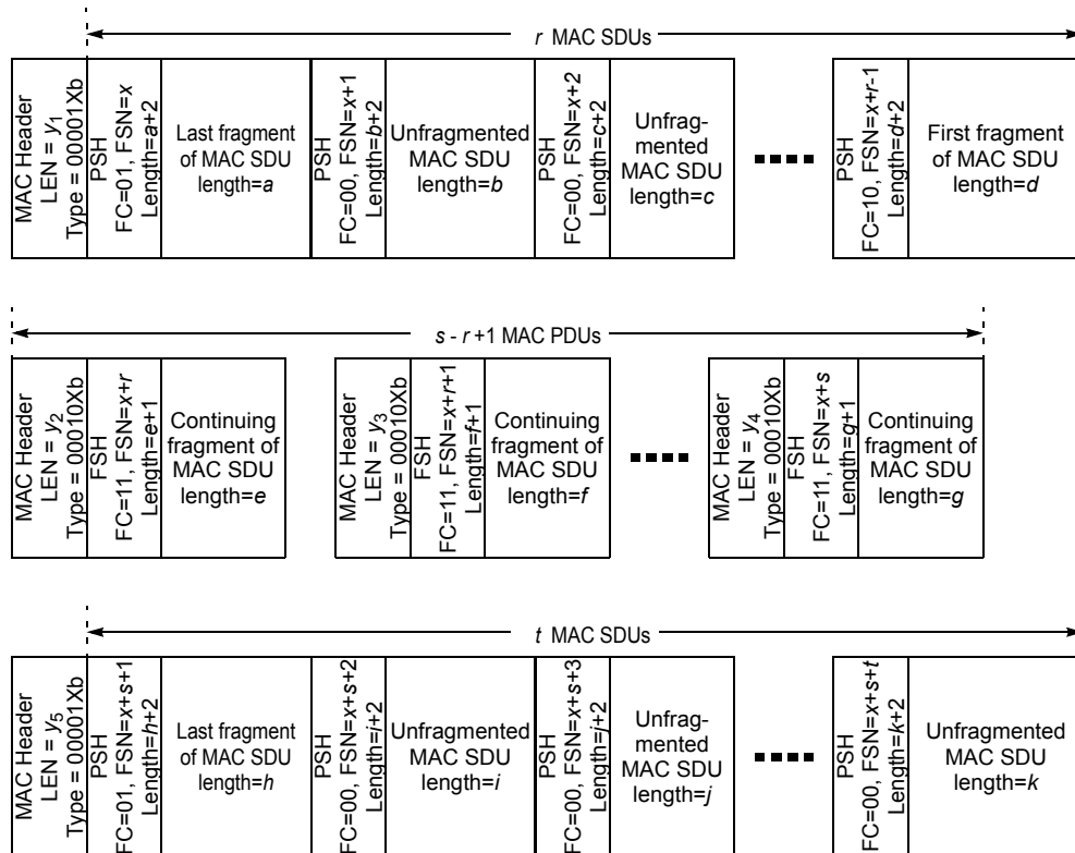
Figure 30—Packing with fragmentation
