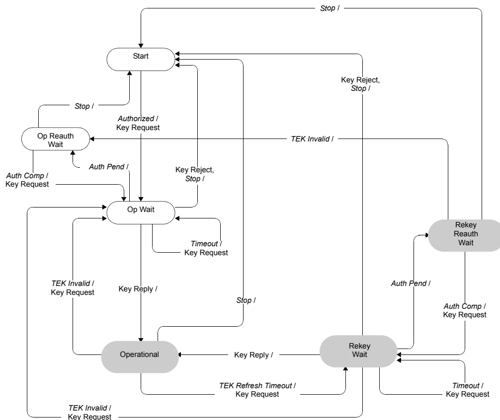
Figure 98—TEK state machine flow diagram
