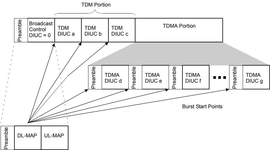
Figure 110—FDD downlink subframe structure
