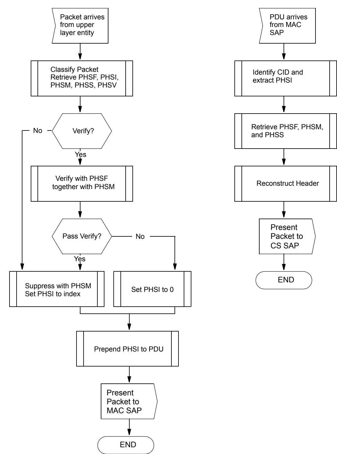
Figure 9—Payload header suppression operation
