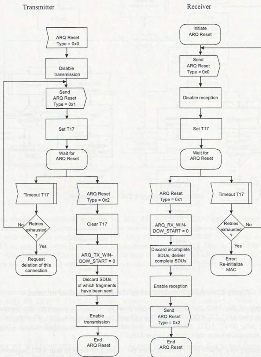
Figure 31b—ARQ Reset message dialog—receiver initiated
