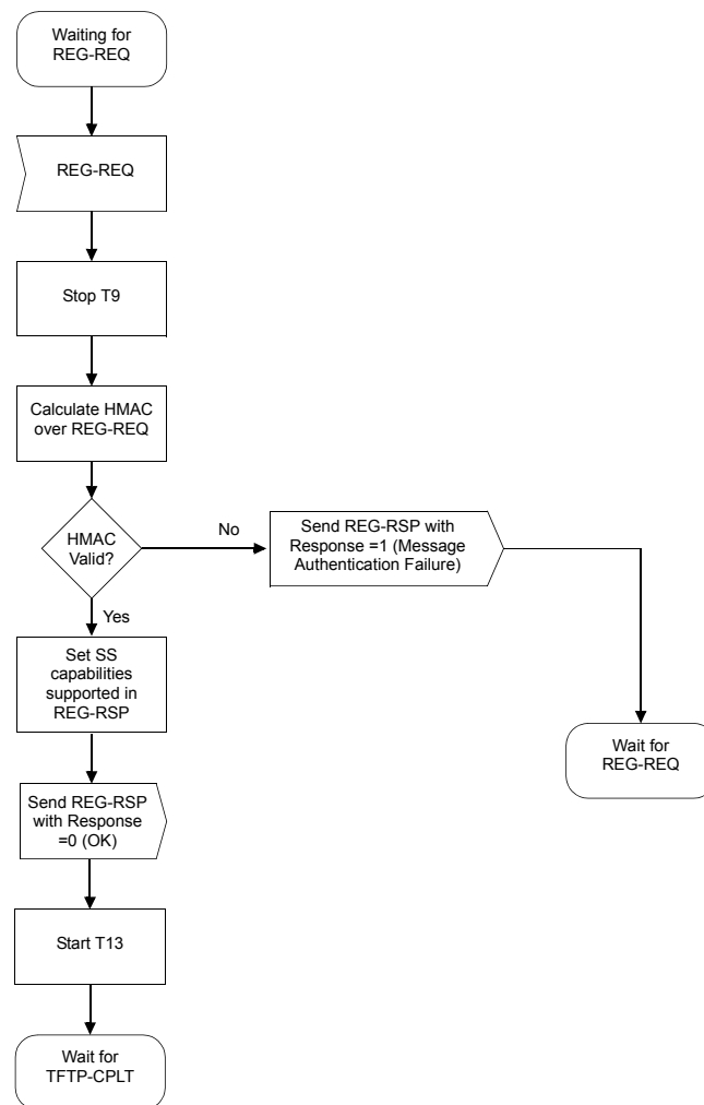
Figure 54—Registration—BS
