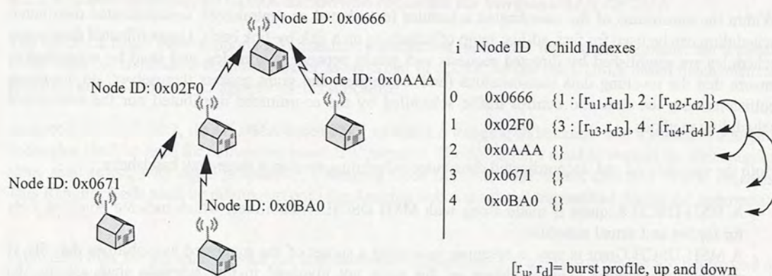
Figure 36a—MSH-CSCF schedule example
