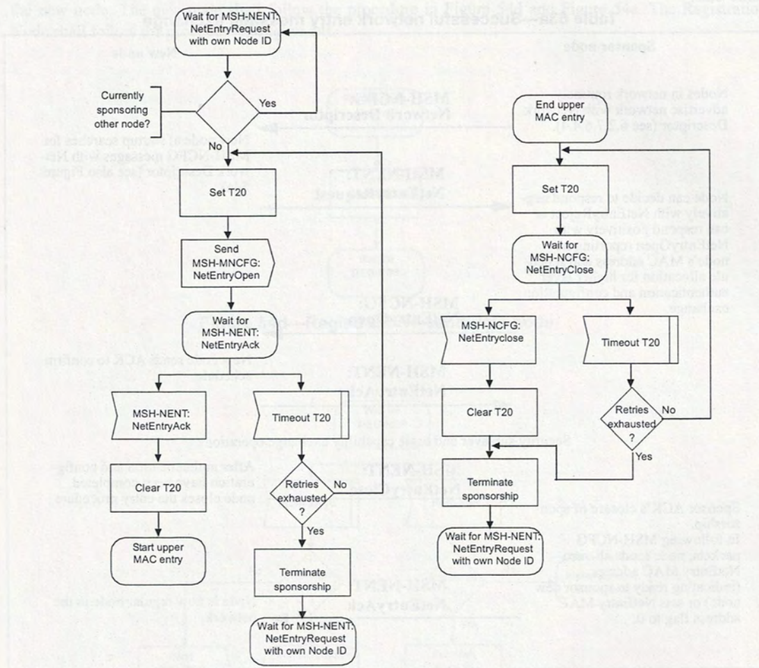
Figure 54c—Mesh network synchronization and entry—sponsor node
