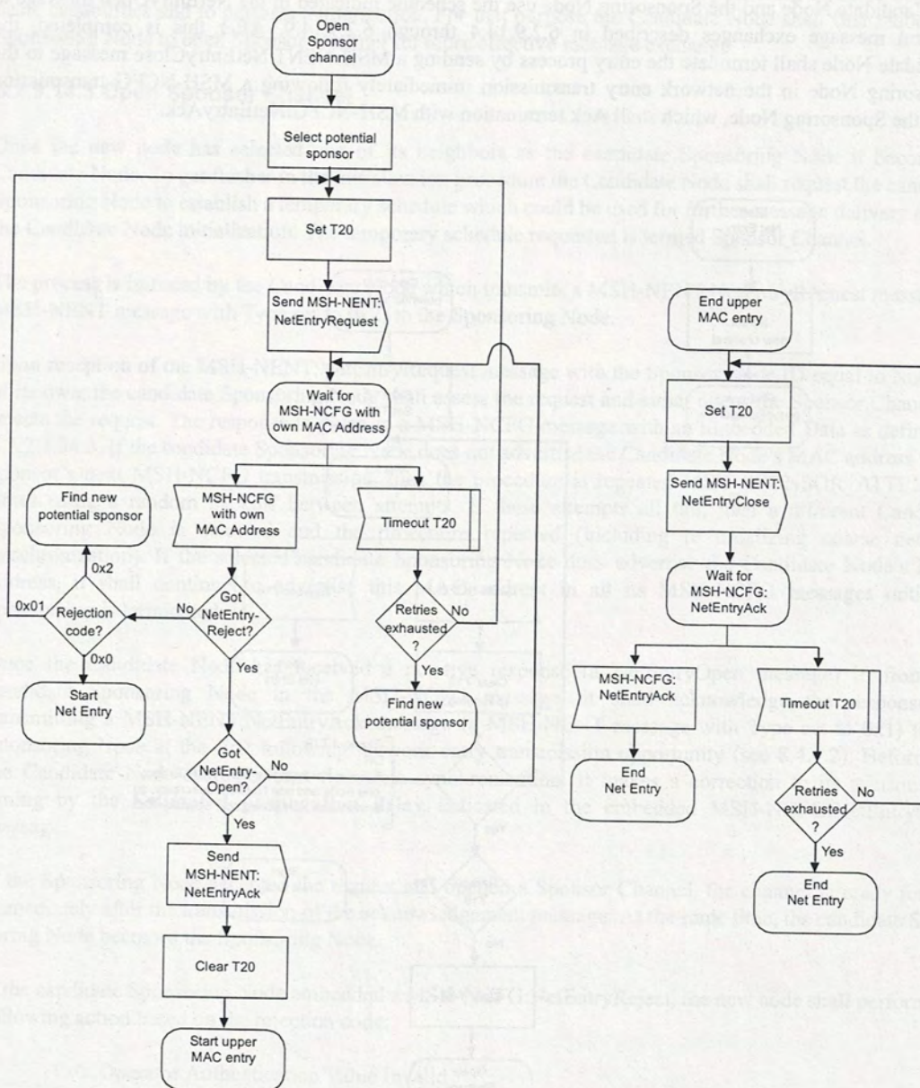
Figure 54b—Mesh network synchronization and entry—New node—II
