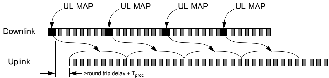
Figure 43—Time relevance of UL-Map information (unframed FDD)
