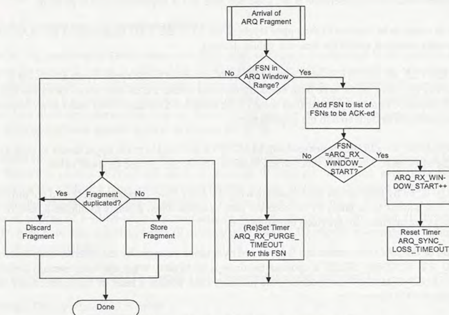
Figure 31d—ARQ fragment reception
