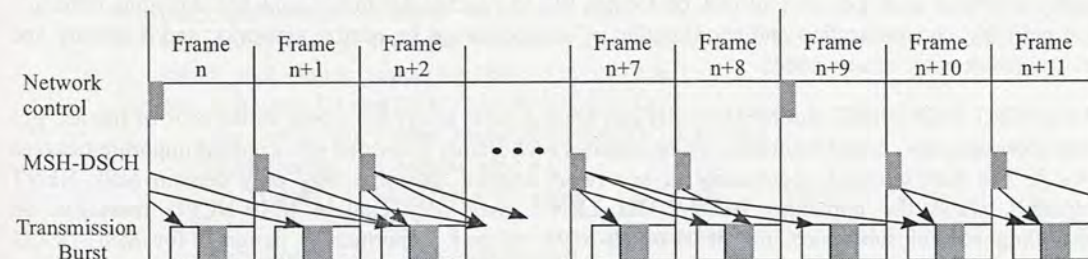
Figure 43c—Time relevance example of MSH-DSCH in distributed scheduling
