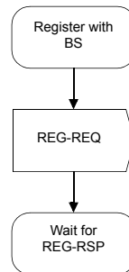
Figure 52—Registration—SS
