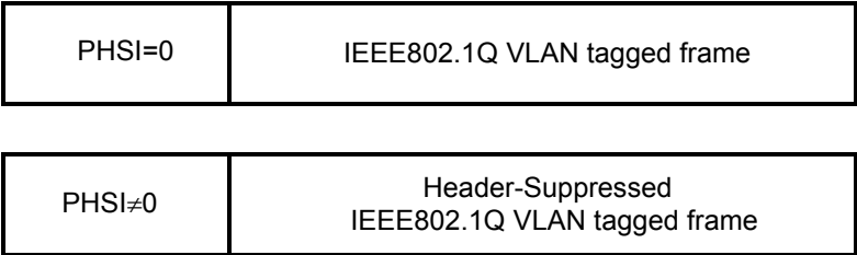
Figure 14—IEEE 802.1Q VLAN CS PDU format
