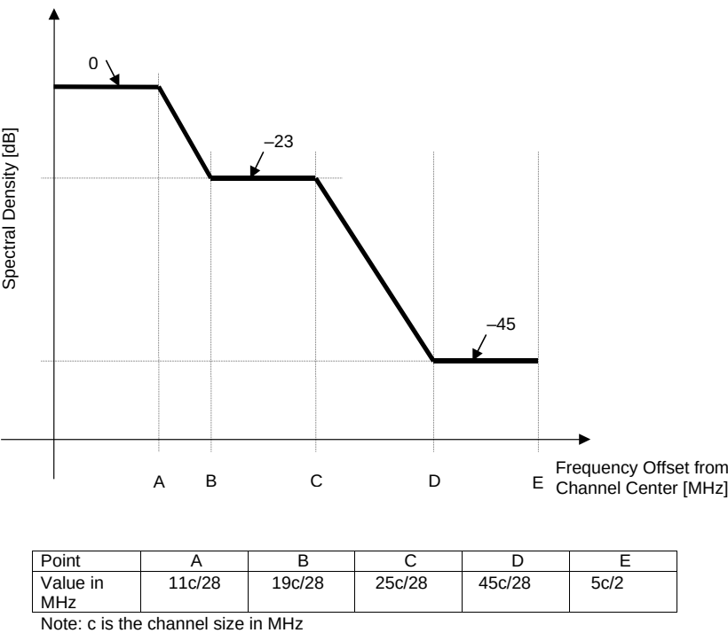
Figure 126—ETSI Type A spectrum mask
