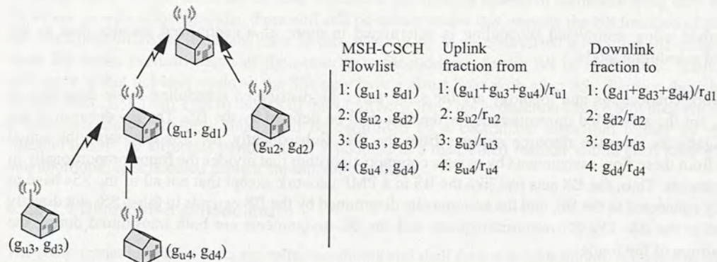
Figure 36b—MSH-CSCF flow usage example
