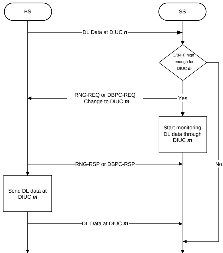
Figure 58—Transition to a less robust burst profile
