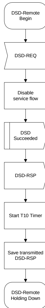
Figure 96—DSD—Remotely initiated transaction begin state flow diagram
