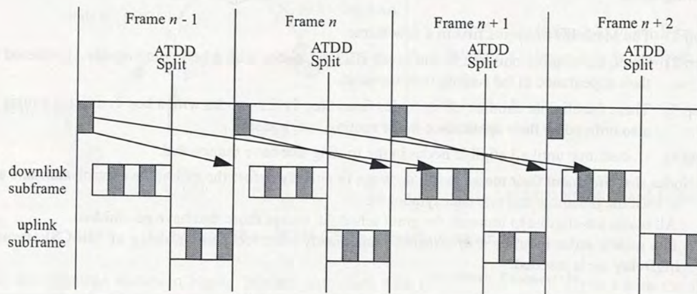
Figure 43a—Time relevance of PHY and MAC control information (TDD)
