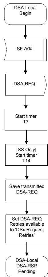
Figure 75—DSA—Locally initiated transaction begin state flow diagram
