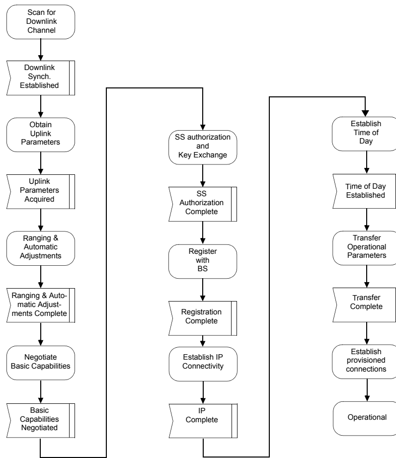
Figure 45—SS Initialization overview
