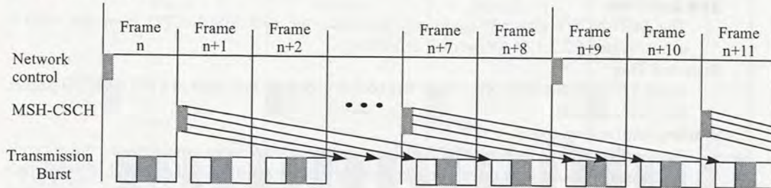
Figure 43d—Time relevance example of MSH-CSCH in centralized scheduling
