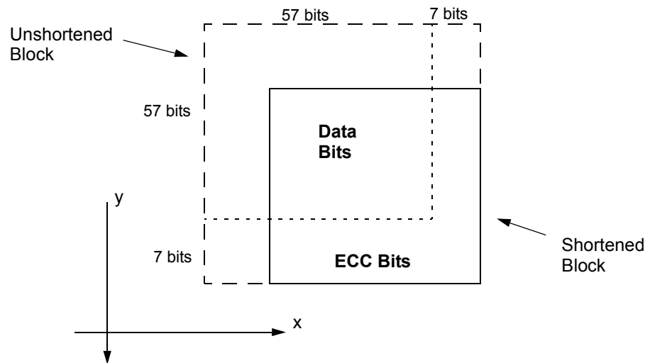
Figure 119—Structure of shortened 2 D block
