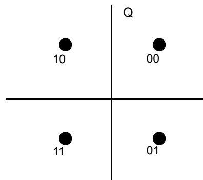
Figure 120—QPSK constellation
