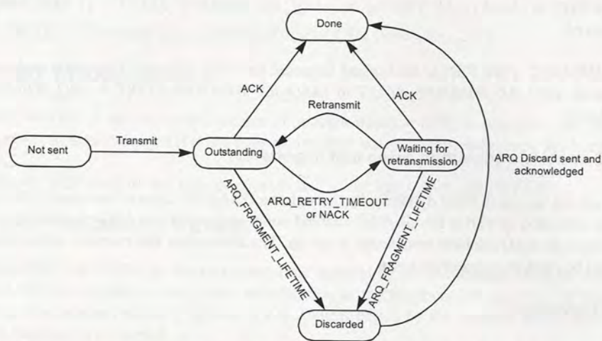
Figure 31a—ARQ transmit fragment states
