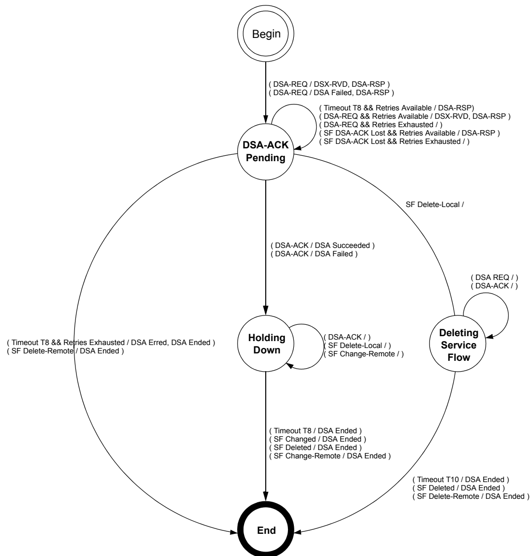
Figure 70—DSA—Remotely initiated transaction state transition diagram
