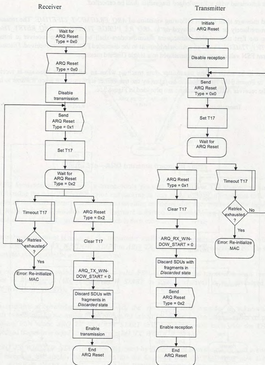
Figure 31c—ARQ Reset message dialog—transmitter initiated
