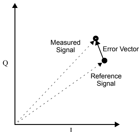
Figure 129—Illustration of EVM
