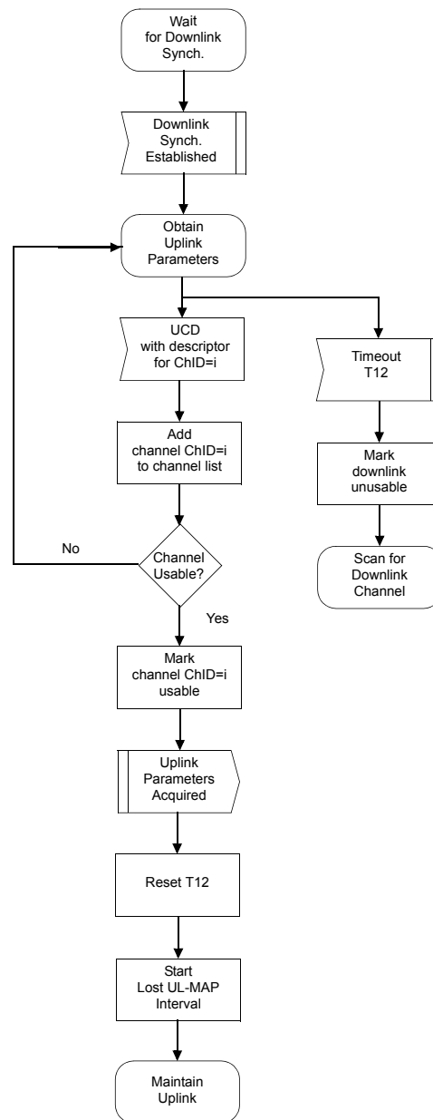
Figure 48—Obtaining uplink parameters
