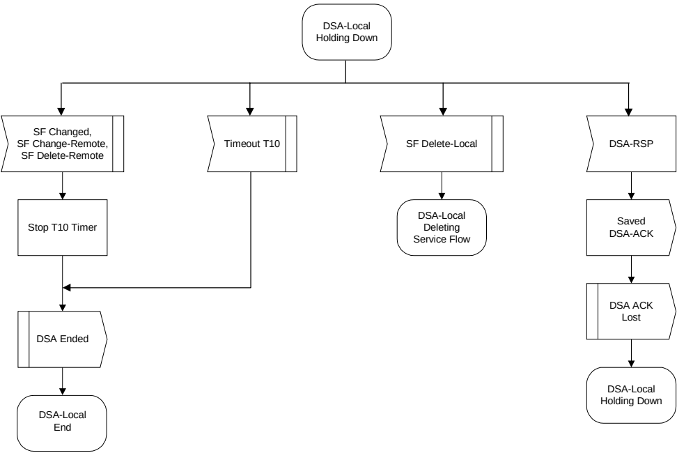
Figure 77—DSA—Locally initiated transaction holding state flow diagram
