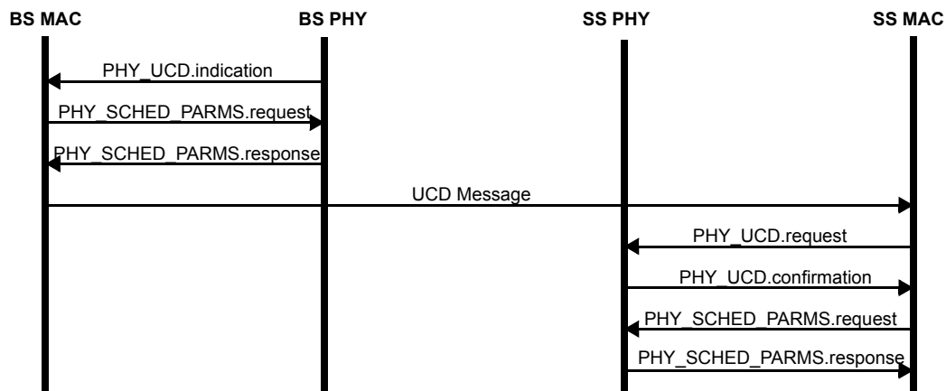
Figure 102—Example of usage of PHY_UCD primitives
