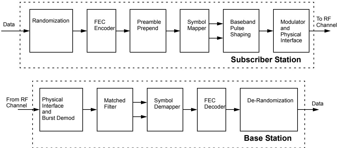
Figure 124—Conceptual block diagram of the uplink PHY
