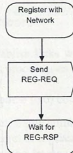
Figure 54d—Registration—candidate node
