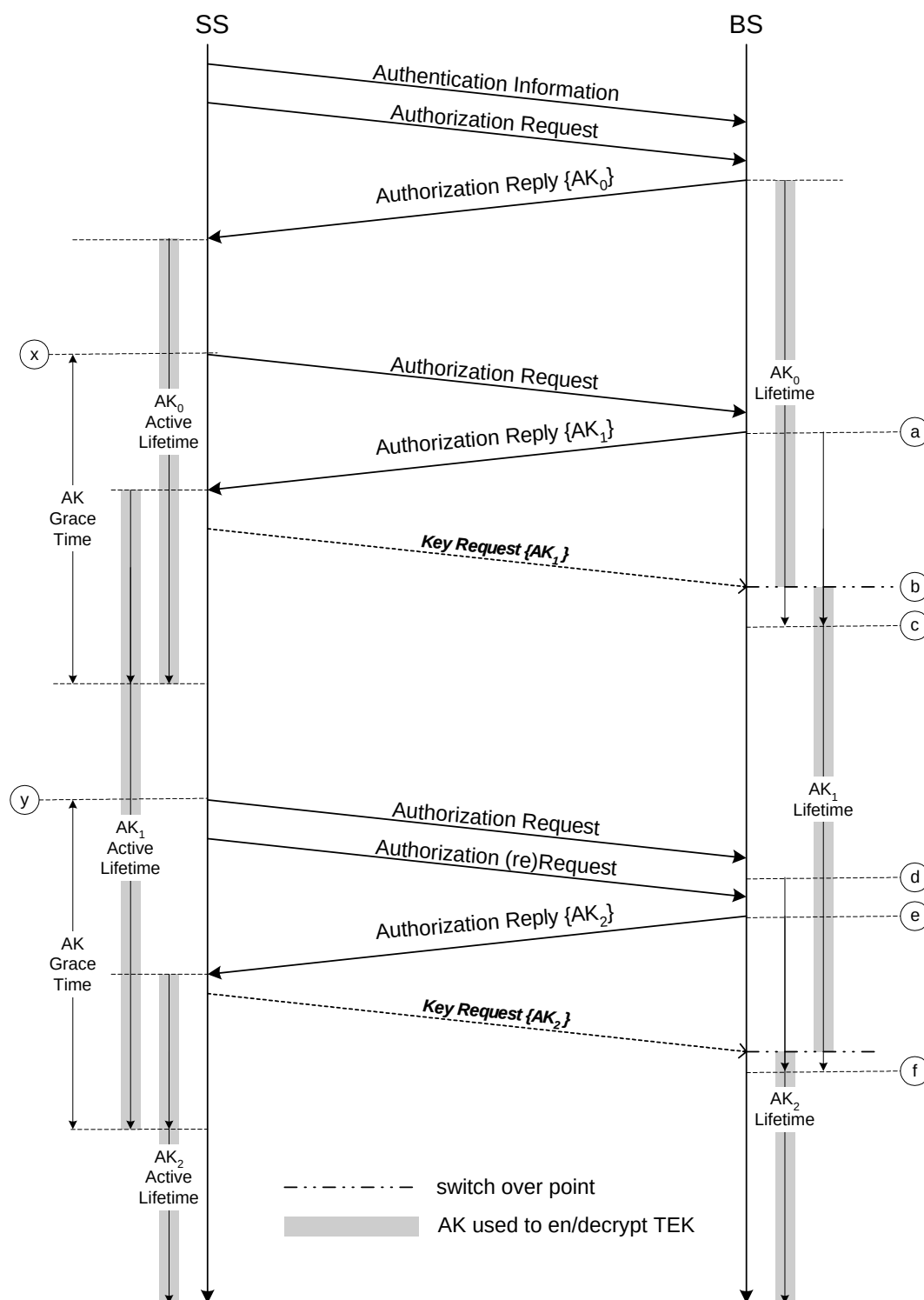
Figure 99—AK management in BS and SS
