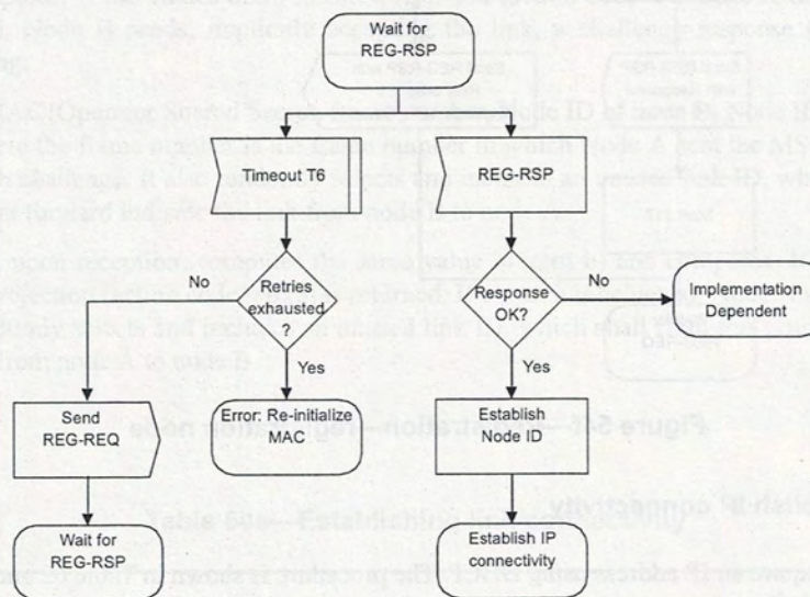
Figure 54e—Wait for registration response—candidate node
