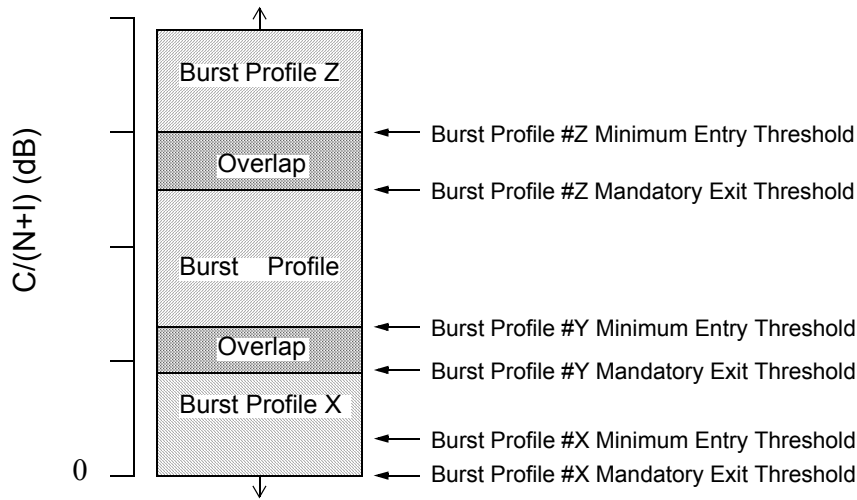
Figure 59—Burst profile threshold usage
