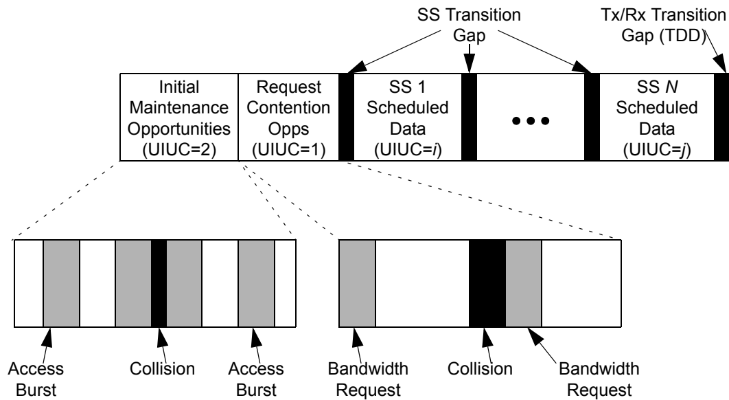
Figure 123—Uplink subframe structure
