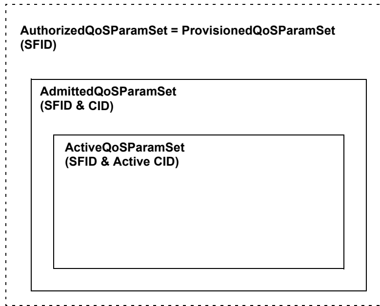
Figure 62—Provisioned authorization model “envelopes”
