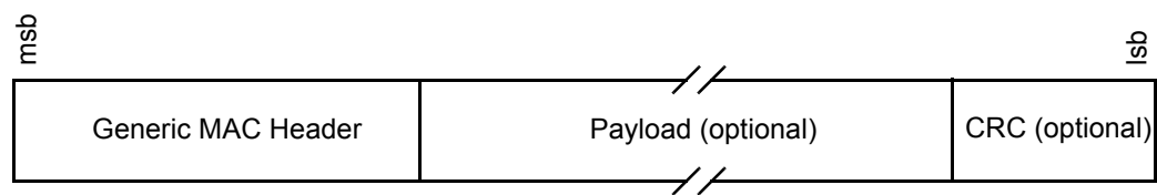
Figure 21—MAC PDU formats
