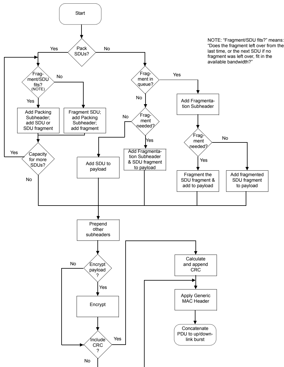
Figure 25—Construction of a MAC PDU
