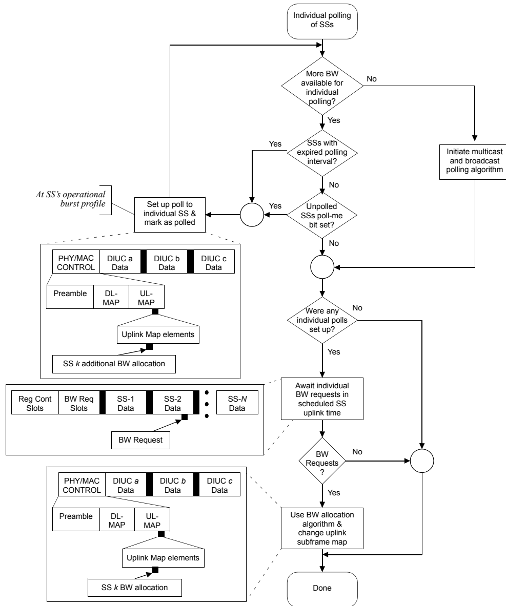
Figure 34—Unicast polling
