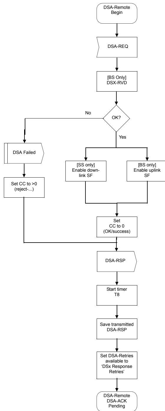
Figure 80—DSA—Remotely initiated transaction begin state flow diagram
