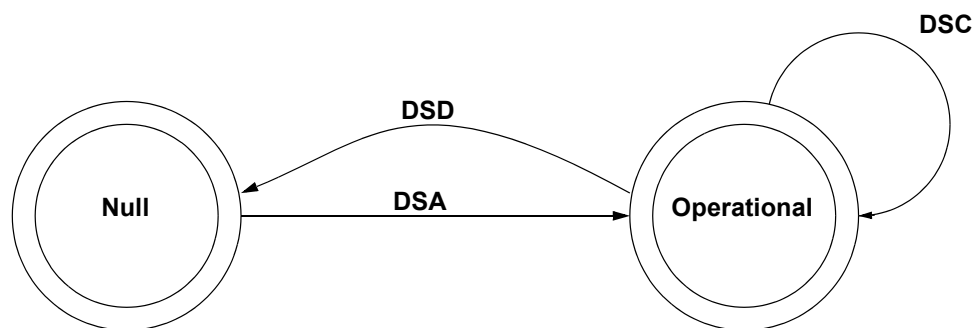
Figure 67—Dynamic service flow overview
