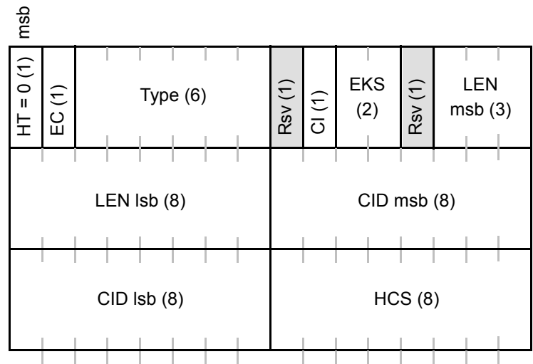
Figure 22—Generic MAC header format
