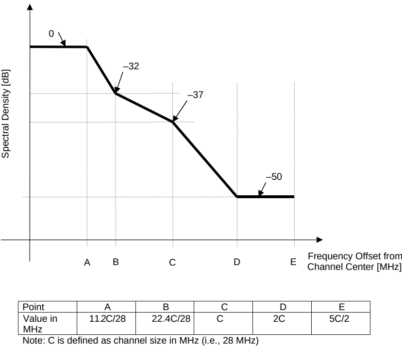
Figure 127—ETSI Type B spectrum mask
