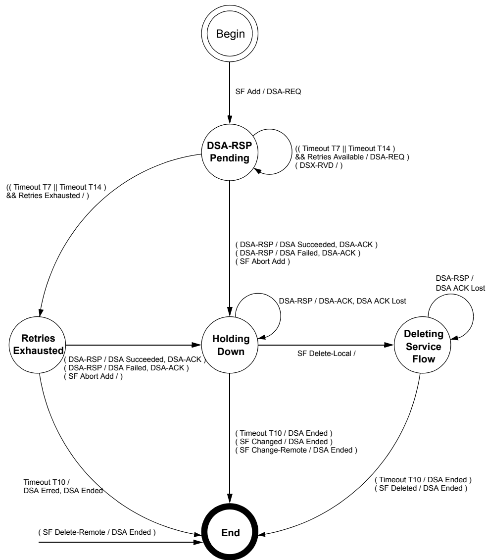
Figure 69—DSA—Locally initiated transaction state transition diagram
