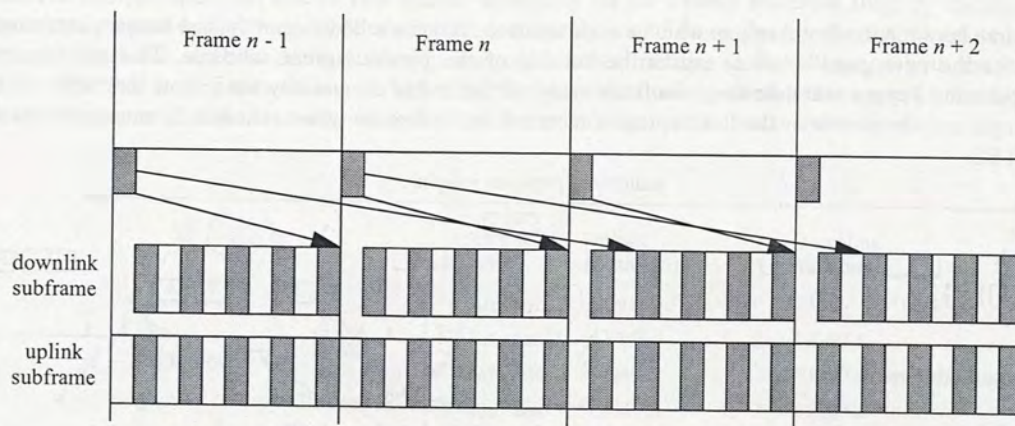
Figure 43b—Time relevance of PHY and MAC control information (FDD)
