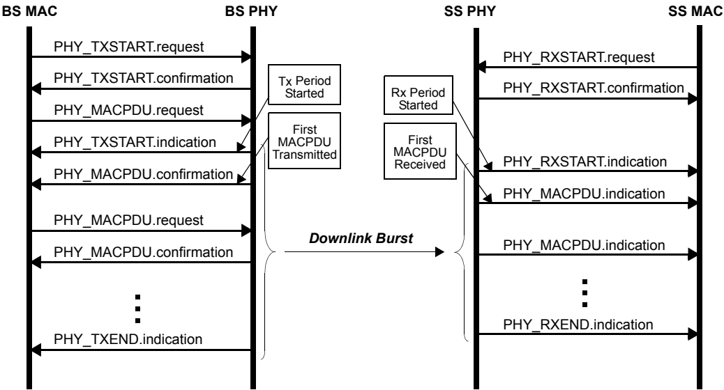
Figure 105—Example of usage of primitives during downlink PHY PDU transfer
