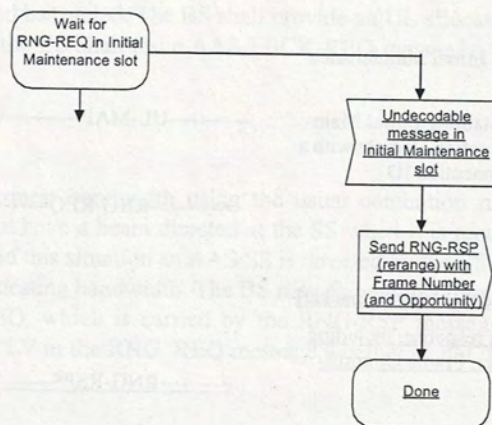
Figure 51a—Initial ranging—BS response to undecodable message
