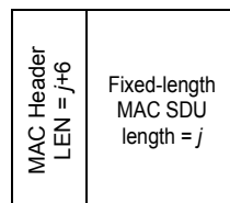
Figure 29—Packing a single variable-length MAC SDU into a single MAC PDU
