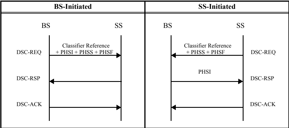
Figure 11—Payload header suppression signaling example
