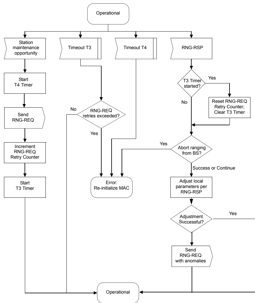
Figure 56—Periodic Ranging—SS
