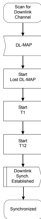
Figure 46—Obtaining downlink synchronization
