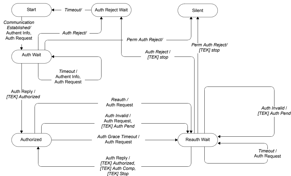
Figure 97—Authorization state machine flow diagram
