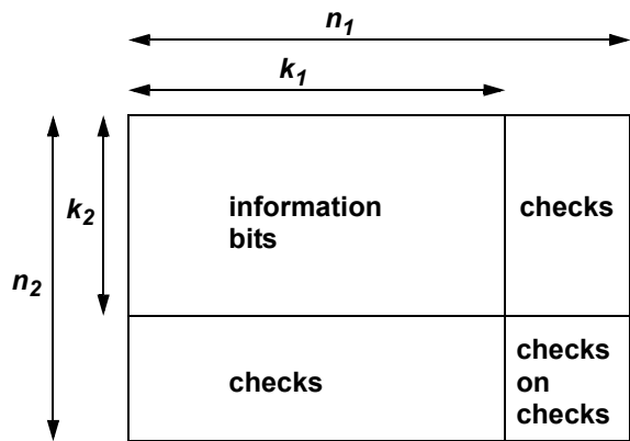
Figure 117—Two-dimensional product code matrix
