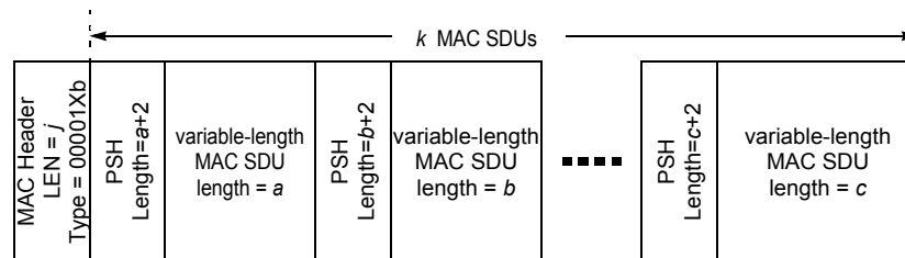
Figure 28—Packing variable-length MAC SDUs into a single MAC PDU
