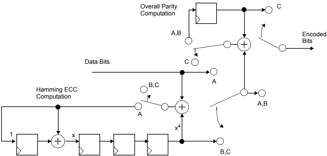
Figure 118—Example encoder for a (16,11) extended Hamming Code
