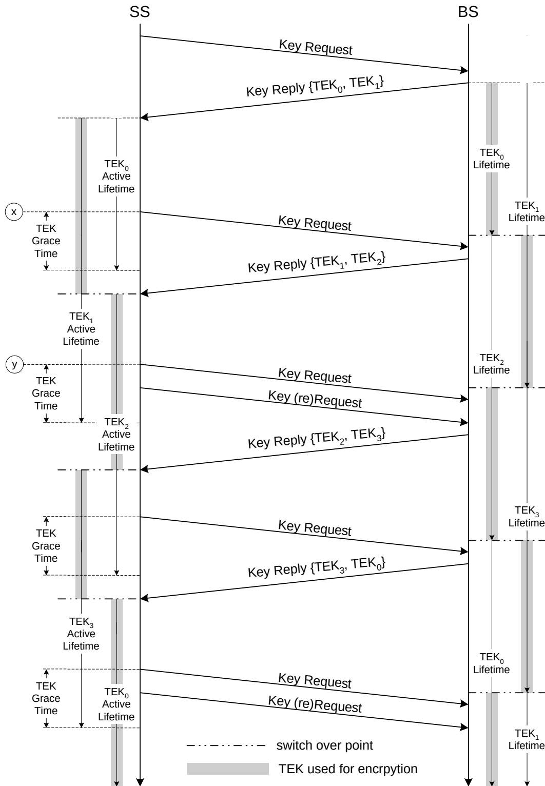
Figure 100—TEK management in BS and SS
