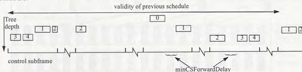
Figure 36c—MSH-CSCH schedule validity
