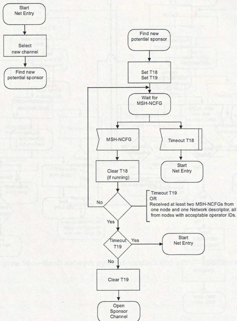
Figure 54a—Mesh network synchronization and entry—New node—I
