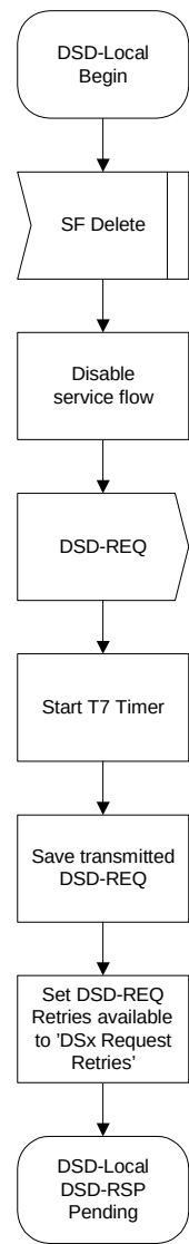
Figure 93—DSD—Locally initiated transaction begin state flow diagram
