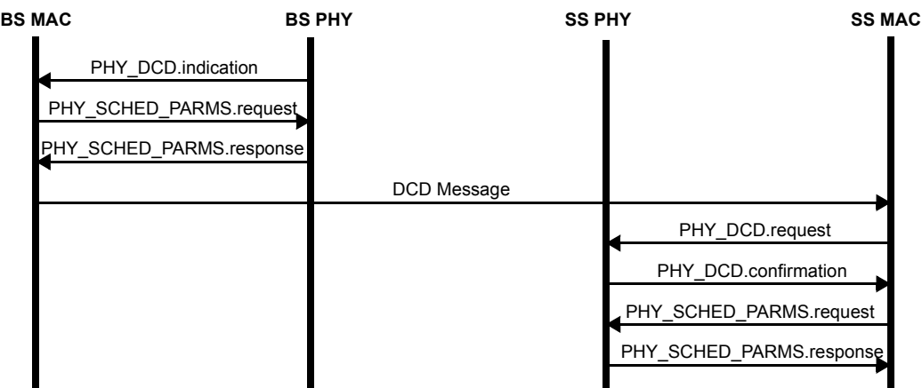
Figure 101—Example of usage of PHY_DCD primitives
