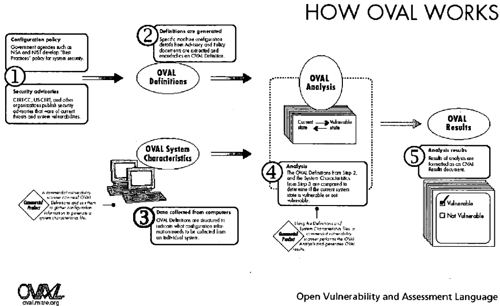
FIGURE 18: Open Vulnerability Assessment Language
