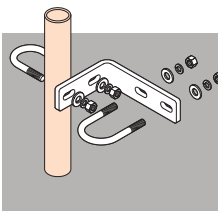
U-bolt to stanchion
