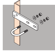
Bolt/Weld to stanchion
