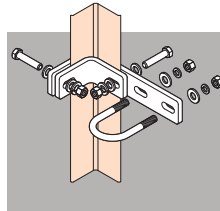
Clamp to stanchion
