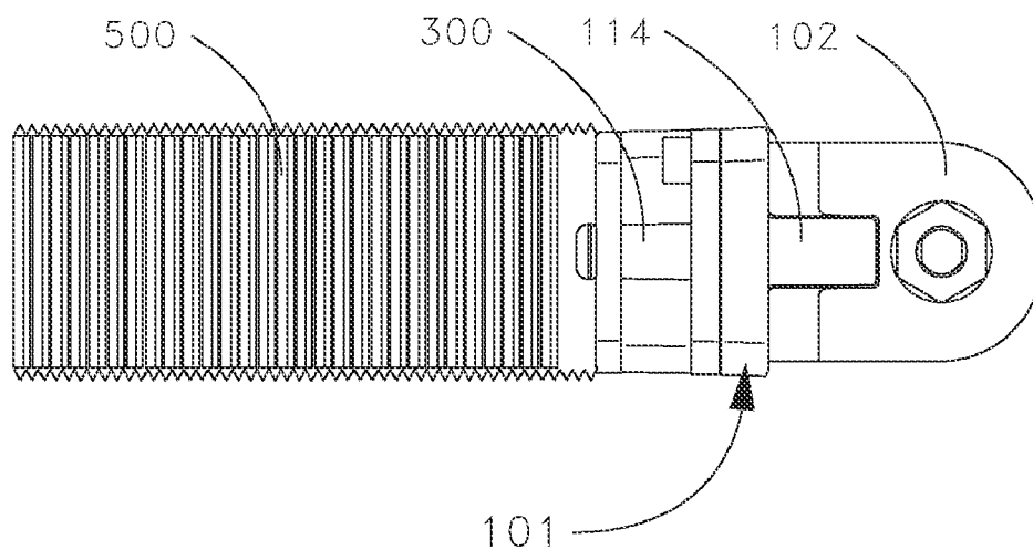
TOP VIEW Fig. 6D
