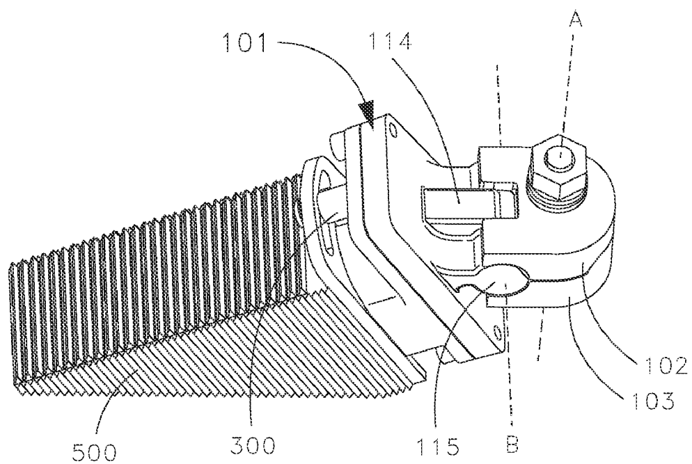
TOP RIGHT VIEW Fig. 6C
