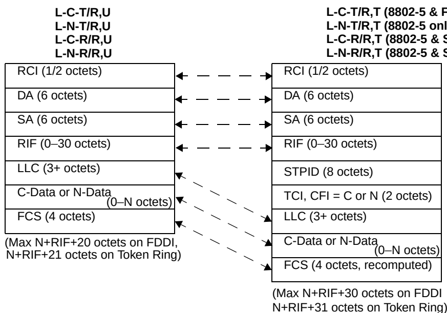
Figure C-14—Translation between L-X-X/R,U and L-X-X/R,T (8802-5 & SR FDDI)
