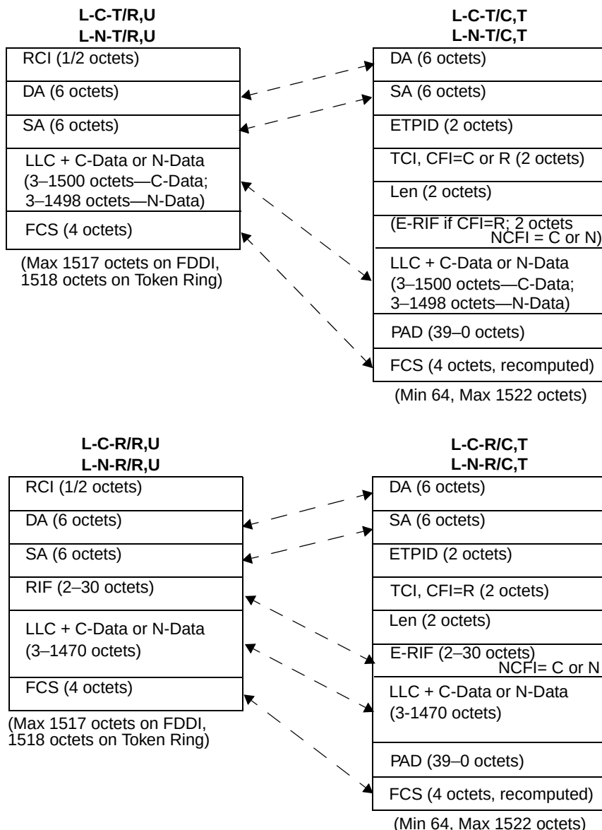
Figure C-13—Translation between L-X-X/R,U and L-X-X/C,T
