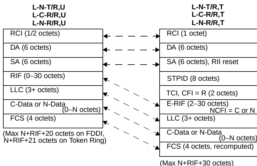
Figure C-15—Translation between L-X-X/R,U and L-X-X/R,T (transparent FDDI)
