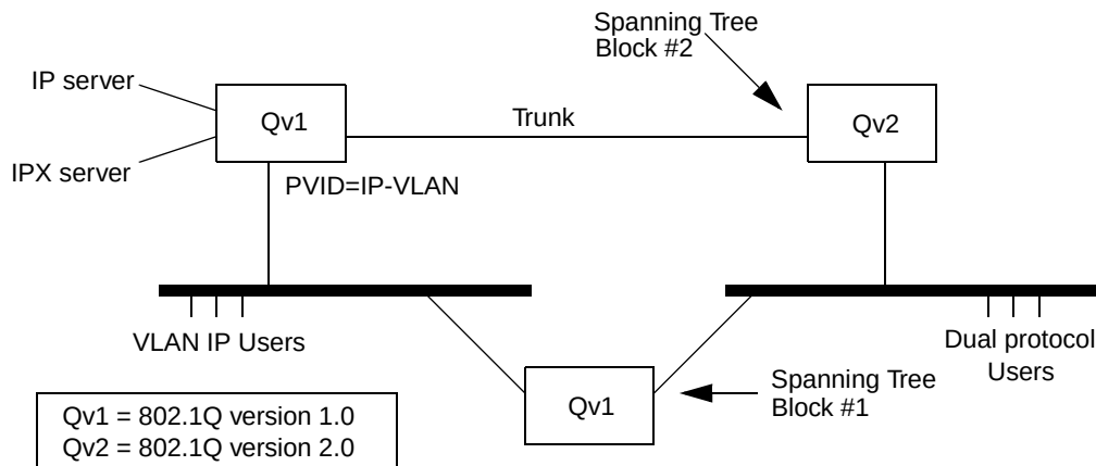
Figure E-4—Interoperability between Q versions 1 and 2
