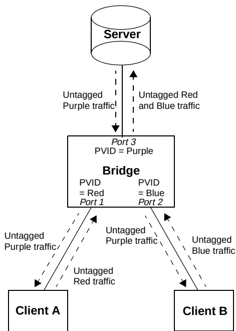
Figure B-4—Asymmetric VLAN use: “multi-netted server”
