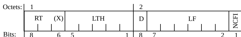
Figure 9-5—E-RIF Route Control (RC) field
