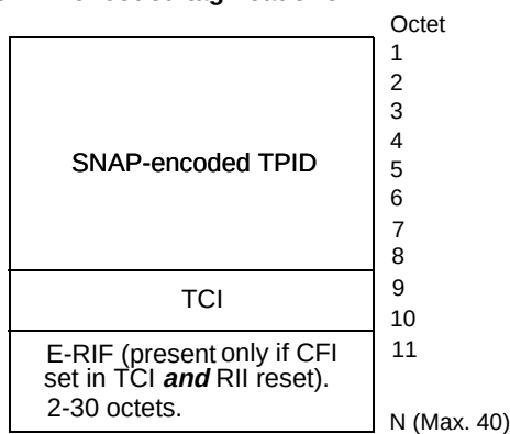
Figure 9-1—Tag header formats
