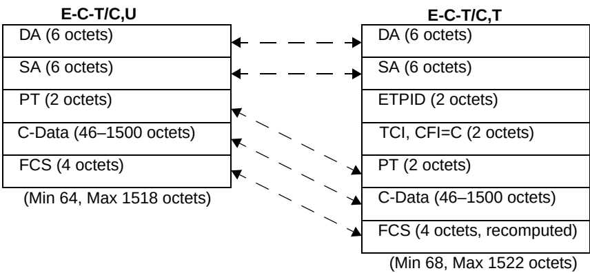
Figure C-6—Translation between E-C-T/C,U and E-C-T/C,T
