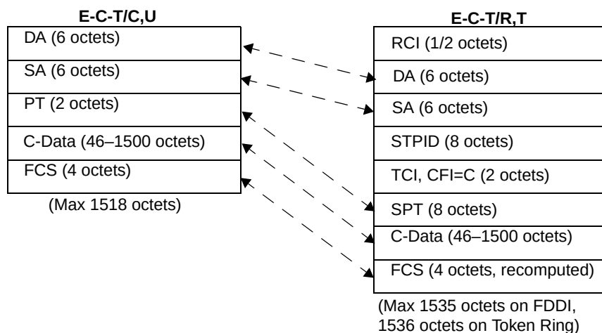
Figure C-7—Translation between E-C-T/C,U and E-C-T/R,T
