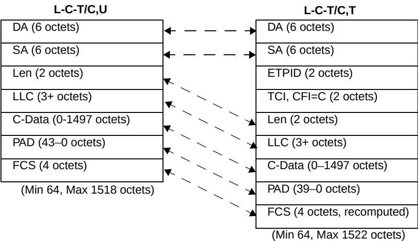
Figure C-8—Translation between L-C-T/C,U and L-C-T/C,T
