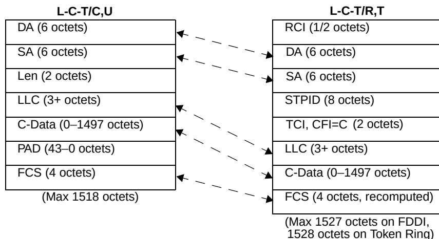
Figure C-9—Translation between L-C-T/C,U and L-C-T/R,T
