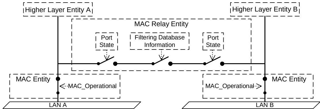
Figure 7-10—Effect of control information on the forwarding path
