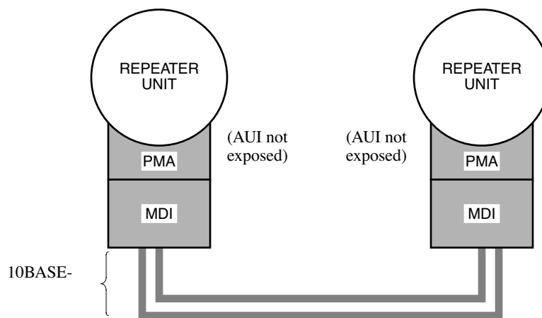
b) 10BASE-FB relationship to CSMA/CD LAN
