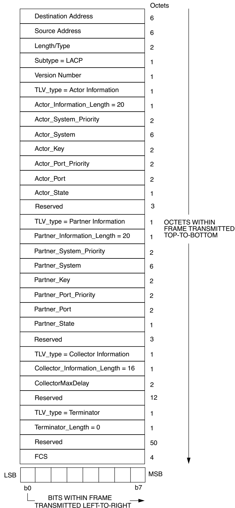
Figure 43-7—LACPDU structure
