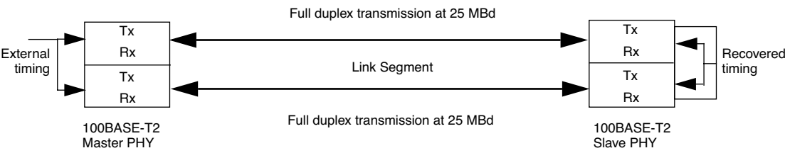
Figure 32-2—100BASE-T2 topology
