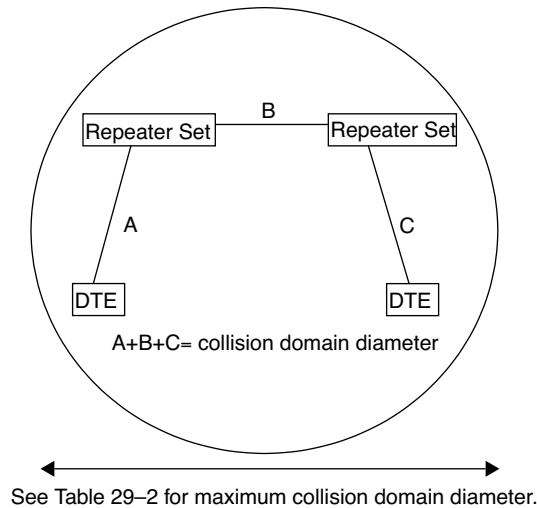
Figure 29-5—System Model 1: Two Class II repeaters
