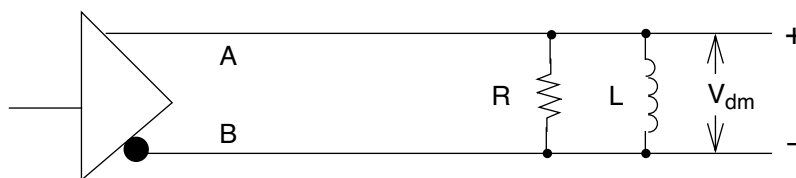
Figure 7–11—Differential output voltage, loaded
