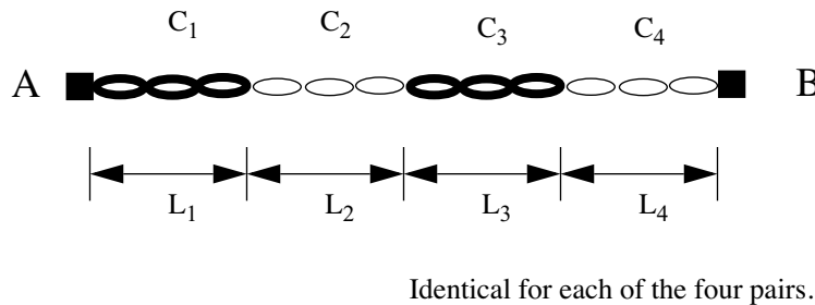
Figure 40-18—Test channel topology for each cable pair
