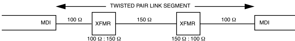
Figure D-1 — Link segment incorporating 150 \Omega cable section
