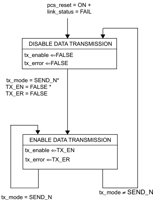
Figure 40–8—PCS Data Transmission Enabling state diagram
