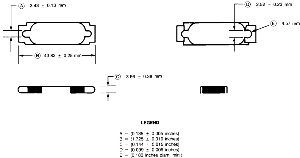
Figure 7-19—Connector slide latch
