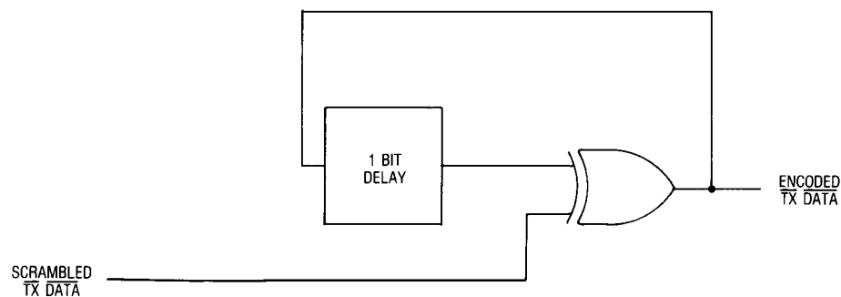
Figure 11–11—Differential encoder
