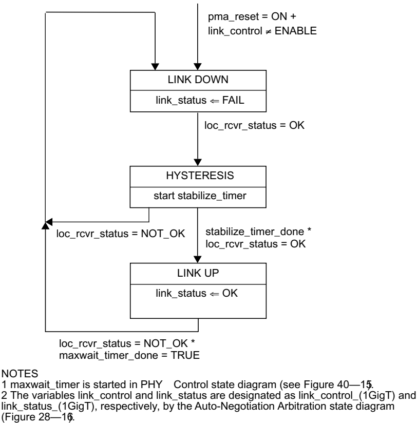
Figure 40–16—Link Monitor state diagram
