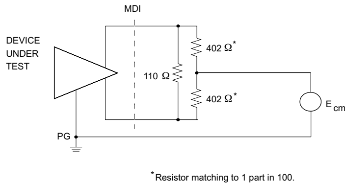
Figure 40-33—MDI fault tolerance test circuit
