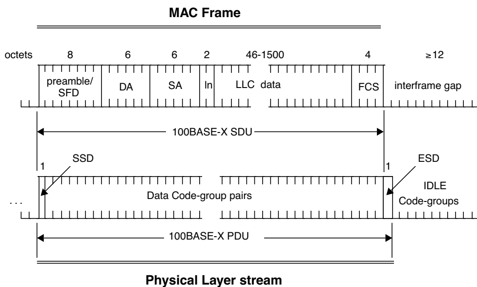
Figure 24–5—PCS encapsulation
