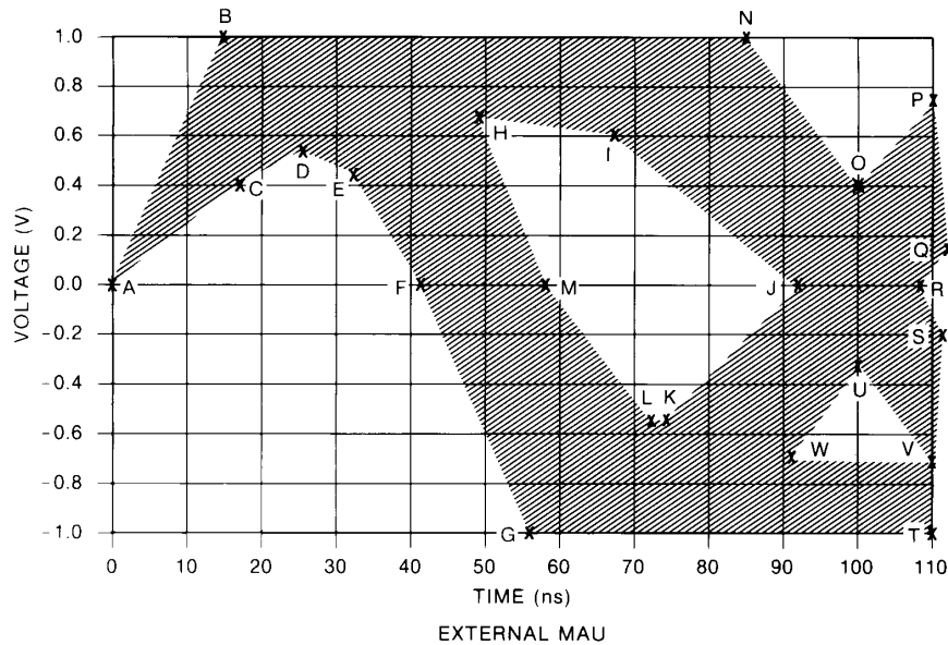
Figure 14-9—Voltage template
