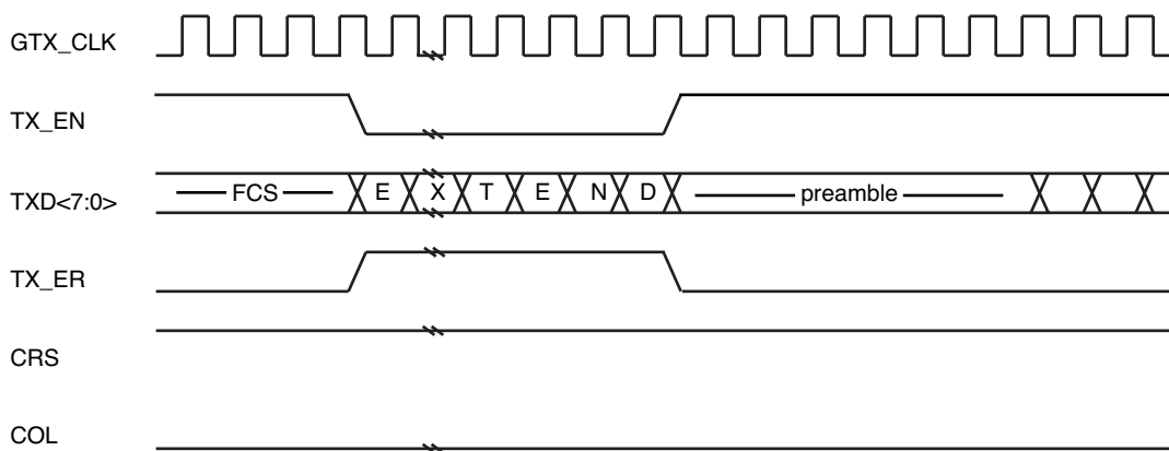
Figure 35-7—Burst transmission
