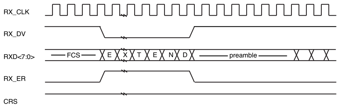
Figure 35-10—Burst reception
