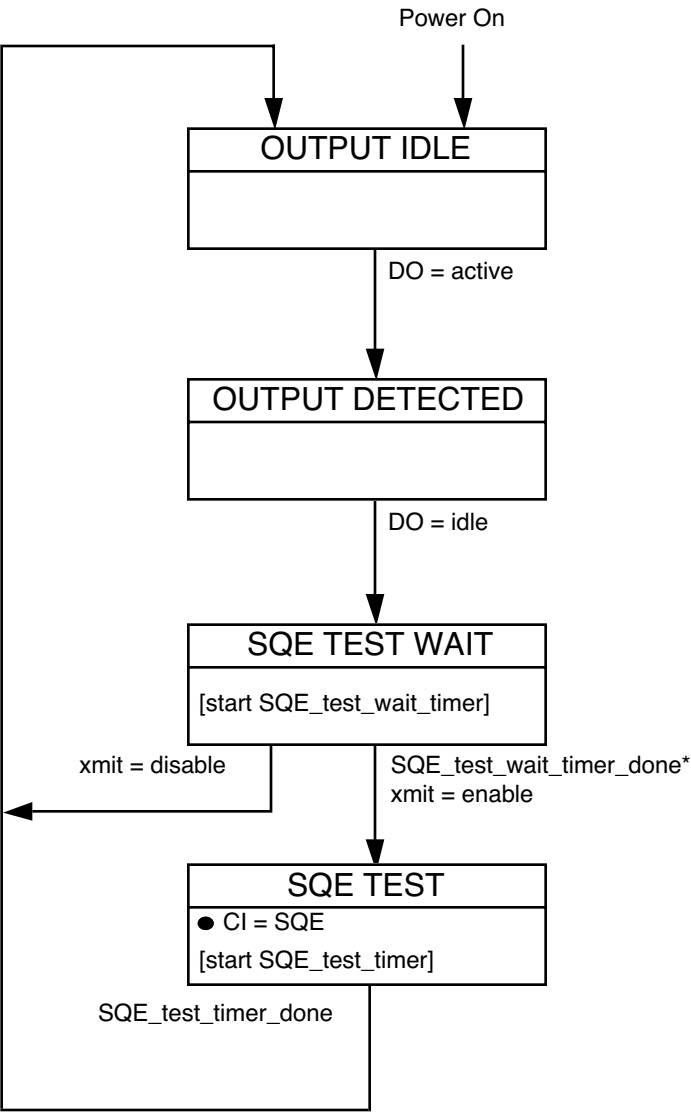
Figure 18–2— signal_quality_error Message Test function state diagram
