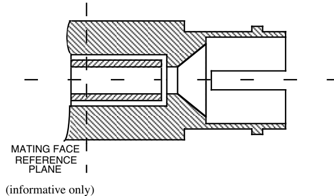
Figure 15-6—BFOC/2.5 connector plug
