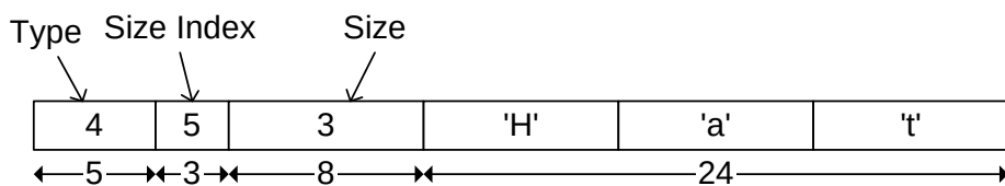
Figure 3.1: Data Element
