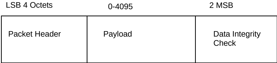
Figure 4.1: Packet Format
