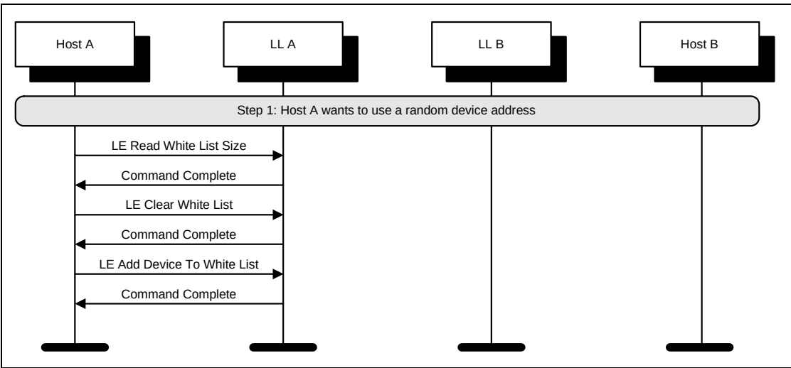
Figure 2.3: White Lists
