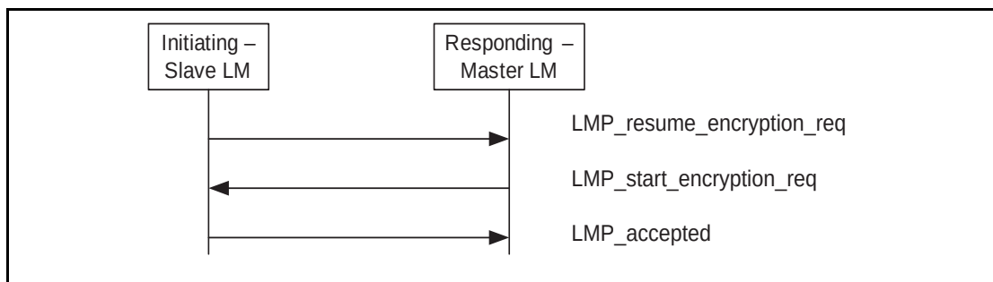
Sequence 43: Initiating Slave LM resumes encryption
