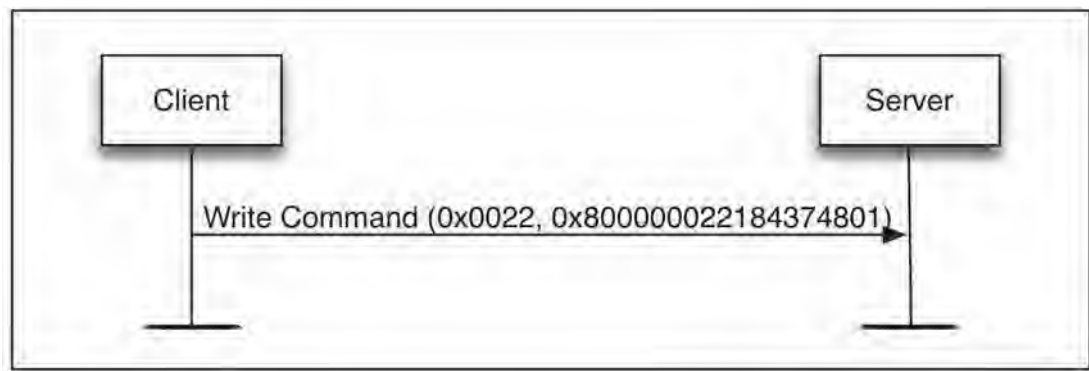
Figure 4.13: Signed Write Without Response example
