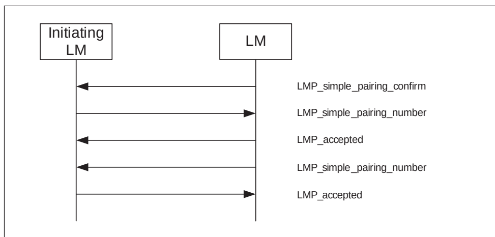
Sequence 49: Numeric Comparison Authentication: Commitment check success
