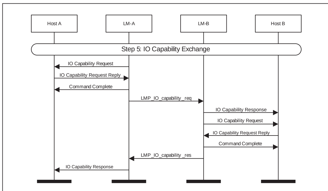
Figure 4.8: IO Capability Exchange
