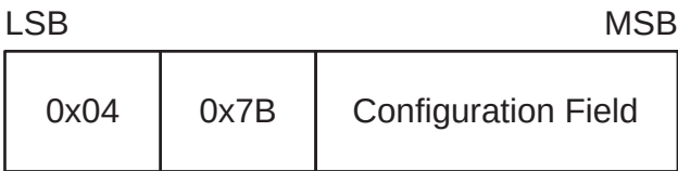
Figure 8.5: Configuration Response Message Format
