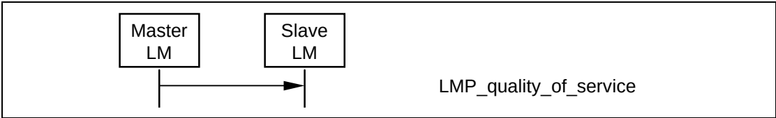
Sequence 13: Master notifies slave of quality of service.
