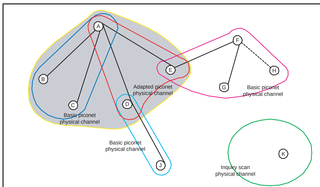
Figure 4.1: Example Bluetooth BR/EDR topology
