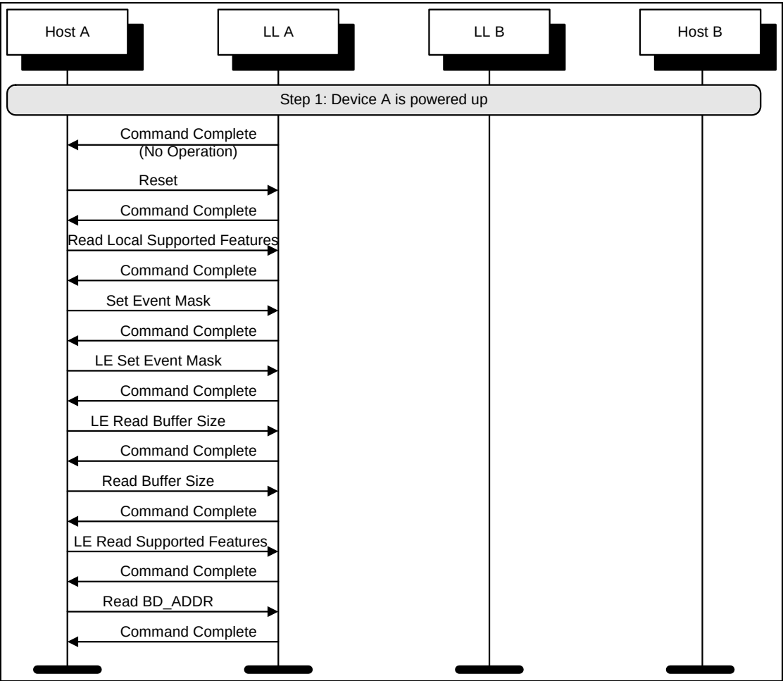
Figure 2.1: Initial Setup
