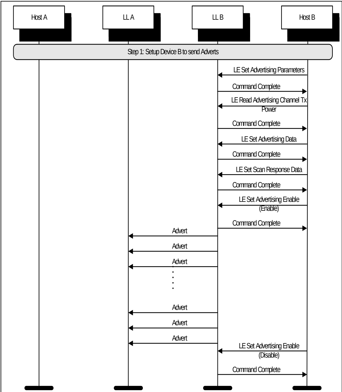
Figure 3.1: Undirected Advertising
