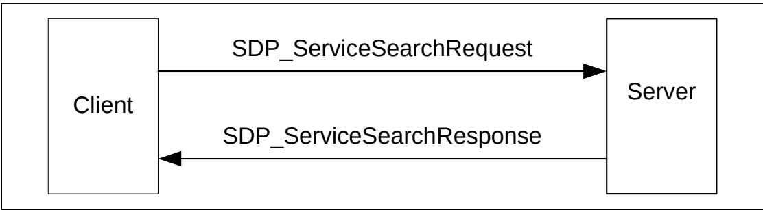
Figure 4.4: ServiceSearch Transaction
