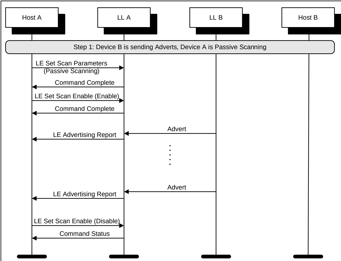
Figure 4.1: Passive Scanning
