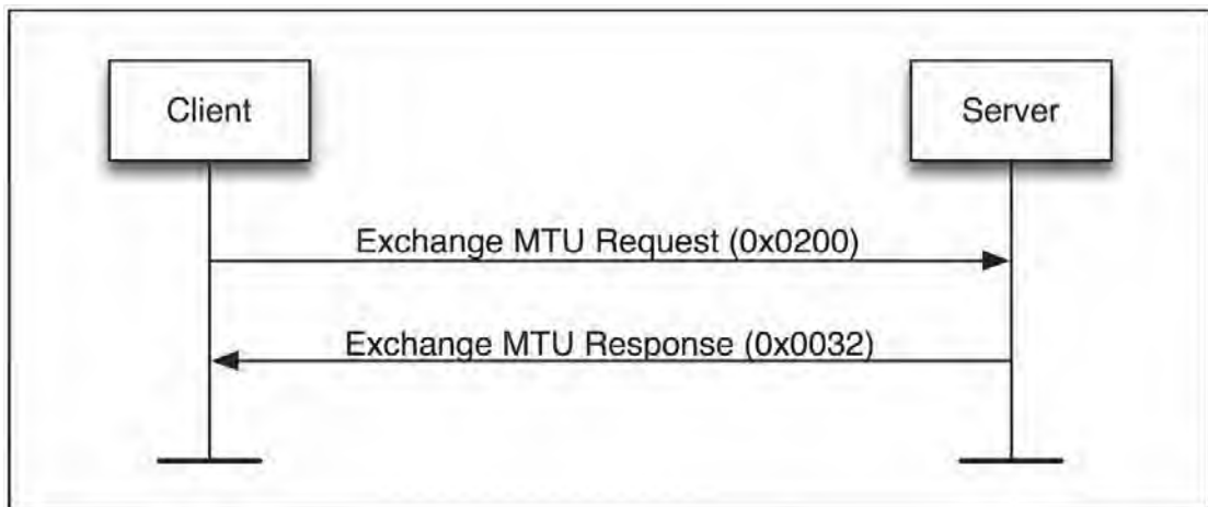
Figure 4.1: Exchange MTU
