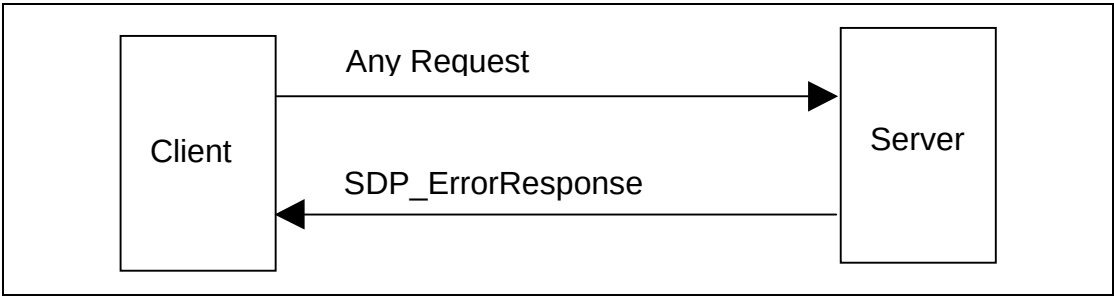
Figure 4.3: Error Handling
