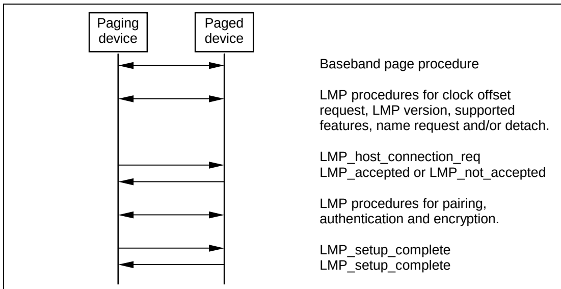
Figure 4.1: Connection establishment.
