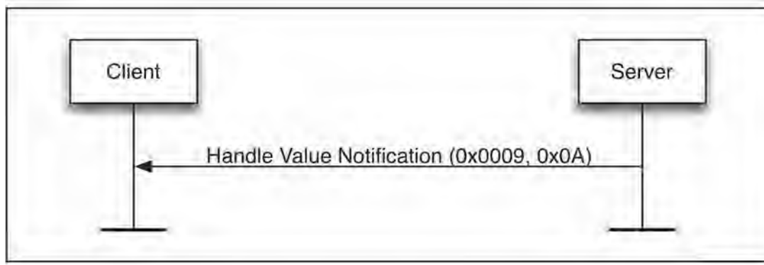
Figure 4.17: Notifications example
