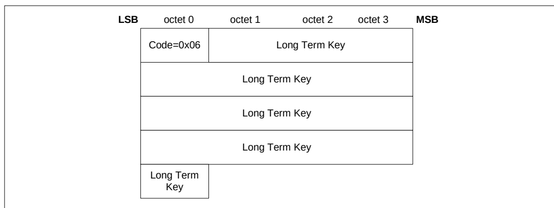
Figure 3.9: Encryption Information Packet
