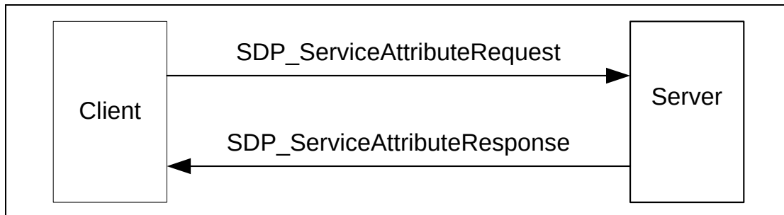
Figure 4.5: ServiceAttribute Transaction
