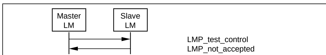
Sequence 102: Control of test mode rejected since slave is not in test mode.
