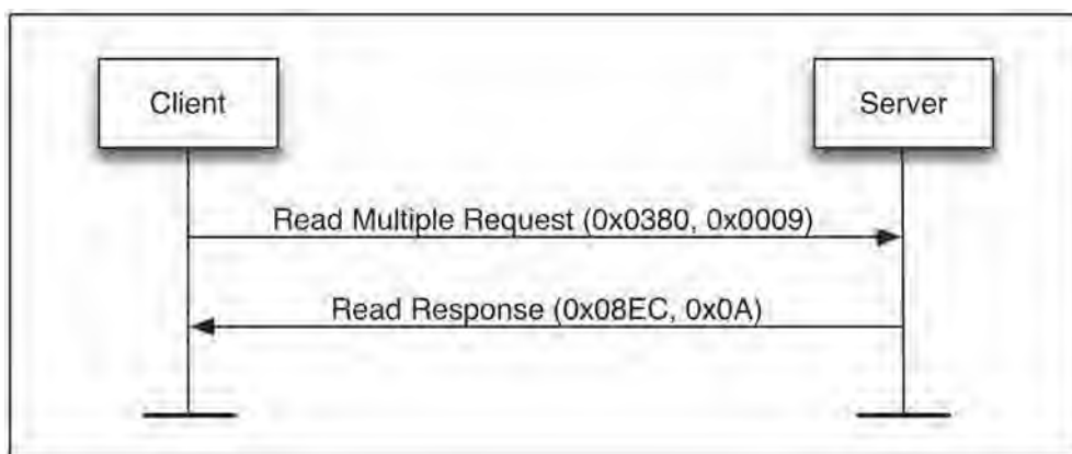
Figure 4.11: Read Multiple Characteristic Values example
