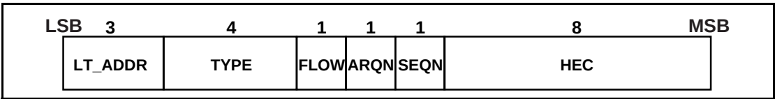
Figure 6.8: Header format.
