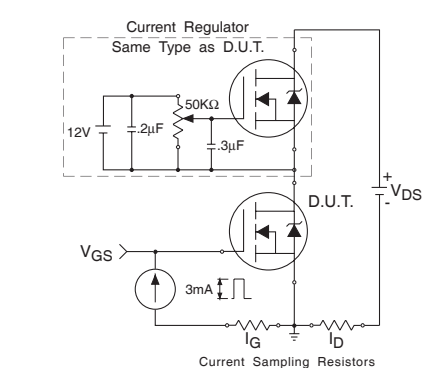
Fig 24a. Gate Charge Test Circuit
