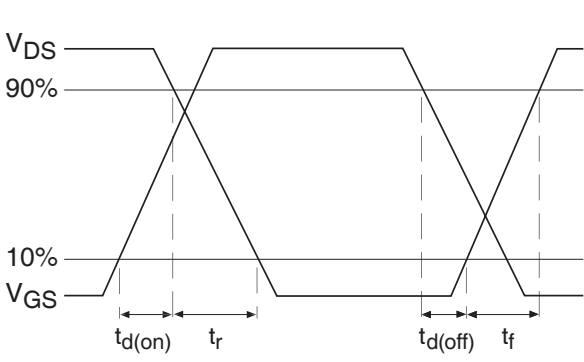
Fig 23b. Switching Time Waveforms
