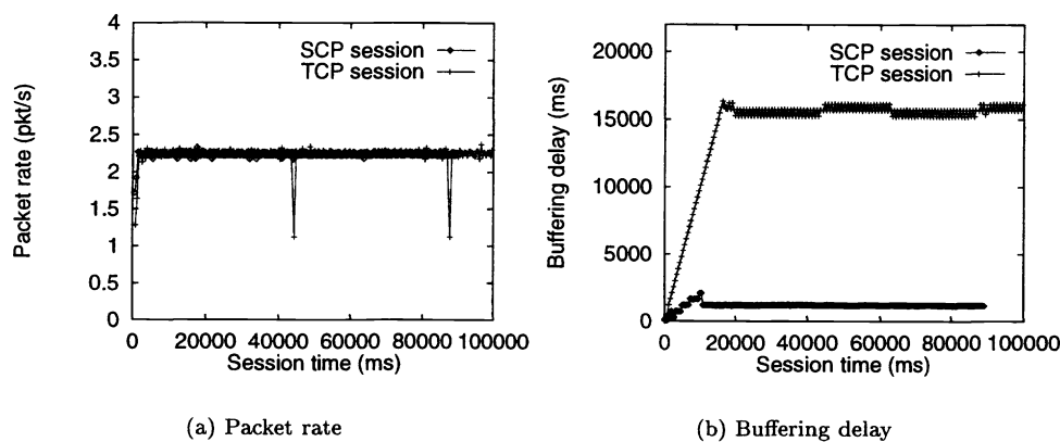
Figure 3. Performance of single SCP and TCP sessions from lemond to anquetil over PPP
