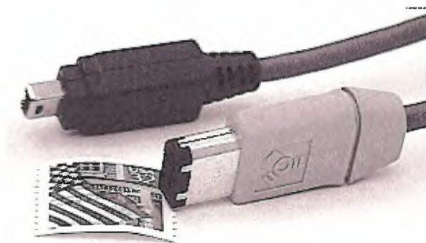
Fig 1: The 1394 connectors
