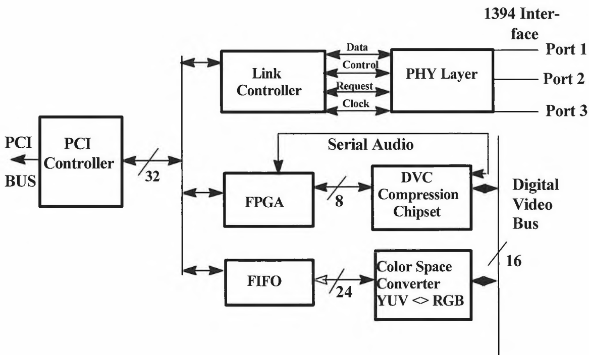
Fig4: 1394/DV adapter-codec block diagram
