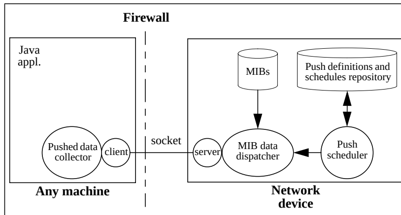
Fig. 7. Push model: distribution via sockets
