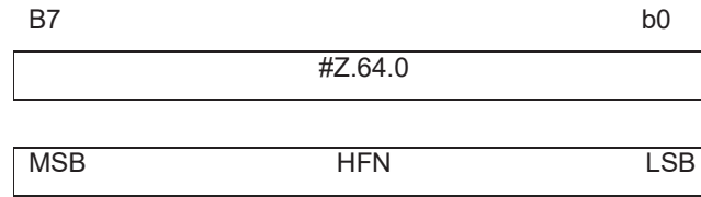
Figure 17: HFN mapping
