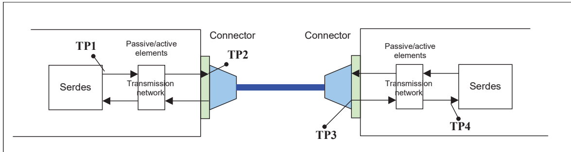
Figure 35: Reference test points
