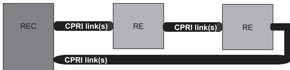
Figure 5C: Ring topology
