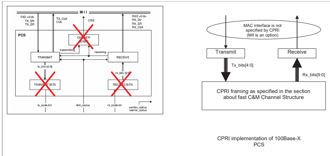
Figure 28: CPRI implementation of 100BASE-X PCS
