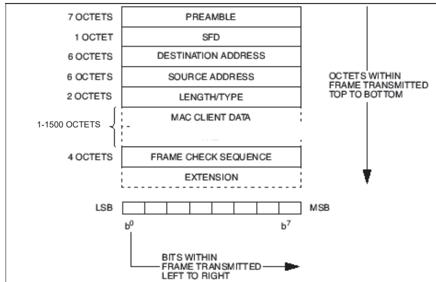
Figure 27: Layer 2 Framing
